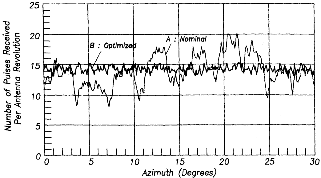
FIGURE 10. COMPARISON OF AZIMUTHAL COVERAGE OF AGILE FREQUENCY SELECTIONS WITH AND WITHOUT OPTIMIZATION.
