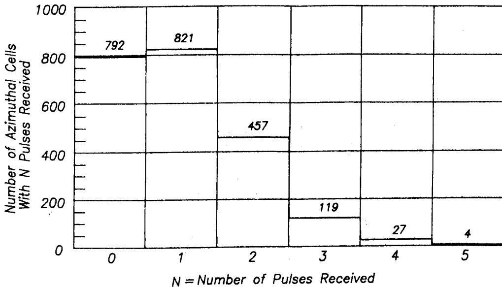
FIGURE 7. DISTRIBUTION OF MULTIPLE PULSE CELLS.
