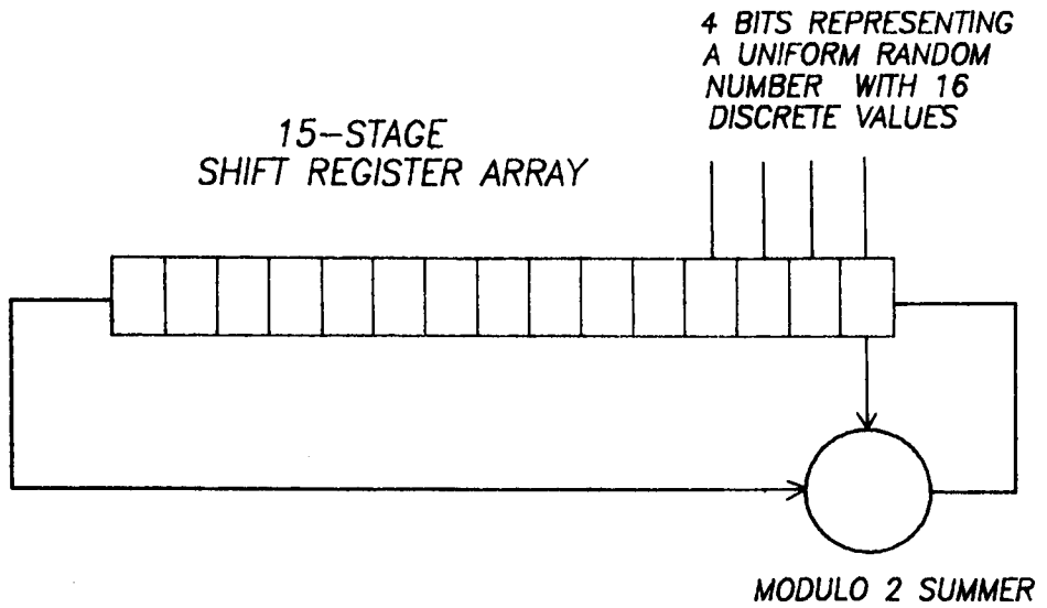
FIGURE 2. A 15-STAGE PSEUDO-NOISE GENERATOR.
