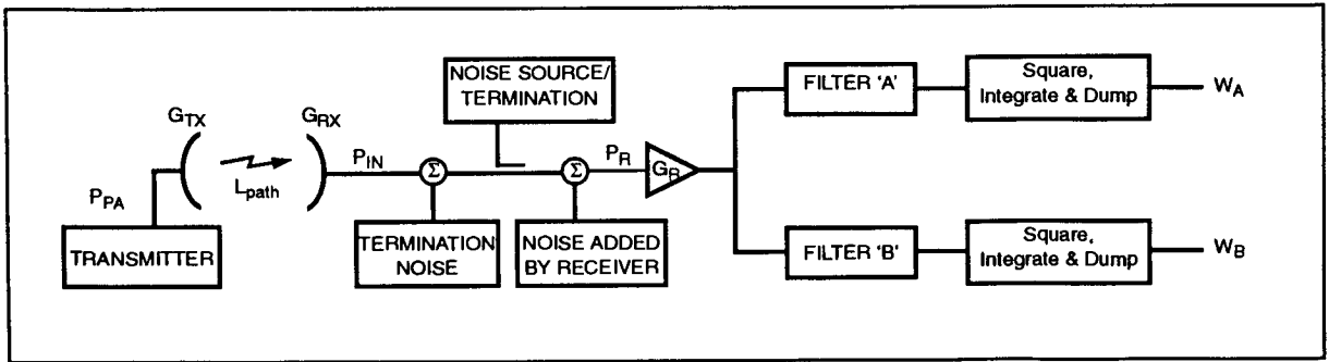
FIGURE 2. Simplified block diagram of troposcatter measurement system
