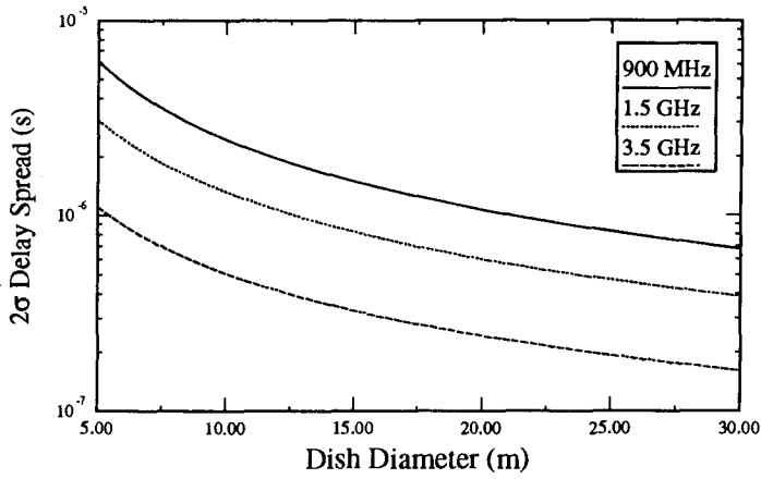
FIGURE 10. Estimate of multipath delay spread using Sunde model for various carrier frequency and parabolic dishes diameter
