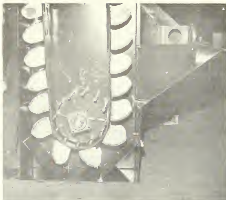
Figure 2.3.13 Elevator boot and inspection section. Courtesy: Clay Equipment Corp.
