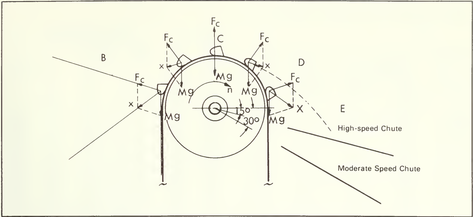
Figure 2.3.11 Resultant forces on material in bucket at elevator head pulley
