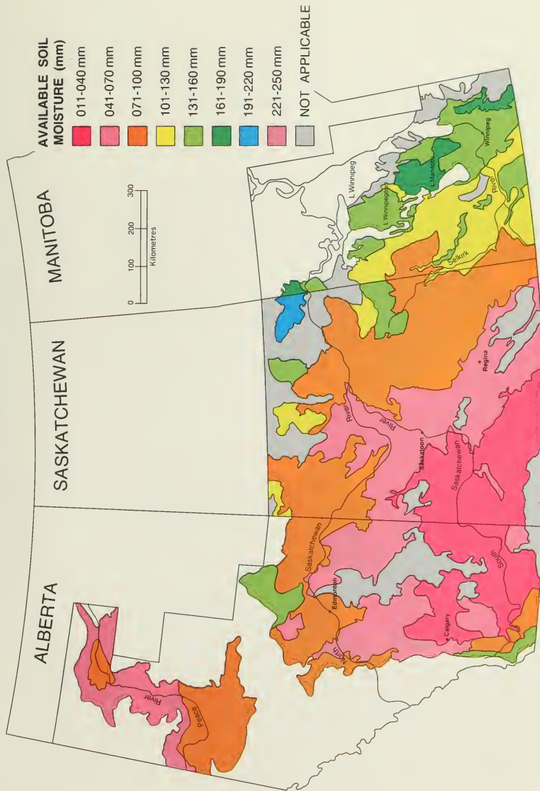
Figure 5. Available soil moisture (mm) at seeding for 250 mm soil AWC, 10% probability, continuous wheat rotation.
