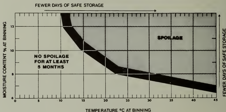
CANOLA STORAGE TIME CHART*
