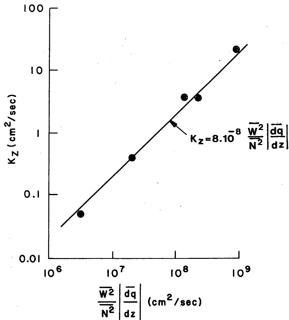
FIGURE 6. VERTICAL EDDY DIFFUSIVITY vs WIND STRESS, STABILITY PARAMETER AND CURRENT SHEAR
