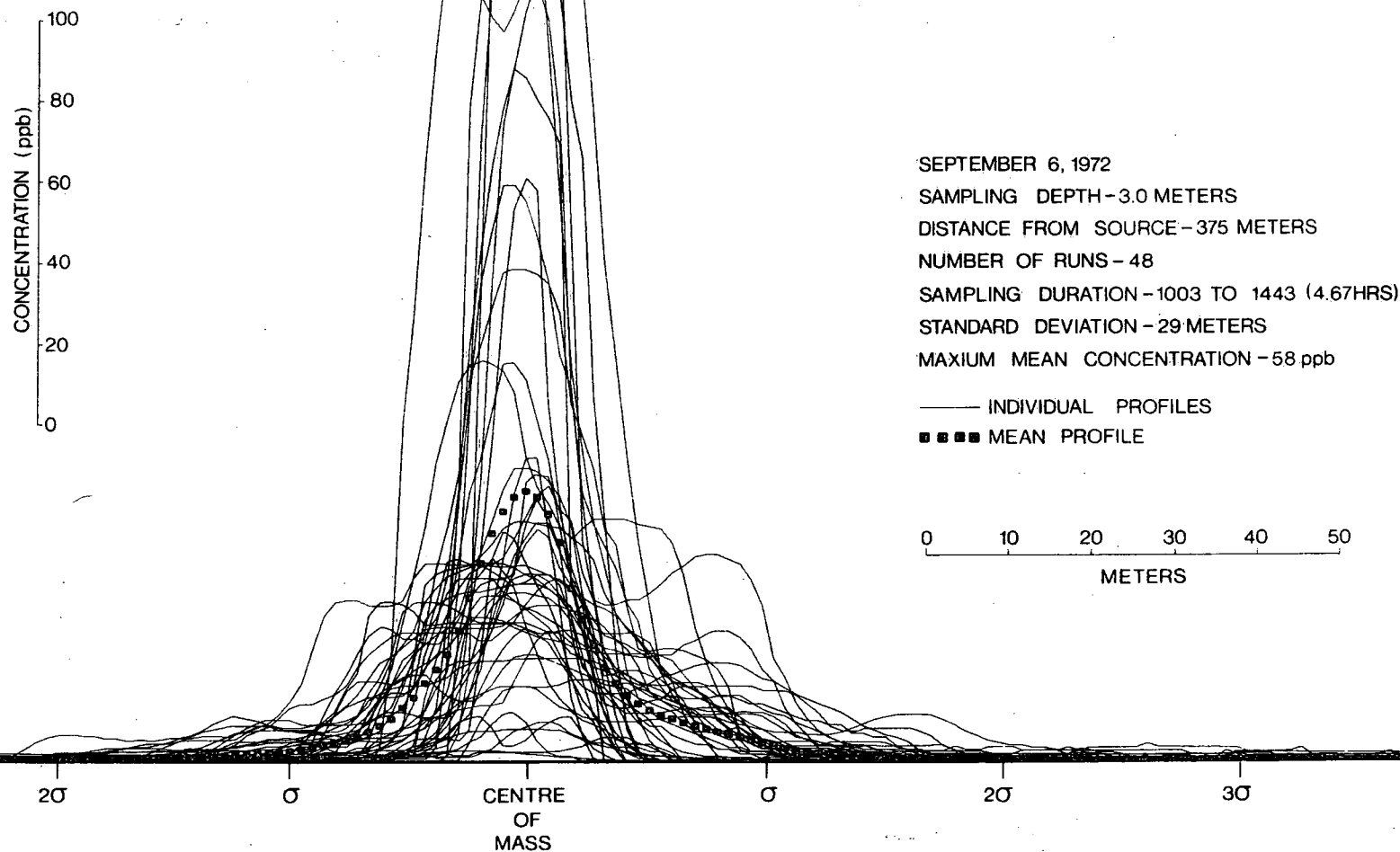
CROSSPLUME CONCENTRATION DISTRIBUTION -RELATIVE
