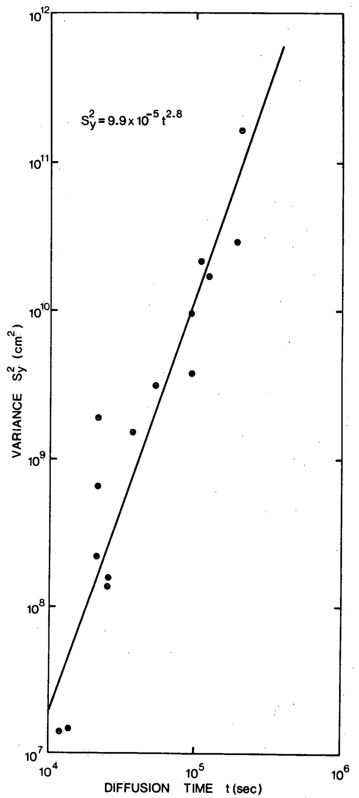
FIGURE 2. HORIZONTAL VARIANCE vs DIFFUSION TIME SCALE
