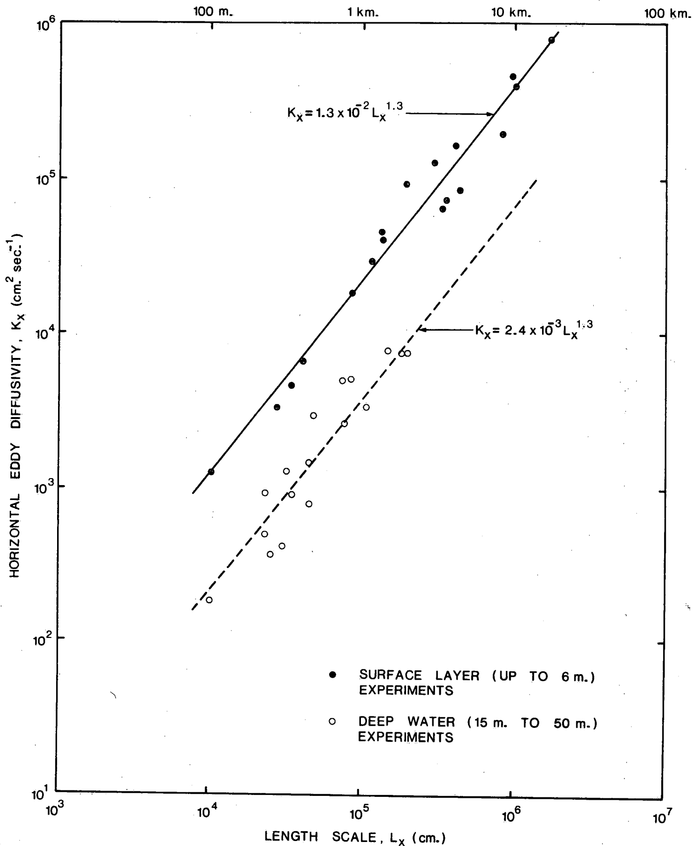
FIGURE 3. HORIZONTAL (LONGITUDINAL) EDDY DIFFUSIVITY vs DIFFUSION LENGTH SCALE
