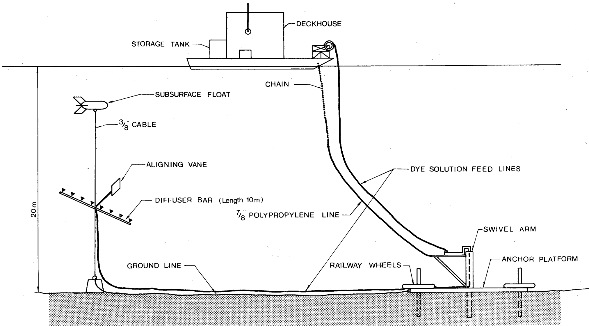
FIGURE 2. CONTINUOUS DYE RELEASE SYSTEM
