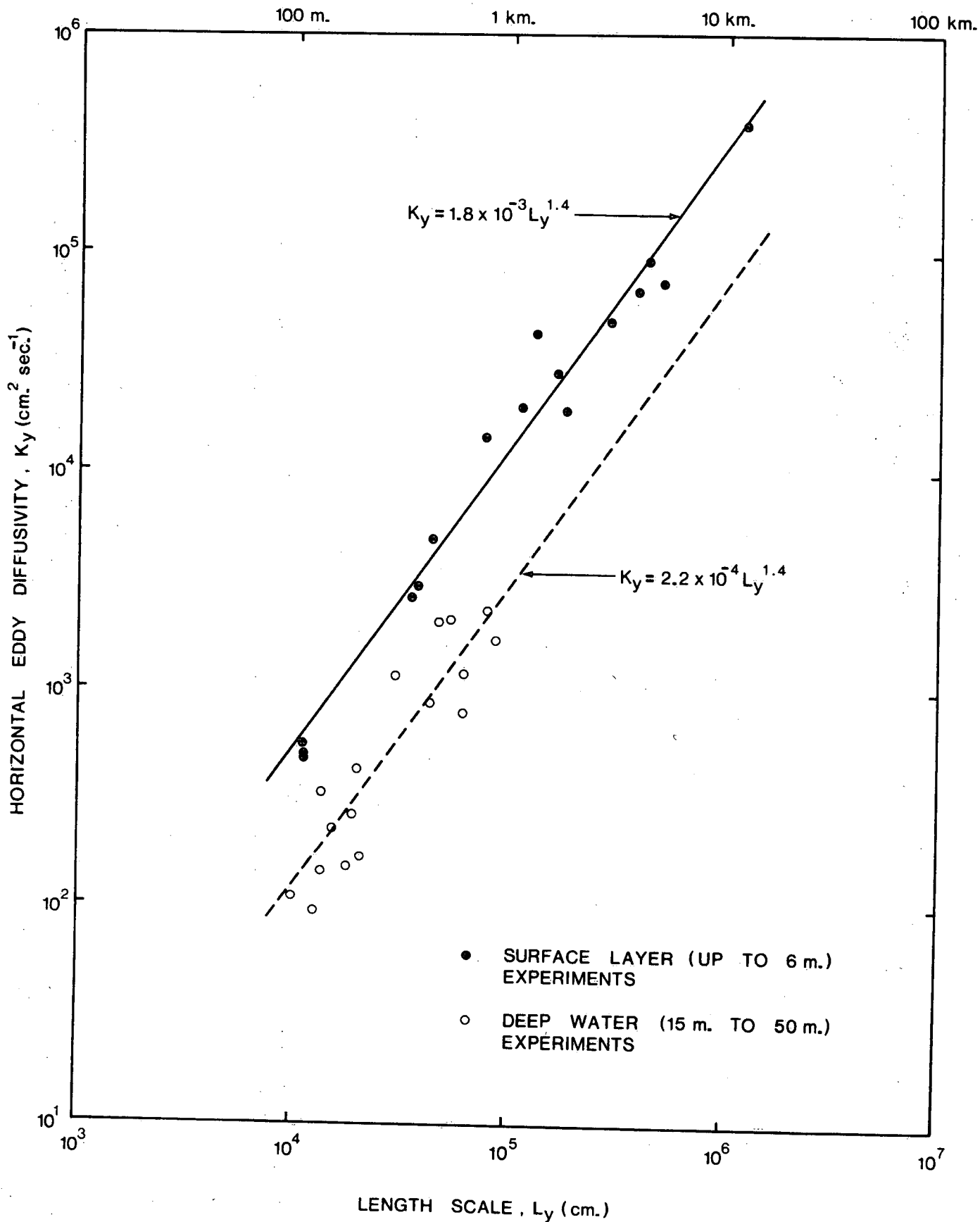
FIGURE 4. HORIZONTAL (LATERAL) EDDY DIFFUSIVITY vs DIFFUSION LENGTH SCALE
