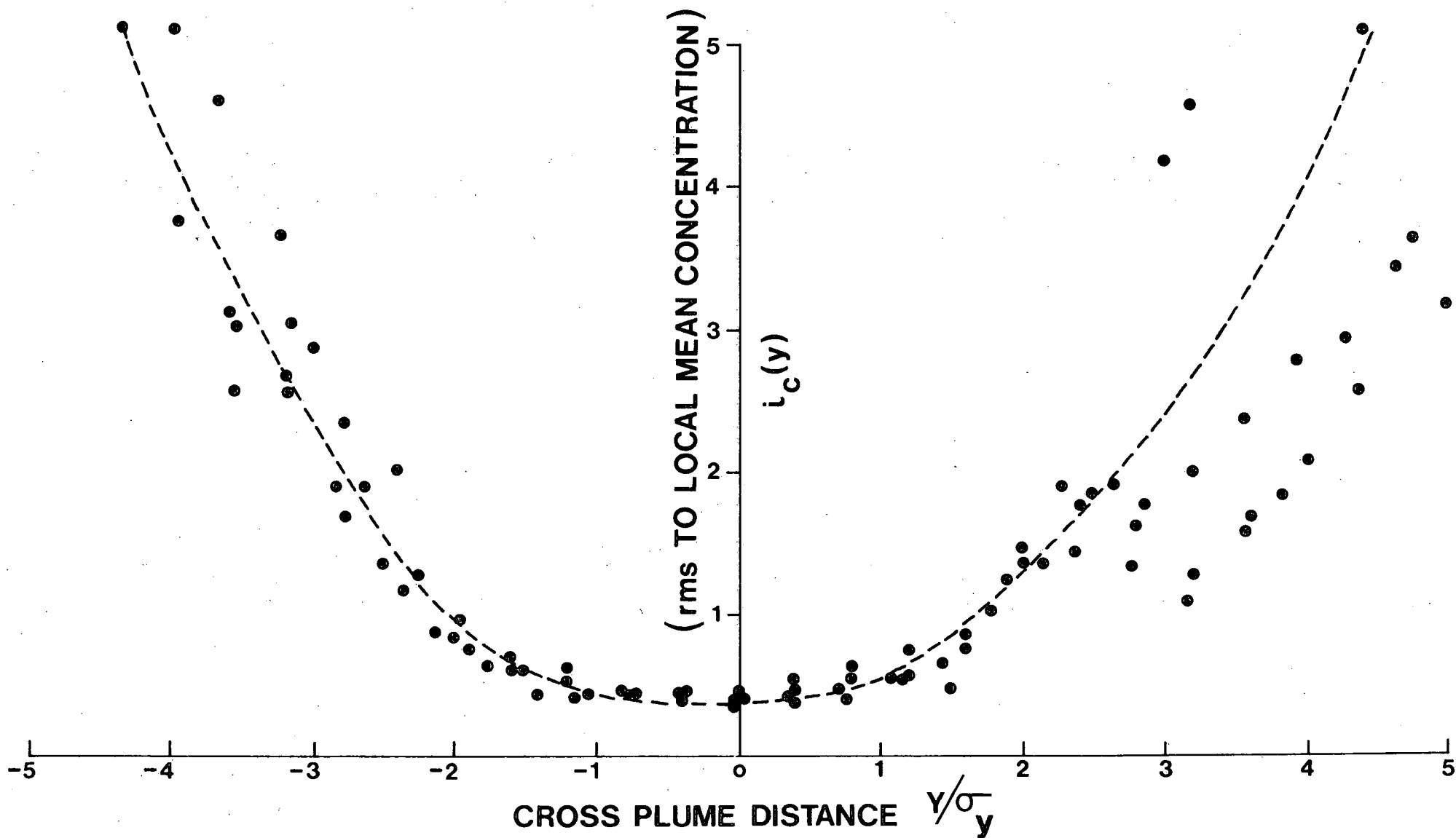
FIGURE 5. CONC. FLUCTUATION PROFILE
