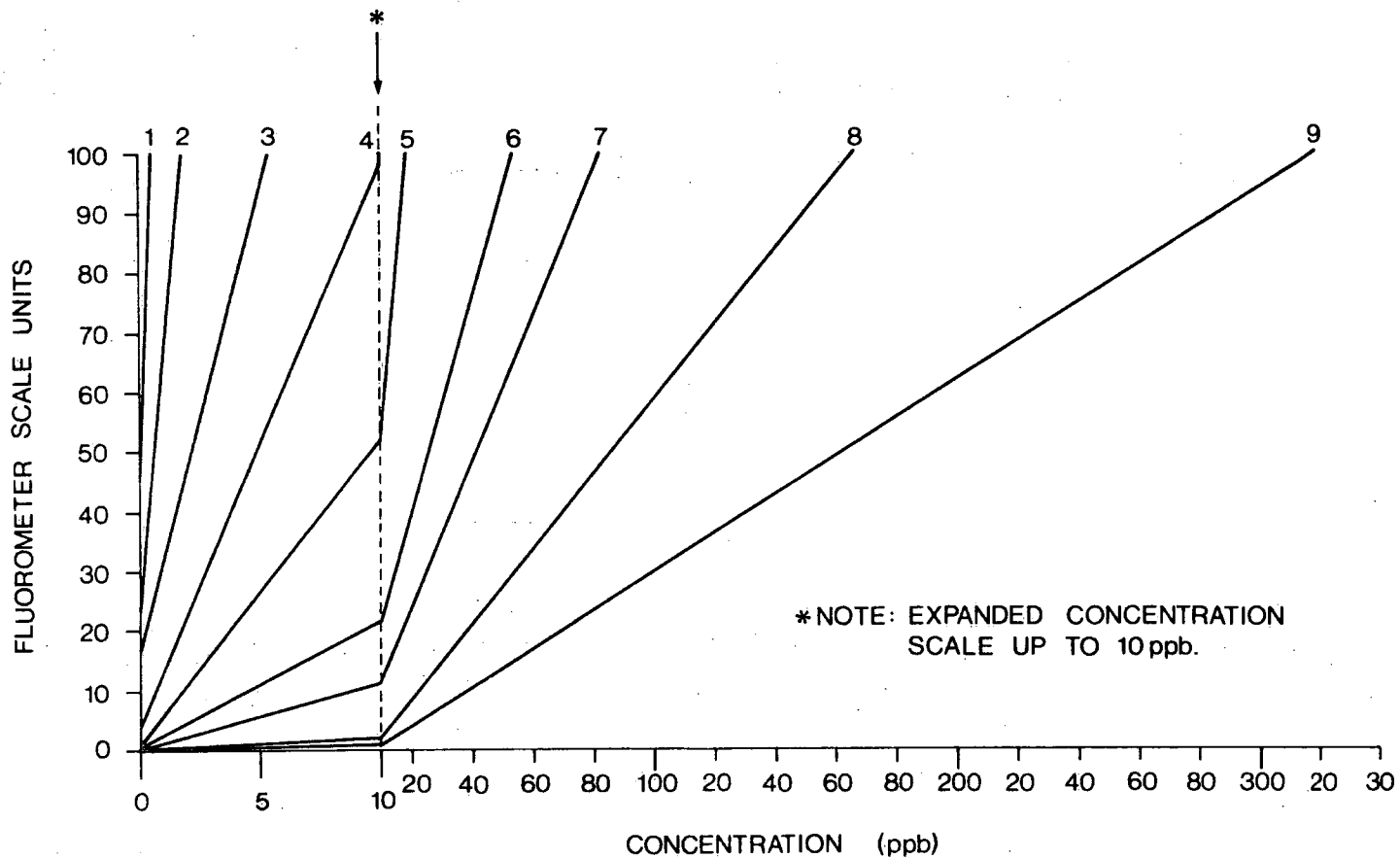
FIGURE 4. TYPICAL CALIBRATION CURVES FOR TURNER MODEL 111 FLUOROMETER
