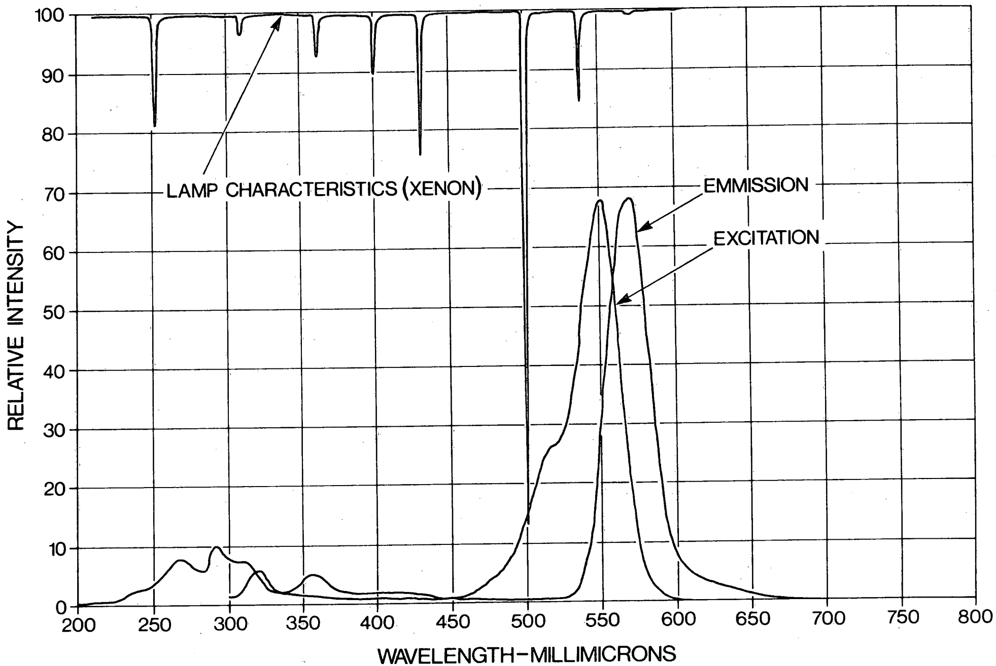
FIGURE 3. EXCITATION AND EMISSION SPECTRA FOR RHODAMINE B
