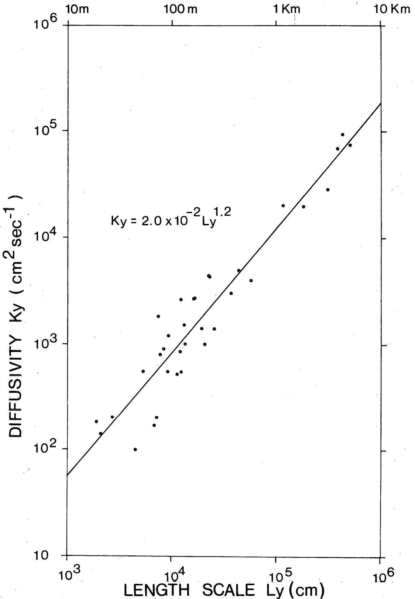
FIGURE 7. HORIZONTAL EDDY DIFFUSIVITY vs LENGTH SCALE OF DIFFUSION
