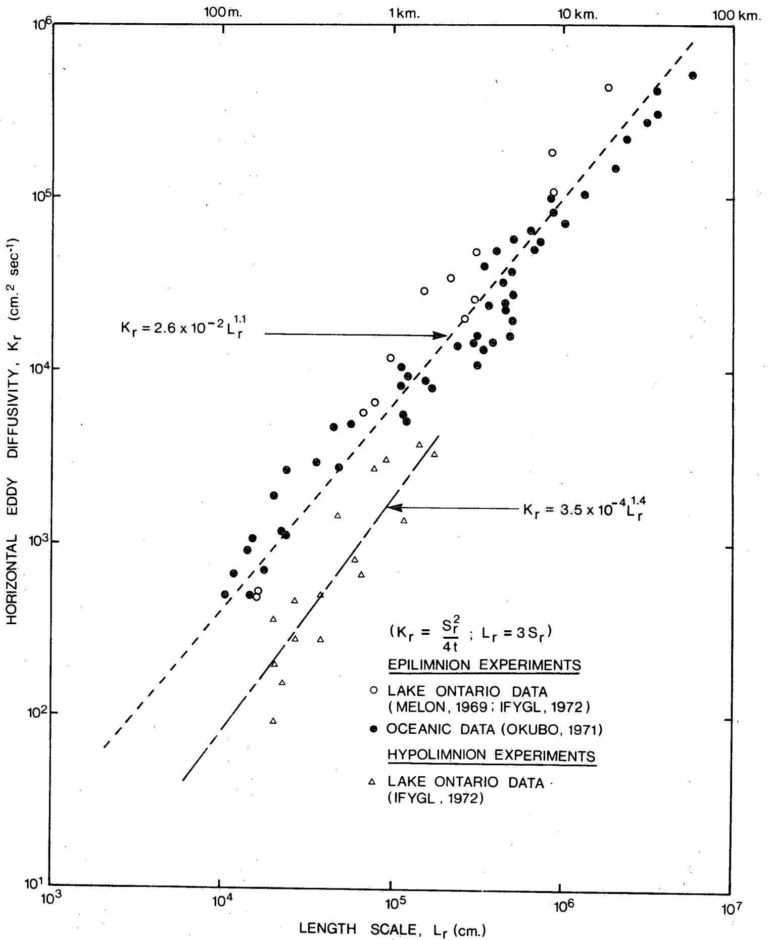
FIGURE 5. COMPARISON OF OCEANIC DIFFUSION DATA WITH GREAT LAKES DIFFUSION DATA
