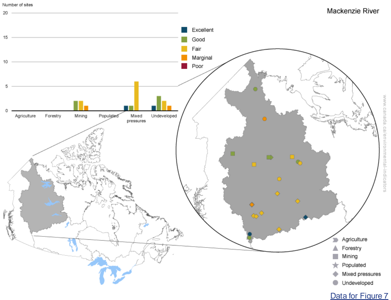
Figure 7. Water quality by land use category, Mackenzie River region, 2017 to 2019 period
