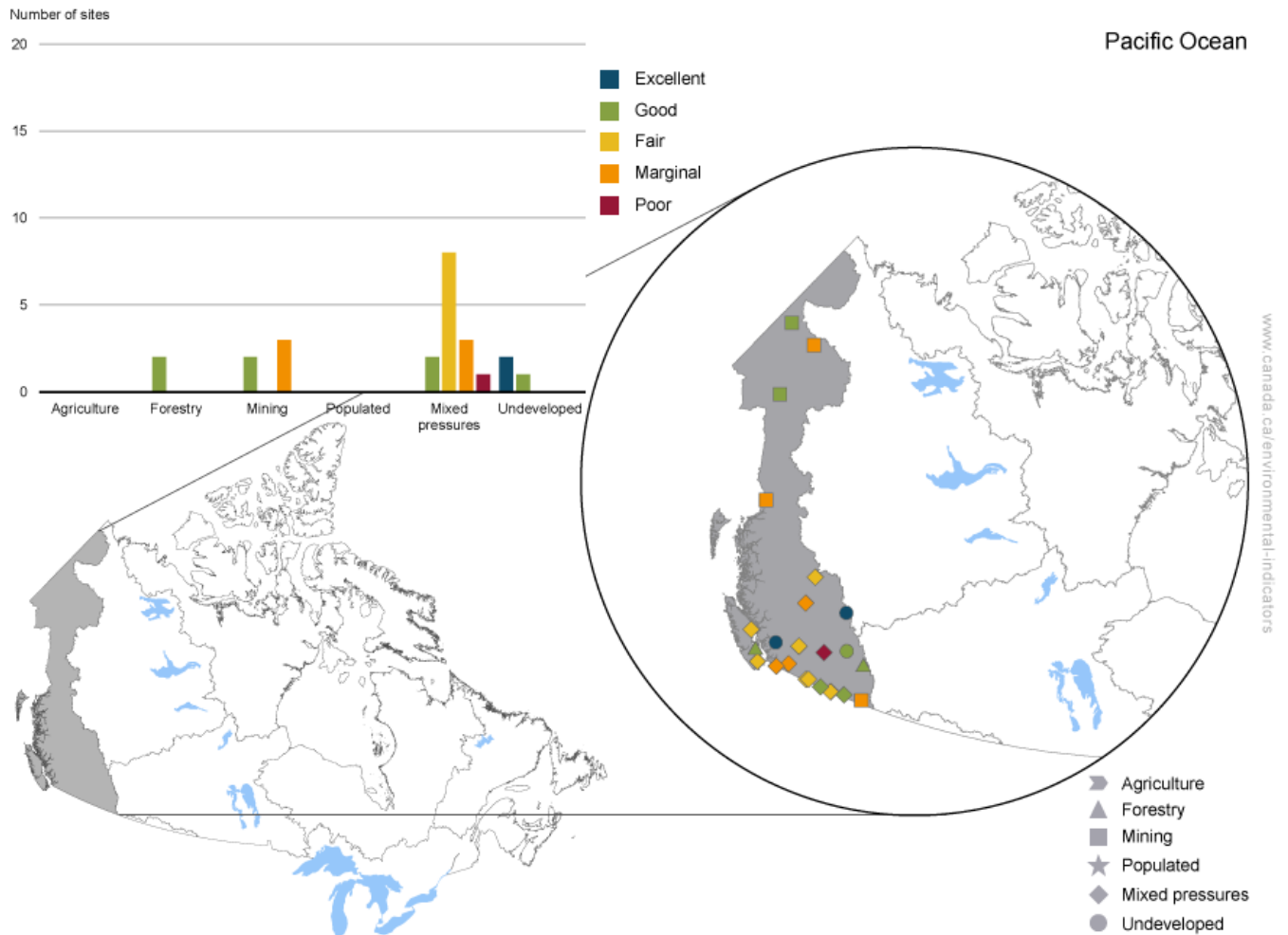
Figure 8. Water quality by land use category, Pacific Ocean region, 2017 to 2019 period
