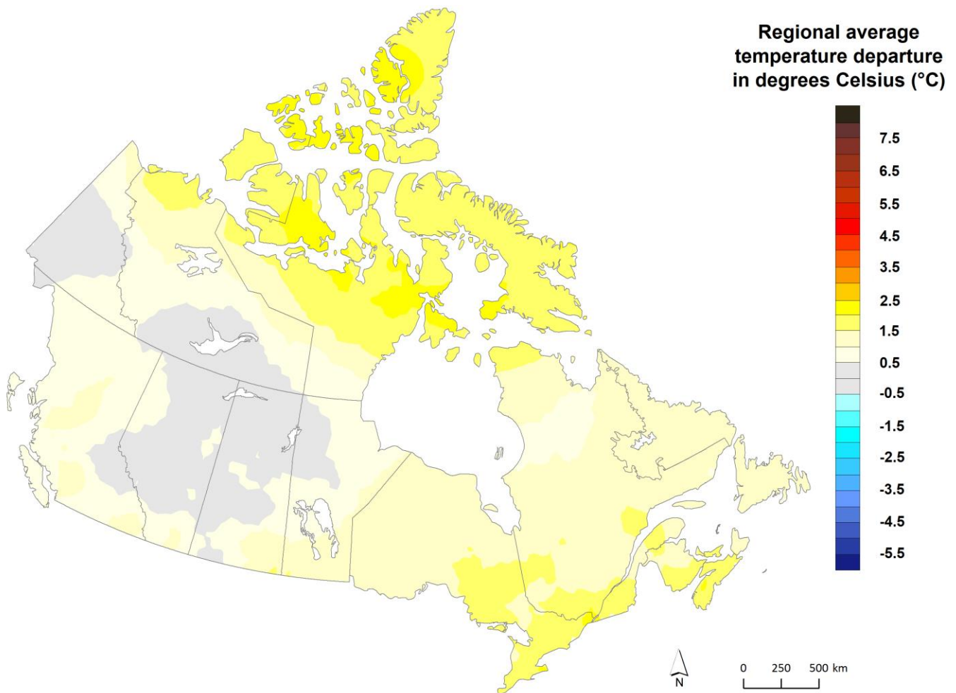
Figure 3. Regional average temperature departures from the 1961 to 1990 reference value, Canada, 2020
