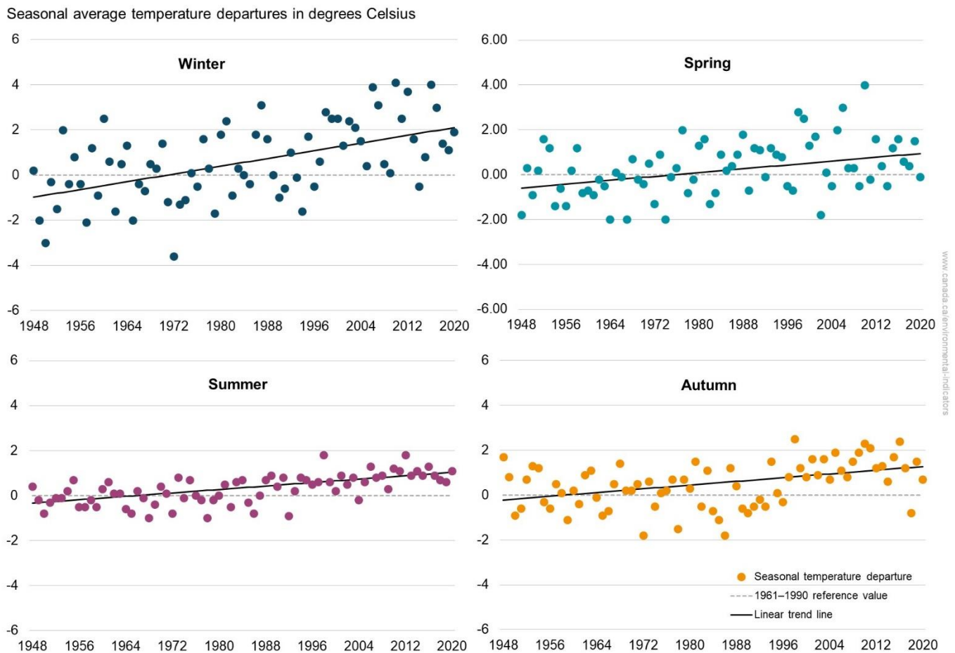
Figure 2. Seasonal average temperature departures compared with the 1961 to 1990 reference value, Canada, 1948 to 2020
