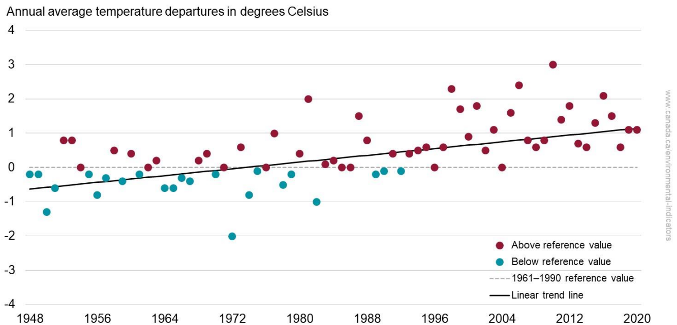
Figure 1. Annual average temperature departures from the 1961 to 1990 reference value, Canada, 1948 to 2020
