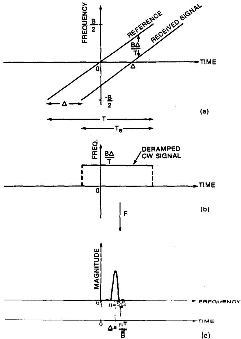
Fig. 31 - Conventional deramping technique for a point target.
