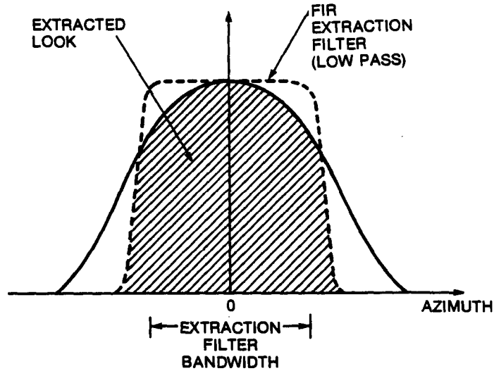
Fig. 26 - Look extraction using a low pass filter.
