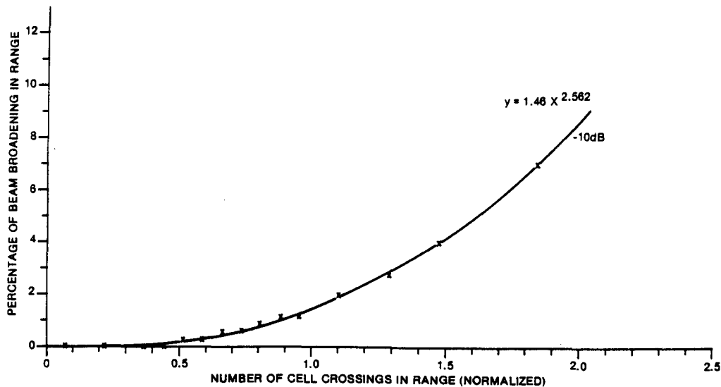
Fig. 10 - Empirical range beam broadening.
