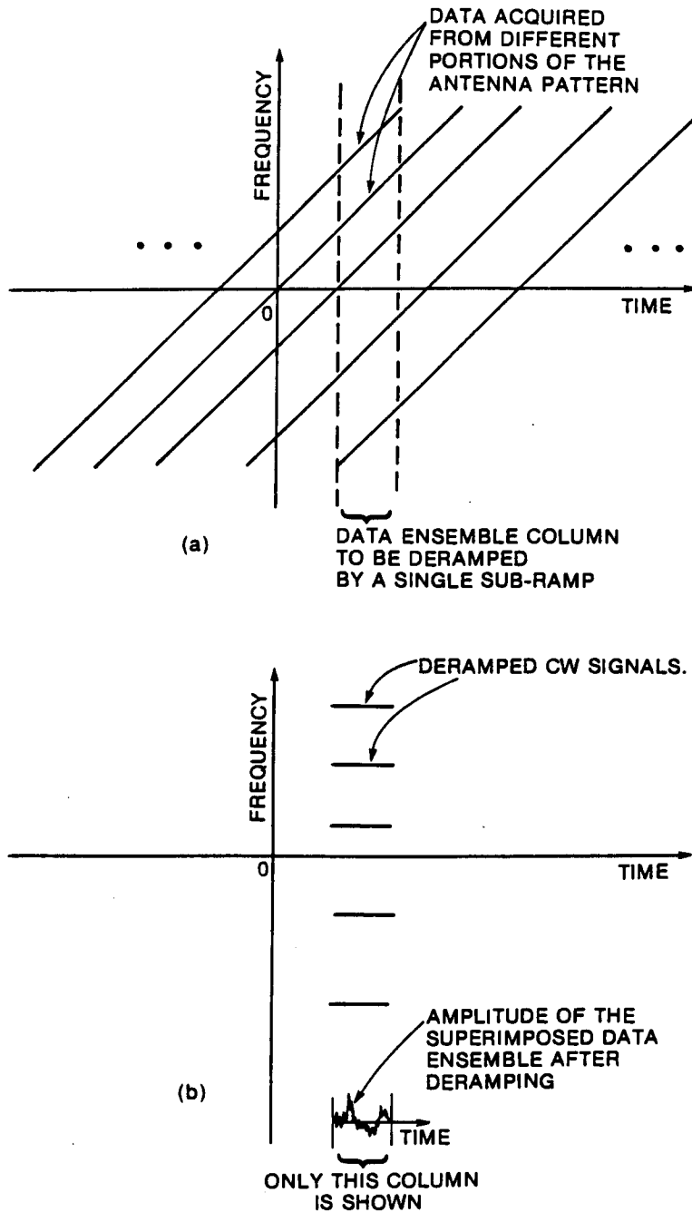
Fig. 41 - Deramping of multiple targets.
