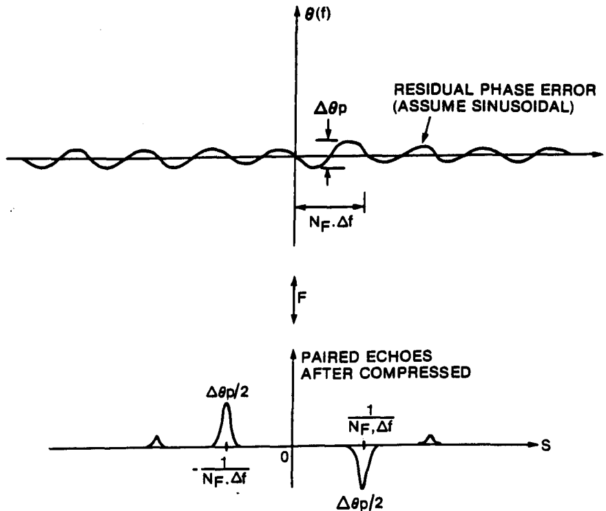
Fig. 30 - Residual phase error and paired echoes.
