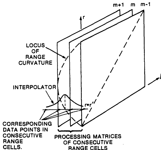
Fig. 52 - Range curvature compensation in step transform.
