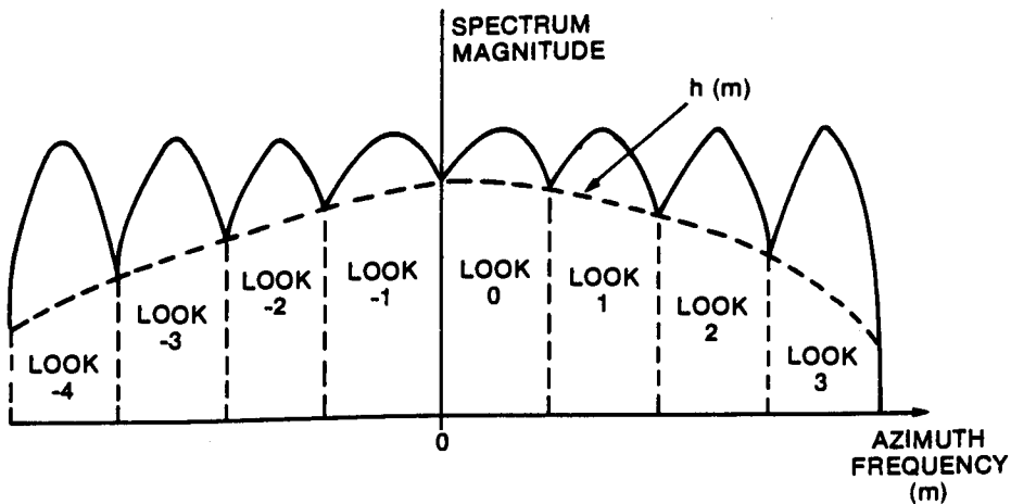
Fig. 27 - A typical coherently summed spectrum. The dotted line connecting all the minima is described by Eq. 68.
