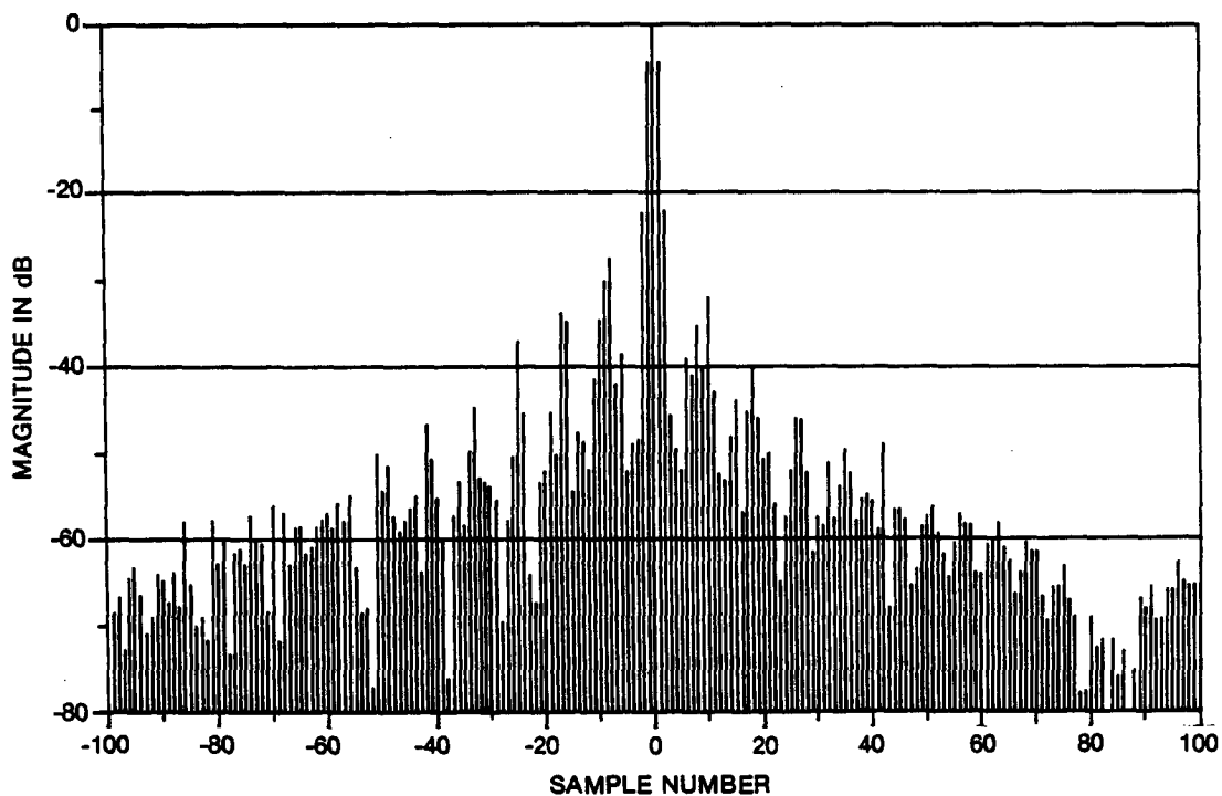
Fig. 23 - Compressed pulse with piecewise range curvature compensation (squint \eta_p = 15^\circ ).
