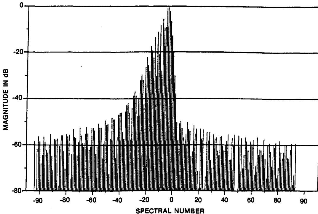
Fig. 17 - Compressed pulse with cubic phase uncompensated.
