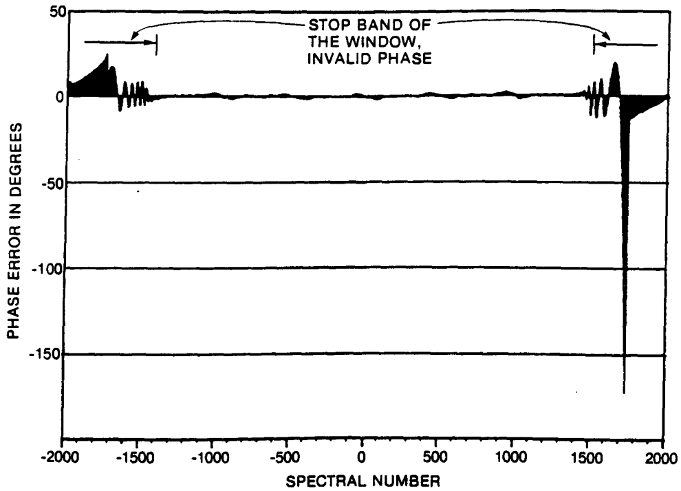
Fig. 21 - Residual Phase error (squint angle \eta_F = 30^\circ ).
