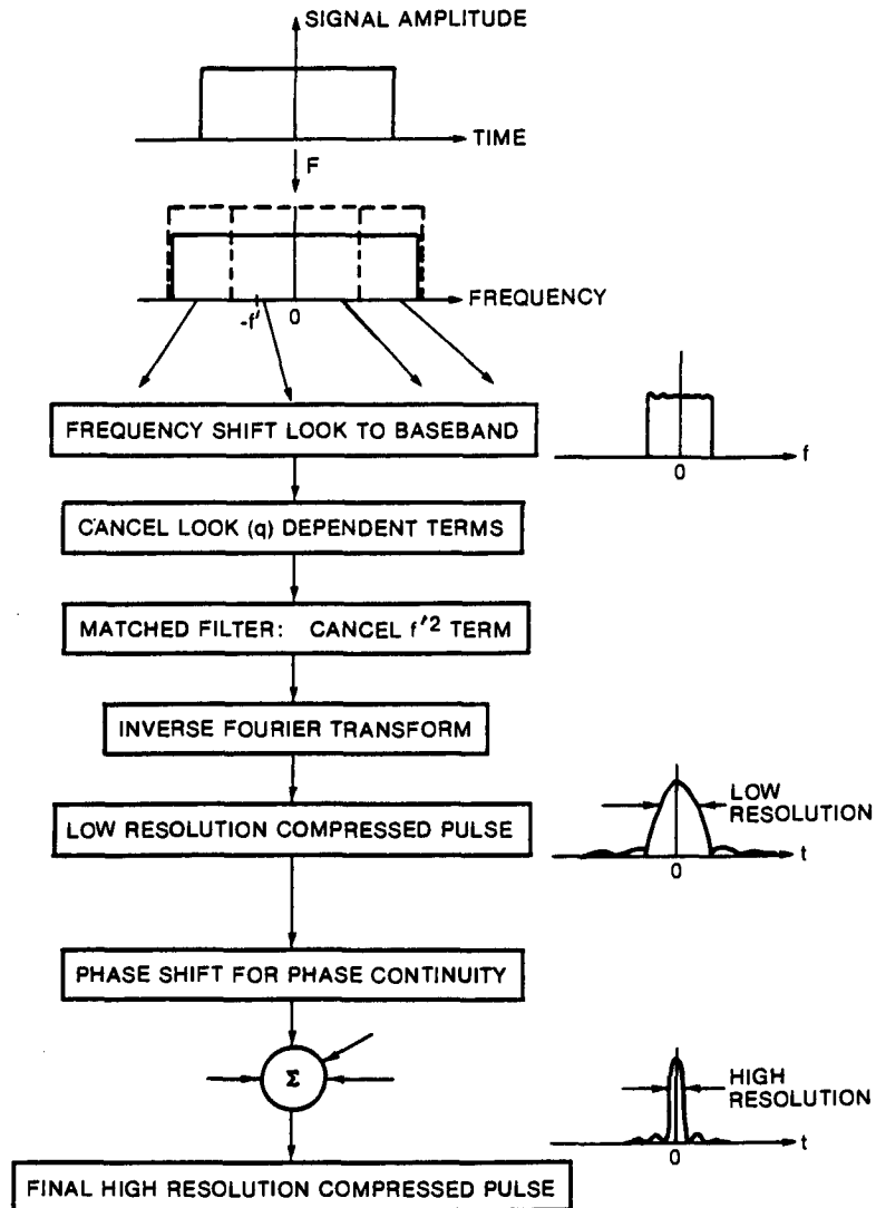
Fig. 2 - Coherent sub-aperture processing procedure for an ideal linear FM signal.
