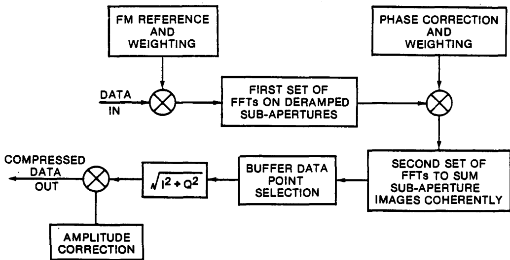
Fig. 44 - Step transform processing procedure [6].
