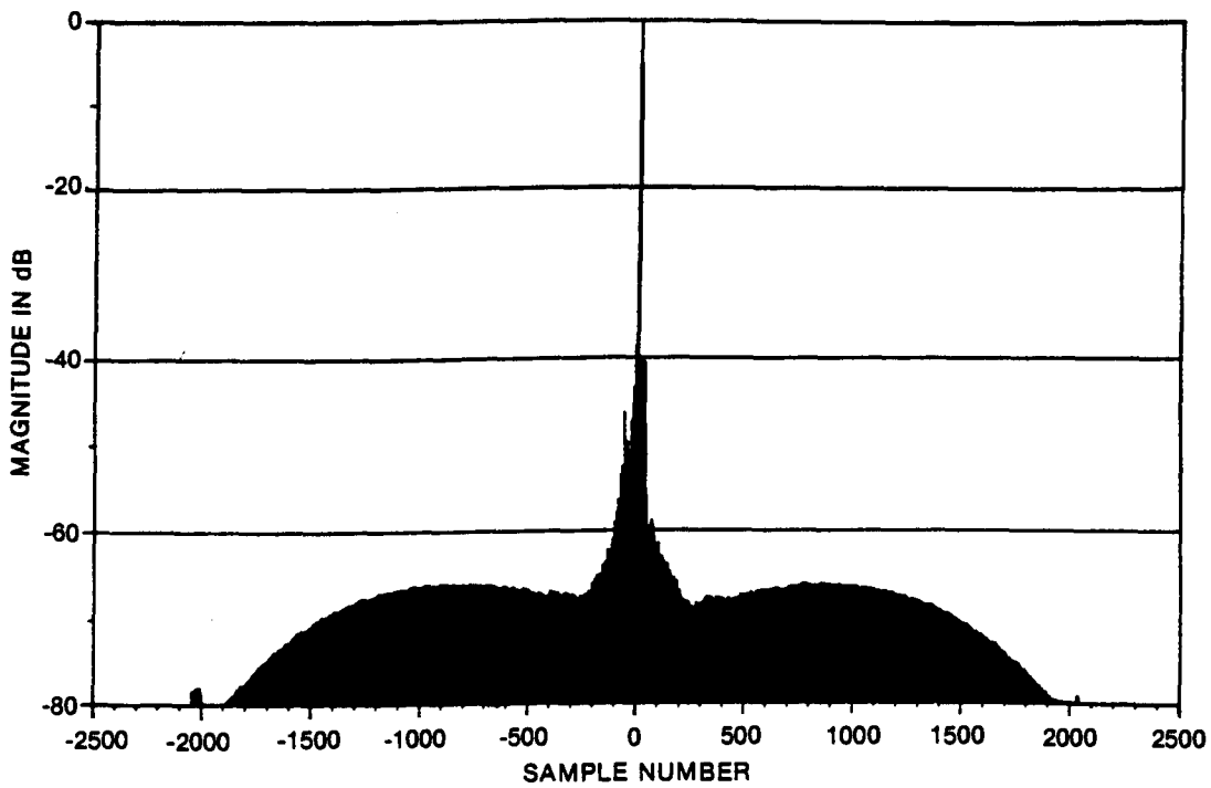
Figure 16 - Compressed pulse with continuous range curvature compensation, (a) overall,
