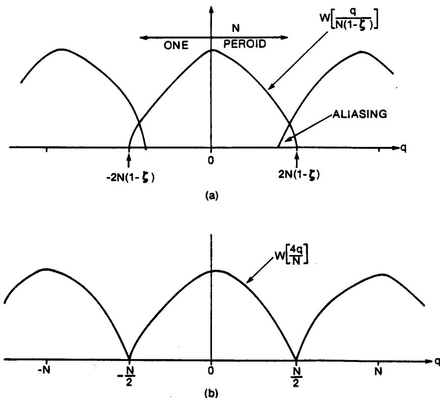
Fig. 47 - Aliasing mechanism due to the envelop function of the Hamming window, (a) with aliasing for \xi < 0.75 , (b) minimum condition with no aliasing, \xi = 0.75 .
