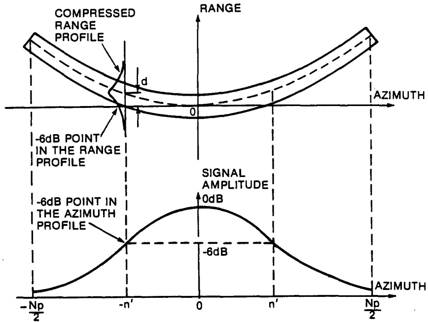
Fig. 8 - Range (compressed) - azimuth (uncompressed) coupling.
