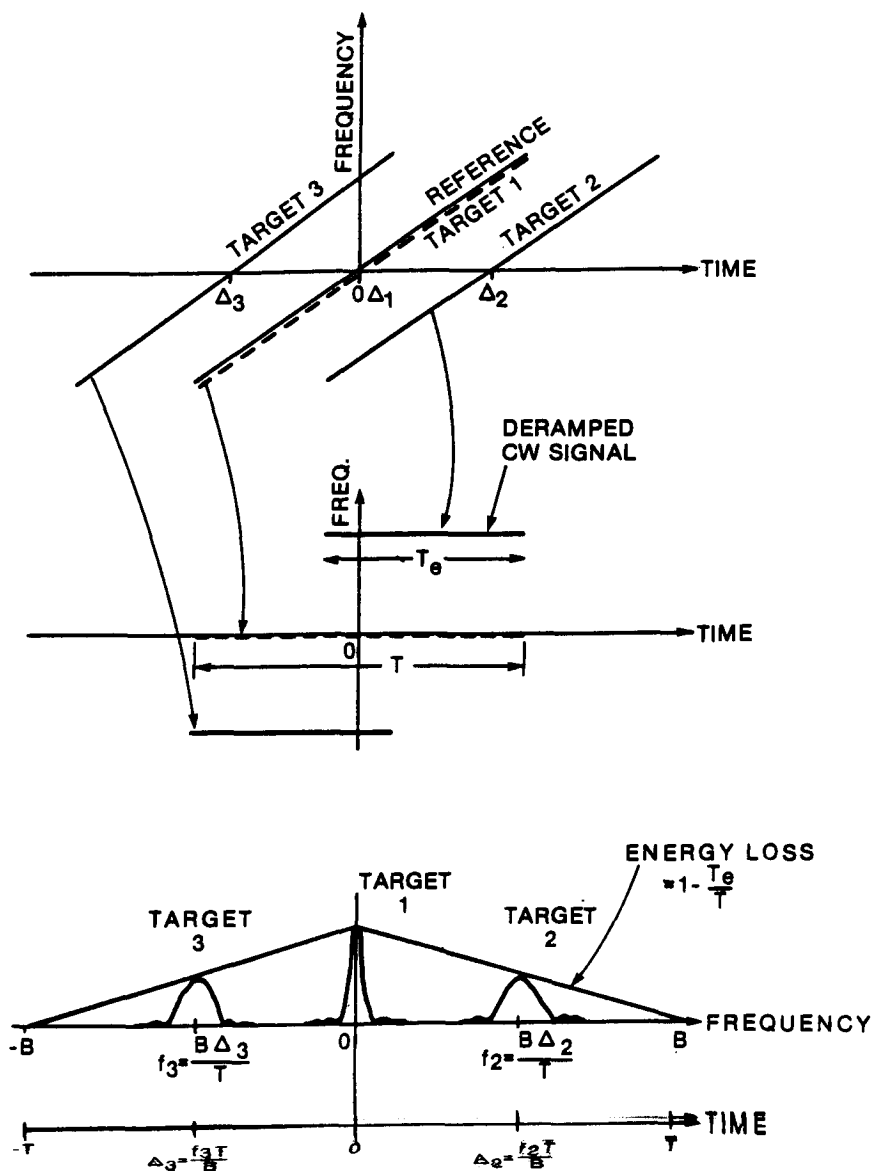
Fig. 32 - Conventional deramping technique for multi-targets.
