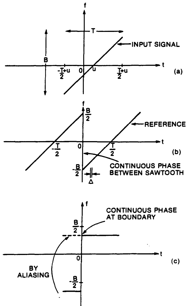
Fig. 34 - The spectral analysis method.
