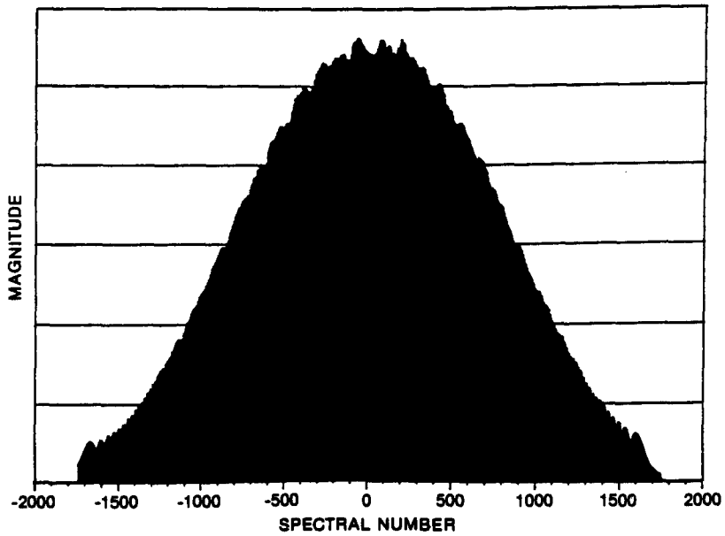
Fig. 15 - Spectrum of Figure 14 with Hamming weighting.
