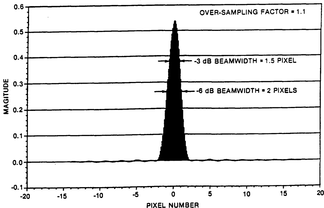
Fig. 13 - Compressed range pulse with Hamming weighting.
