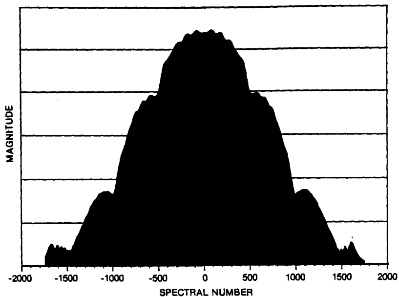
Fig. 19 - Spectrum of Figure 18 with Hamming weighting.
