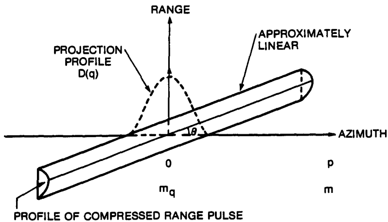
Fig. 25 - Range-azimuth coupling.
