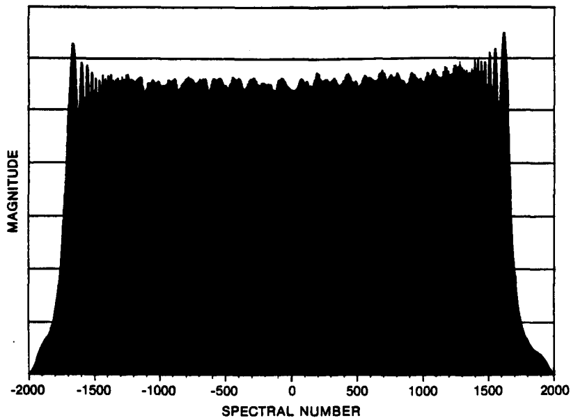
Fig. 14 - Azimuth spectrum continuous range curvature compensation.
