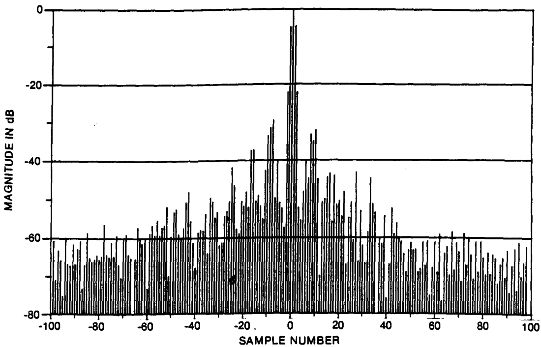
Fig. 22 - Compressed pulse with piecewise range curvature.
