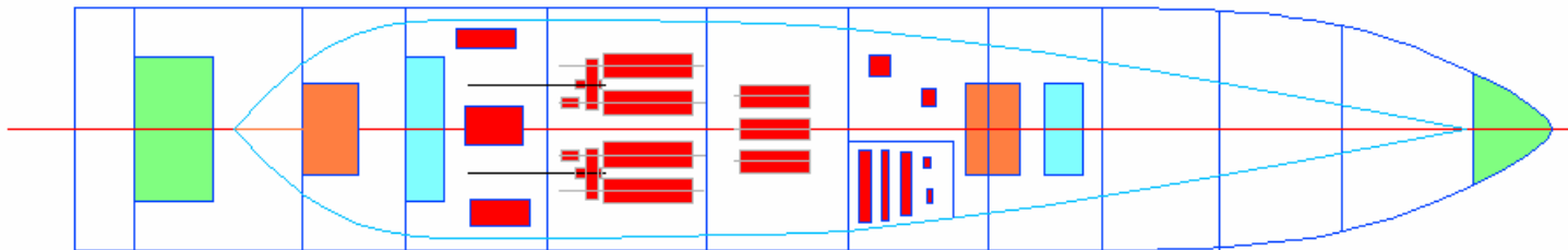
Figure 5 - Machinery Layout
