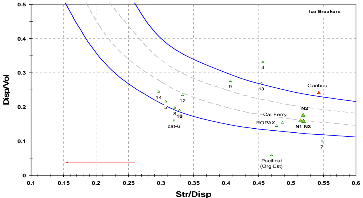
Figure 8 – Structural Density
