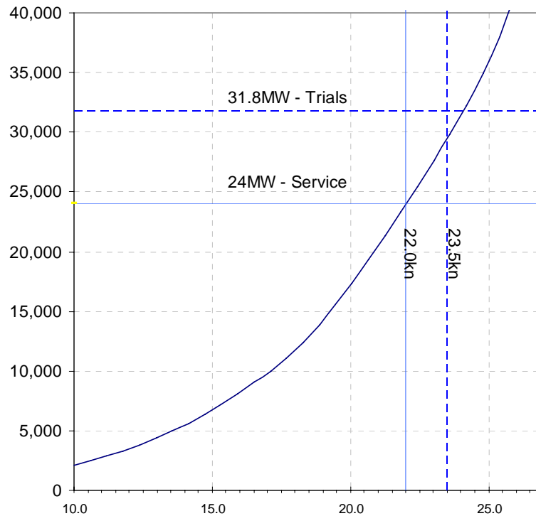
Figure 11 - Speed Power Curve
