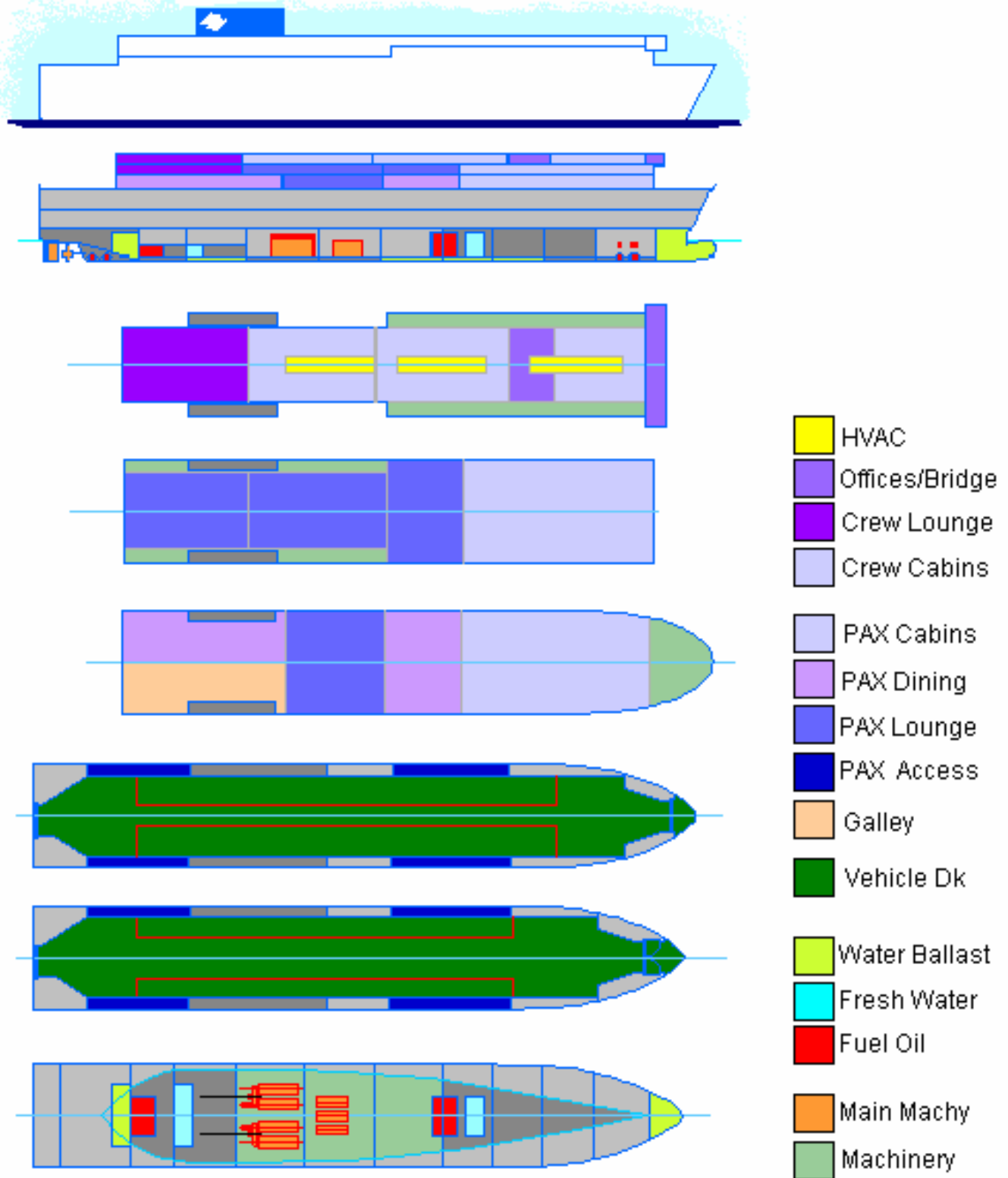
Figure 3 - General Arrangement
