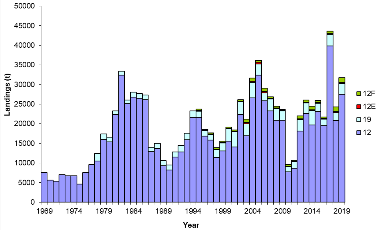
Figure 3. Landings (t) by fishing area and overall in the southern Gulf of Saint Lawrence snow crab fishery, 1969 to 2019.
