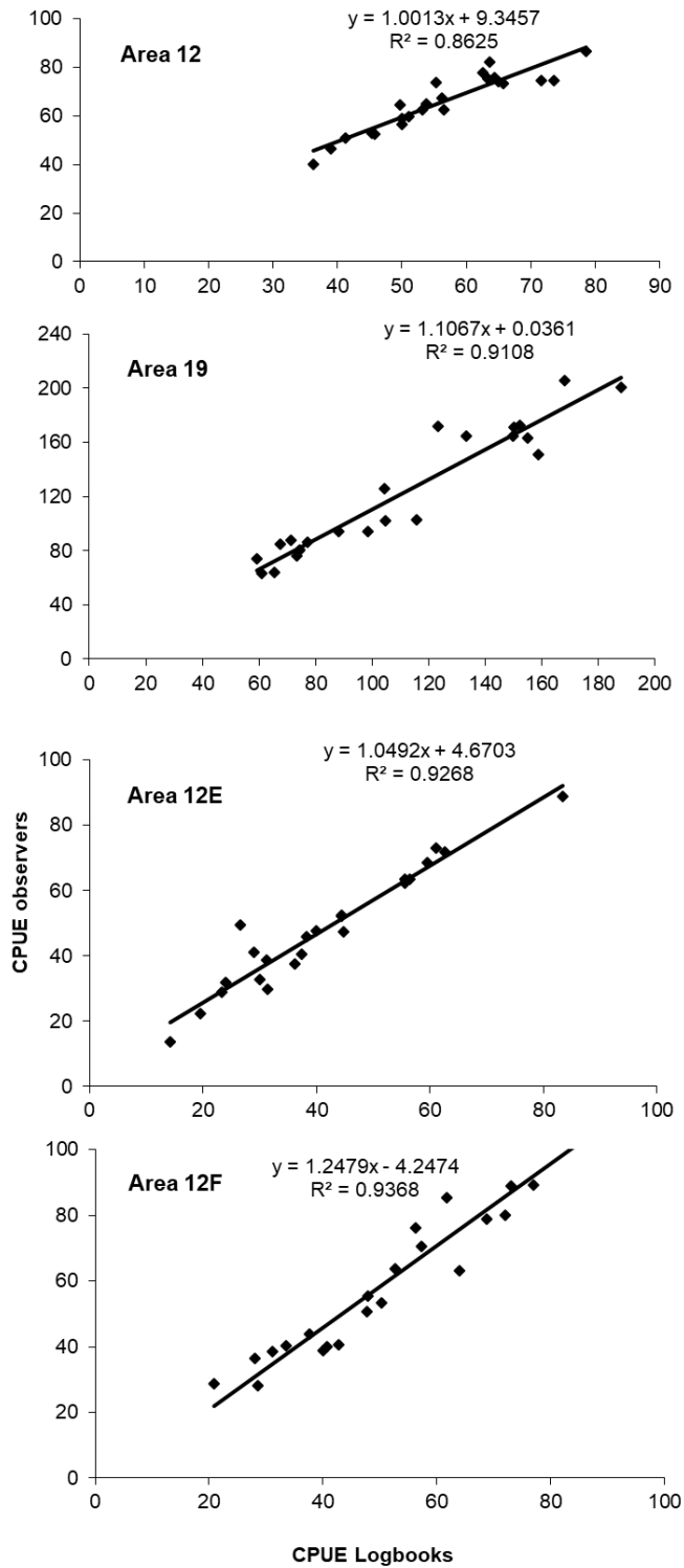
Figure 16. Relationship of catch-per-unit-of-effort (CPUE) between the logbook data and at-sea observer sampling by management area for 1997 to 2019.
