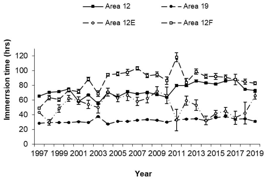
Figure 7. Mean (and one standard error bars) reported immersion time (hours) of traps by management areas in the southern Gulf snow crab fisheries, 1997 to 2019.
