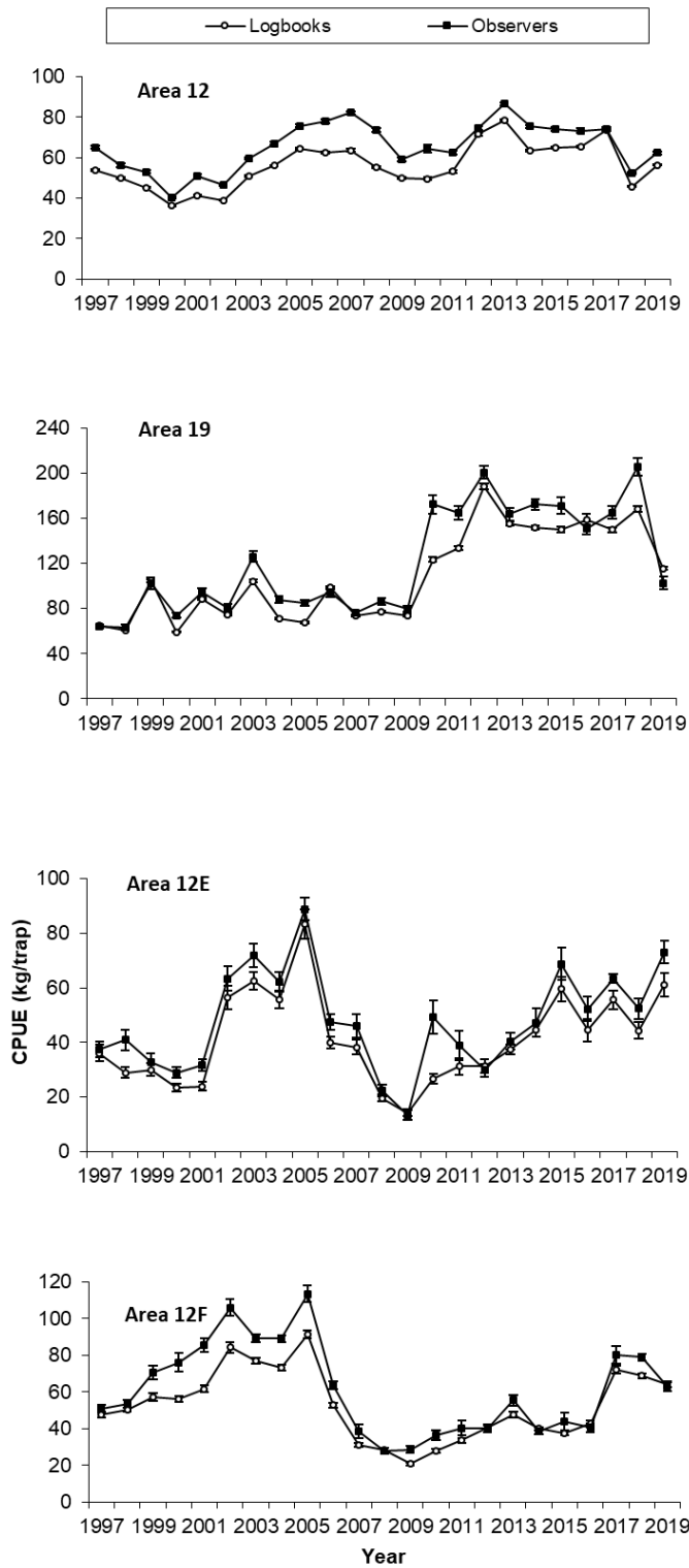
Figure 9. Comparison of catch-per-unit-of-effort (CPUE;kg / th, mean and one standard error bars) between the logbook data and at-sea observer sampling data by management area for 1997 to 2019.
