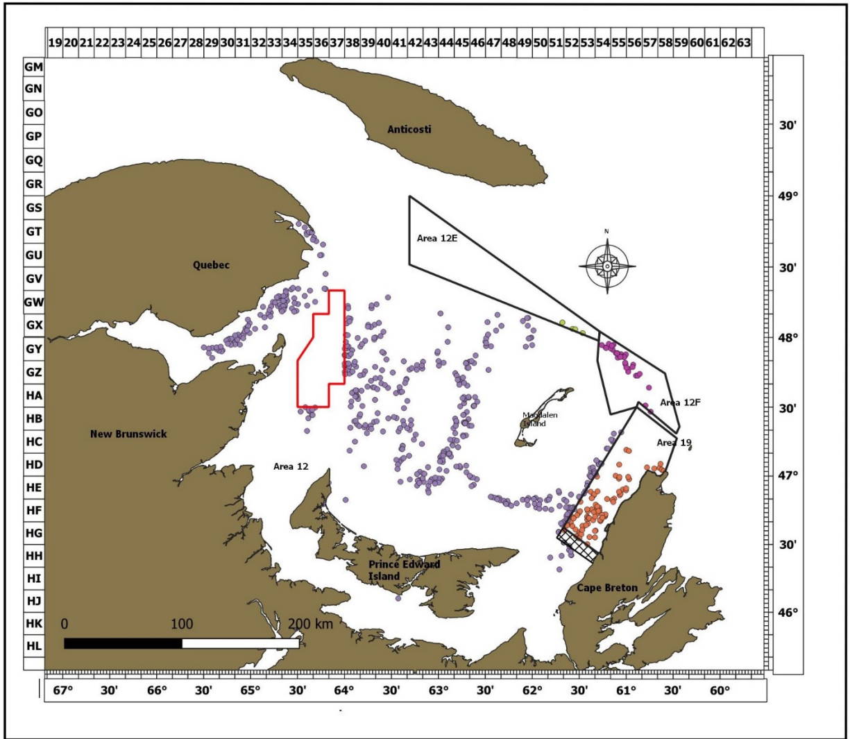
Figure 2. Locations of traps sampled aboard snow crab fishing vessels within the management areas of the southern Gulf of St. Lawrence during the 2019 fishing season.
