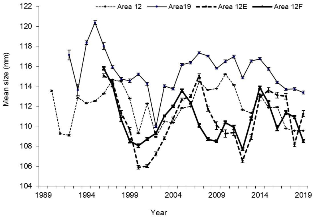
Figure 11. Carapace width (mm; mean and one standard error bar) of commercial-sized adult male snow crab in the catches from management areas 12, 19, 12E, and 12F for 1990 to 2019.
