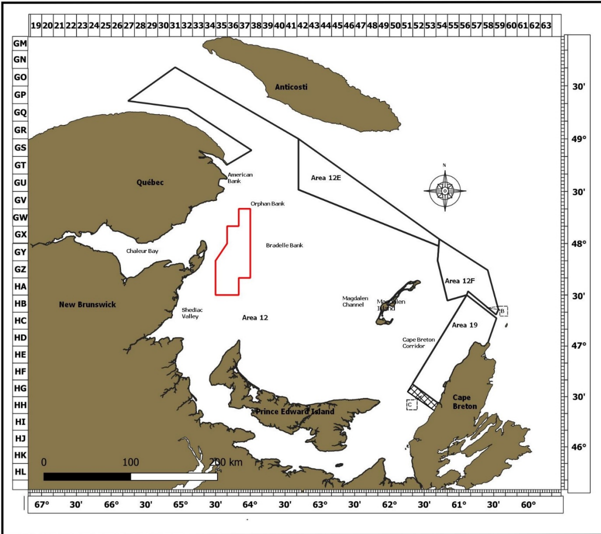
Figure 1. Locations of snow crab ( Chionoecetes opilio ) fishing grounds and management areas in the southern Gulf of St. Lawrence. Areas B and C are buffer zones. The red zone is the static zone (area closed for the fishery) introduced for the 2019 fishery to minimize the interactions with the North Atlantic right whales.
