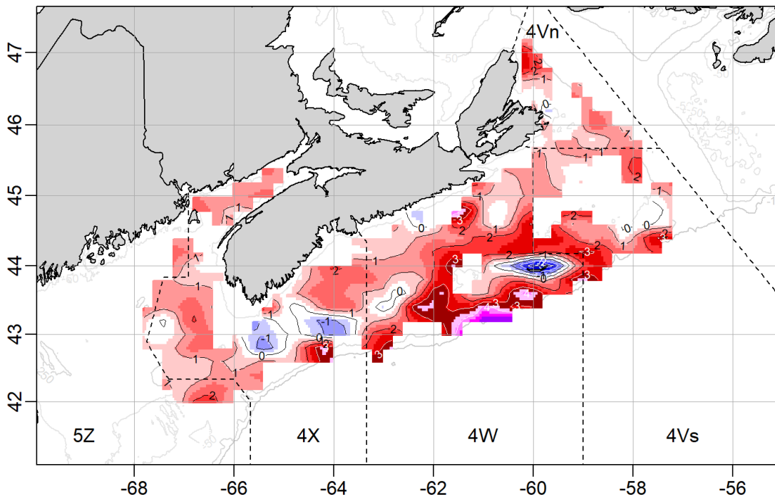
Figure 32. Bottom temperature anomalies (°C) from the 2020 DFO Summer RV Survey.
