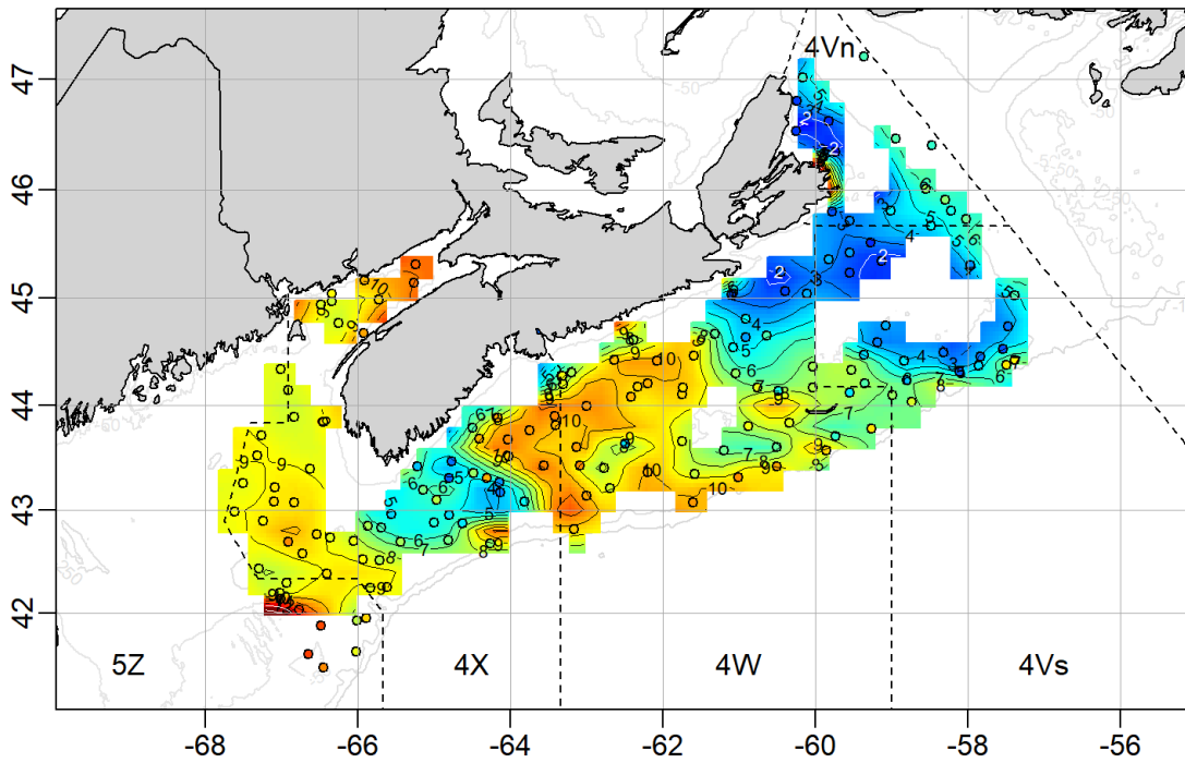
Figure 31. Bottom temperatures (°C) from the 2020 DFO Summer RV Survey.
