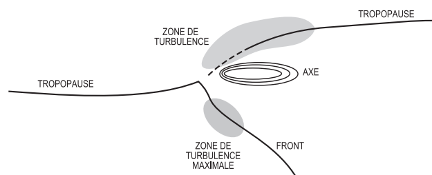
Figure 2.8 – Turbulence en air clair
