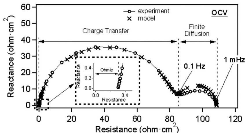
FIGURE 4 Measured complex impedance spectrum of a V(II)/V(III) single layer anode, at 30^\circ\text{C} and flow rate of 1.5 \text{ mL min}^{-1} (reproduced and modified with permission from ECS) 113
