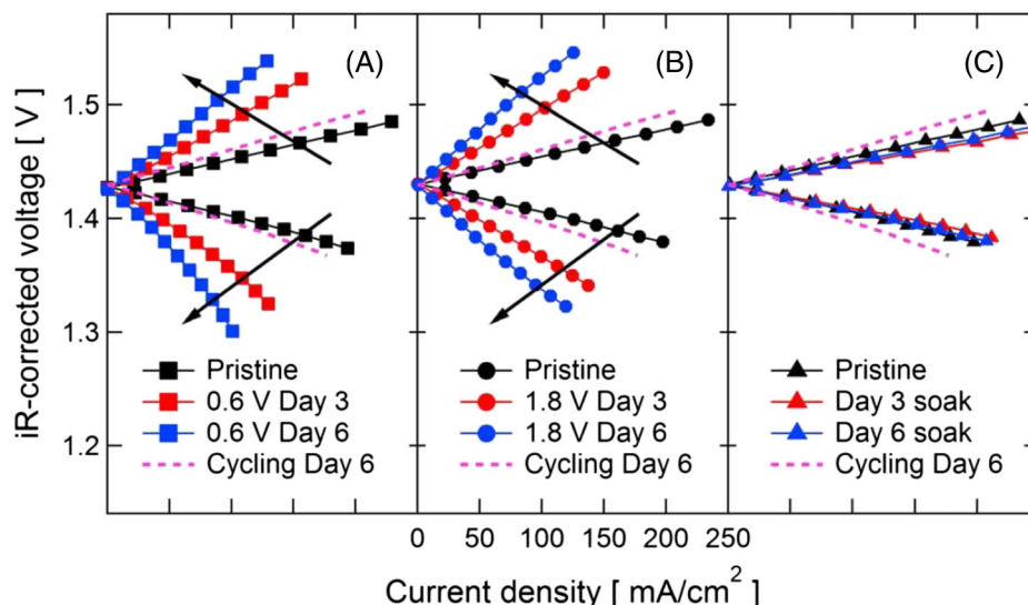
FIGURE 12 iR-corrected polarization curves taken after initial build, 3 and 6 day: (A) cell-in-series experiment E: potential hold at 0.6 V and at low SOC; (B) cell-in-series experiment F: potential hold at 1.8 V and at high SOC; and (C) soaked in high SOC solution; curve for cell cycled for 6 days shown for 160 (reproduced with permission from ECS) [Colour figure can be viewed at wileyonlinelibrary.com ]
