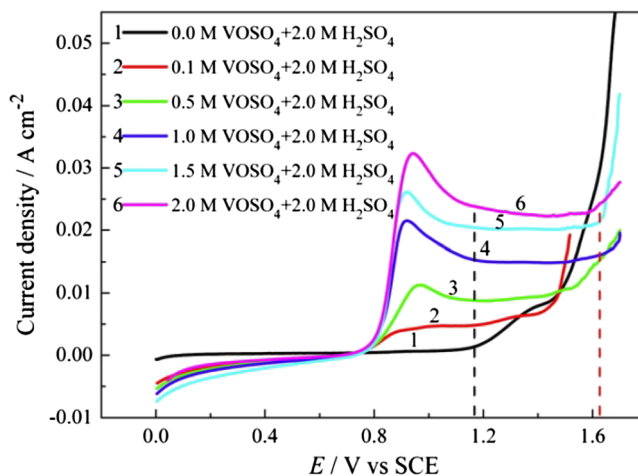
FIGURE 5 Linear sweep voltammograms of graphite electrodes in different concentrations of \text{VOSO}_4 with 2M \text{H}_2\text{SO}_4 at a scan rate 114 of 5 \text{ mV s}^{-1} (reproduced with permission from Elsevier) [Colour figure can be viewed at wileyonlinelibrary.com ]
