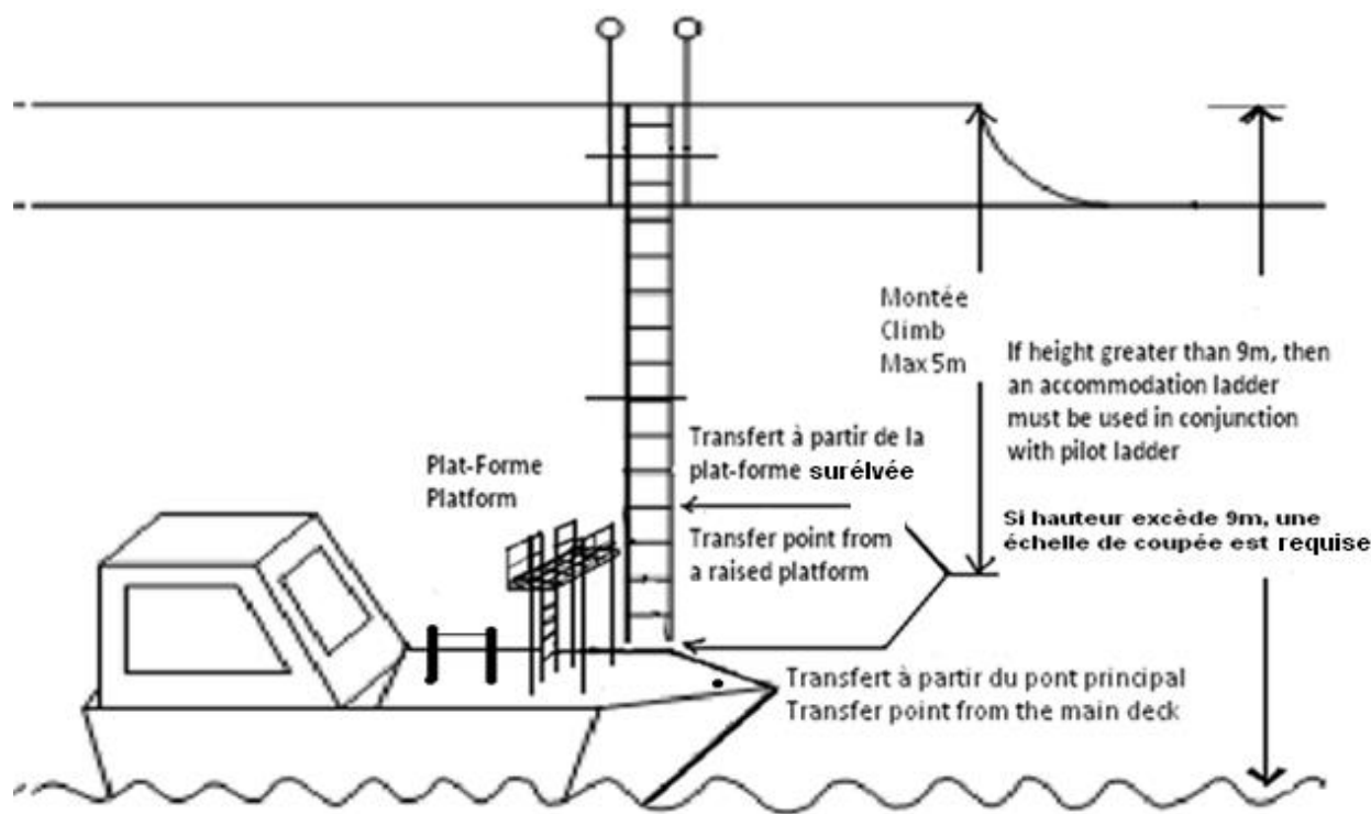
FIGURE 3: CLIMB ON THE PILOT LADDER MUST NOT EXCEED 5 METRES
