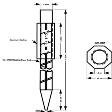
Figure 1 - CLS 77 Post
