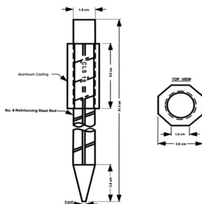
Figure 1: Borne ATC 77
