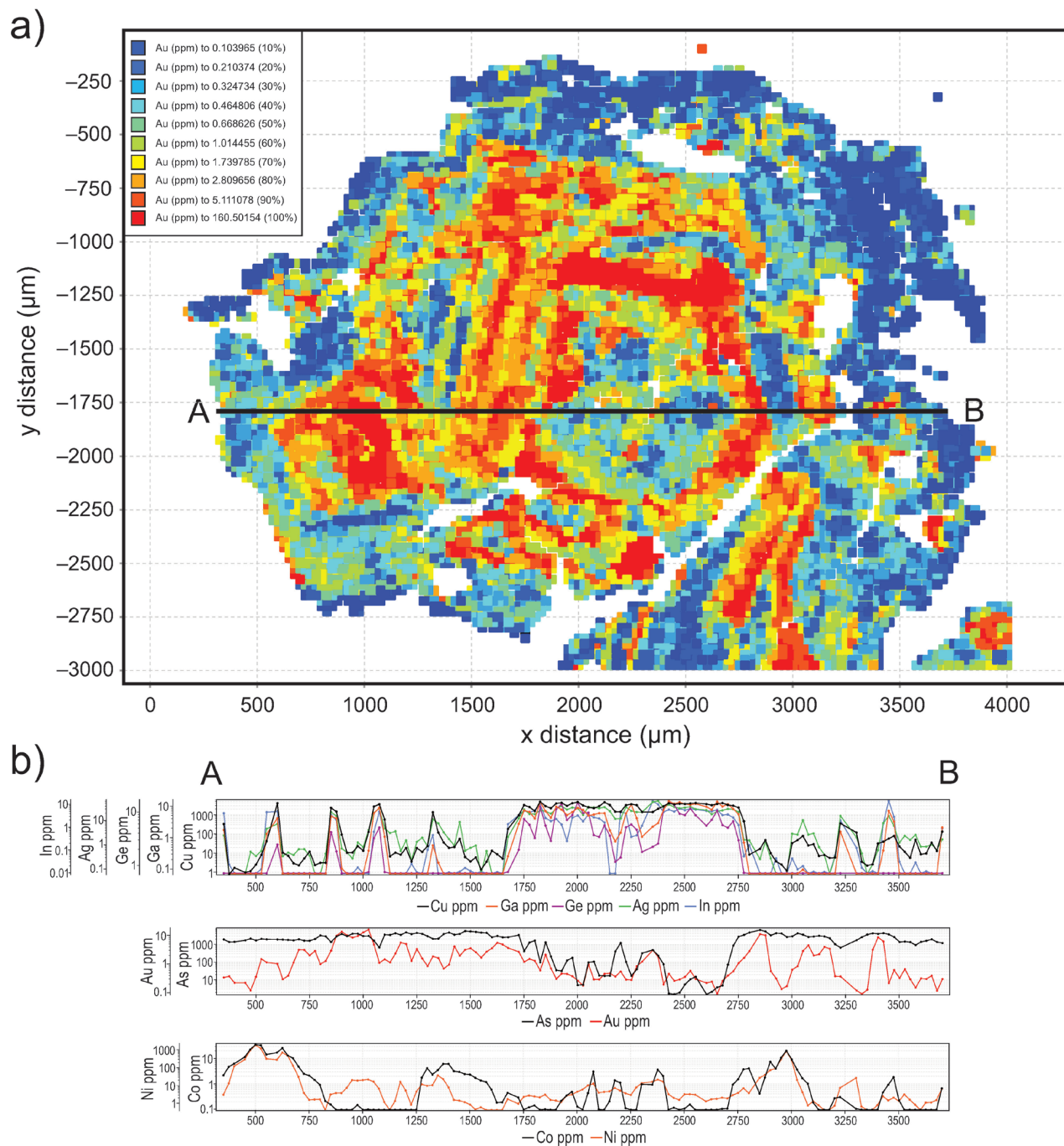
Figure 11. a) Laser-ablation inductively coupled plasma mass spectrometry (LA-ICP-MS) Au distribution map of a pyrite grain in sample 08-SP-155 from the Abbott-Wagner deposit, generated with ioGAS, and b) trace-element profiles along a linear transect (black line A–B). Pixels are assigned colours based on concentration ranges (in ppm) determined from the LA-ICP-MS data.
