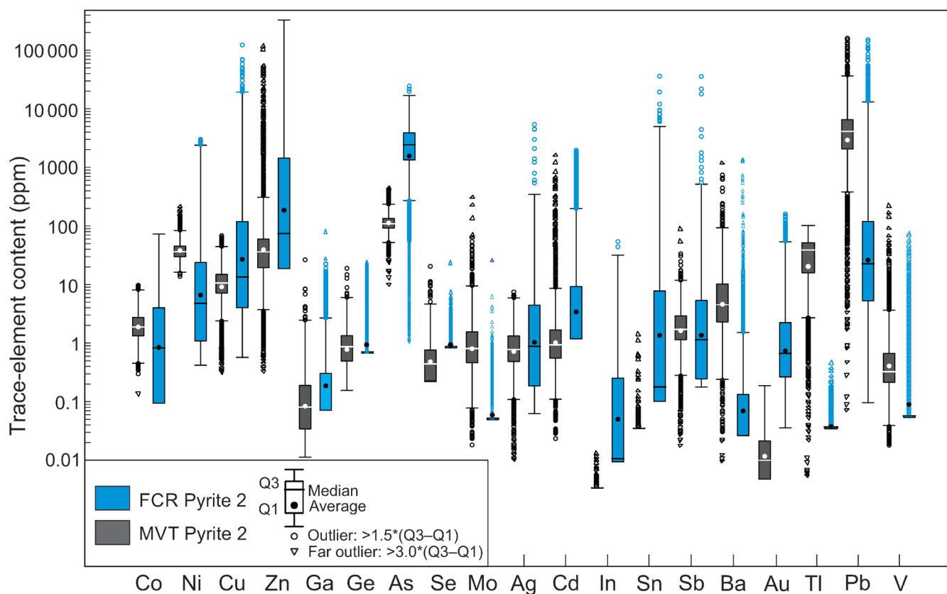
Figure 10. Box and whisker plots of trace-element contents of Pyrite 2 in Mississippi Valley-type and fracture-controlled replacement deposits. Except for V, elements follow are listed from left to right in order of increasing atomic number and atomic weight. Concentrations span eight orders of magnitude. Symbols: Q3 = top of box; Q1 = bottom of box; black circle = average; line = median. The central box is the middle 50% of the data from Q1 to Q3. An outlier (circle) is further than 1.5 \times (Q3 - Q1) from the box. A far outlier (triangle) is further than 3.0 \times (Q3 - Q1) from the box. The whiskers are the extreme values that are not outliers.
