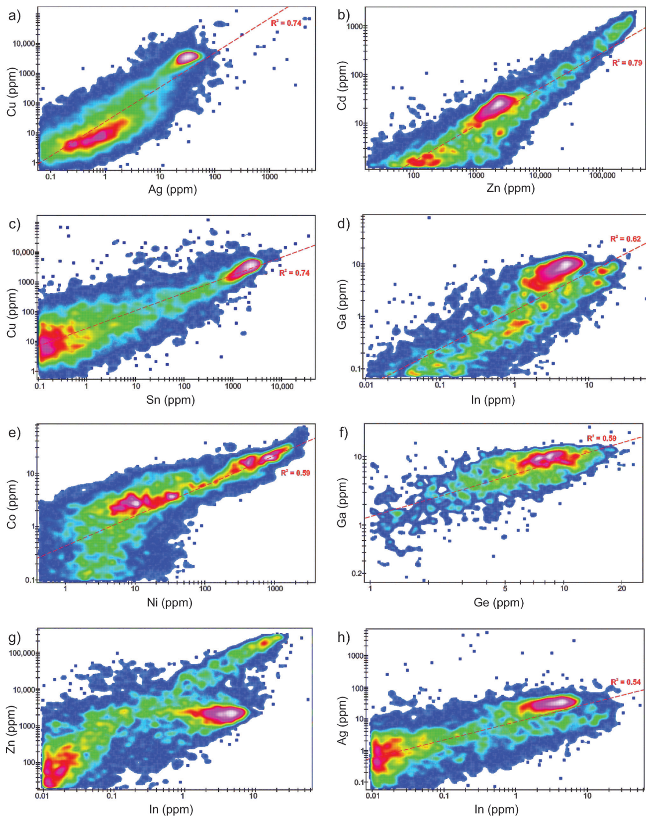
Figure 12. Binary plots of laser-ablation inductively coupled plasma mass spectrometry (LA-ICP-MS) data for pairs of trace elements with high to low levels of covariance throughout Pyrite 2 from sample 08-SP-155 from the Abbott-Wagner fracture-controlled replacement deposit. The variation of colours from blue to pink corresponds to an increase in point density: a) Cu vs. Ag; b) Cd vs. Zn; c) Cu vs. Sn; d) Ga vs. In; e) Co vs. Ni; f) Ga vs. Ge; g) Zn vs. In; h) Ag vs. In.
