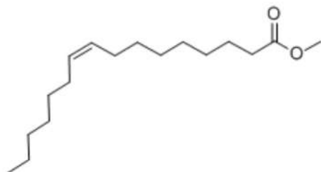
Figure 5. Palmitoleic acid methyl ester (C16)
