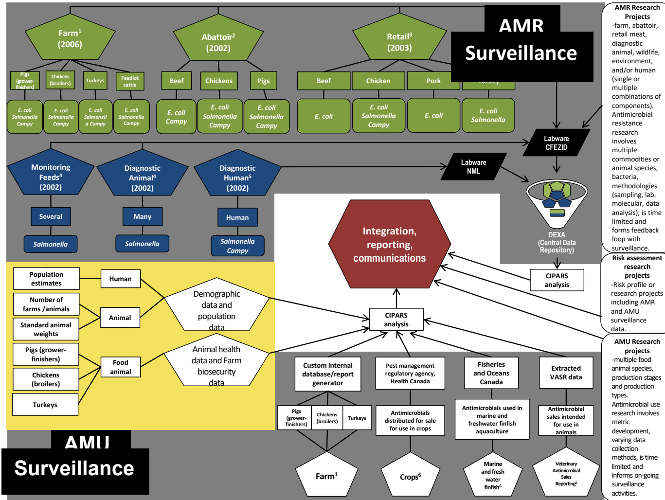
Figure A. 1 Summary of the CIPARS samples and data flow, 2019
