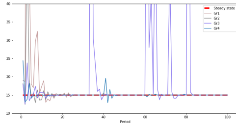
(b) \lambda = 3.5
