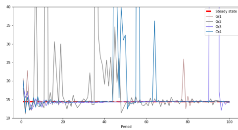
(e) \lambda = 3.9
