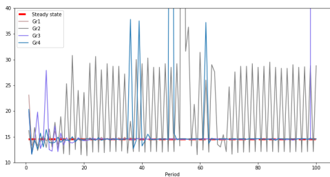
(c) \lambda = 3.8
