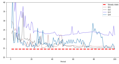
(b) \lambda = 3.8
