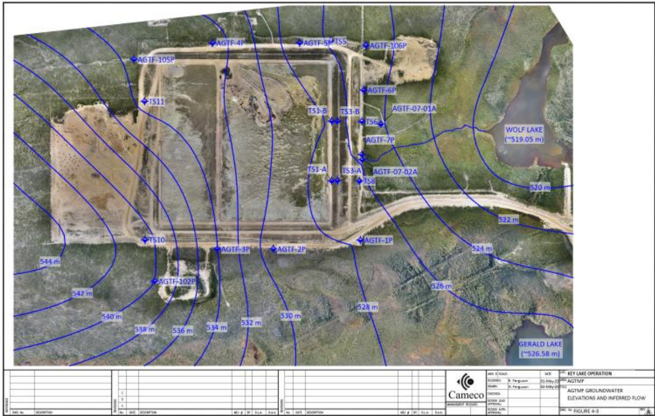
Figure 3.4: Groundwater flow directions at the AGTMF [63]
