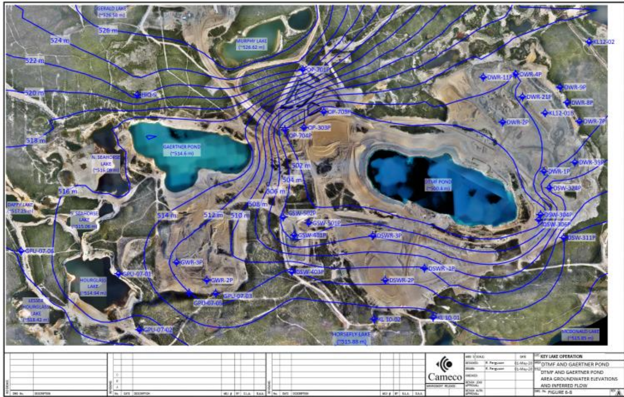
Figure 3.6: Groundwater flow directions at the DTMF [63]
