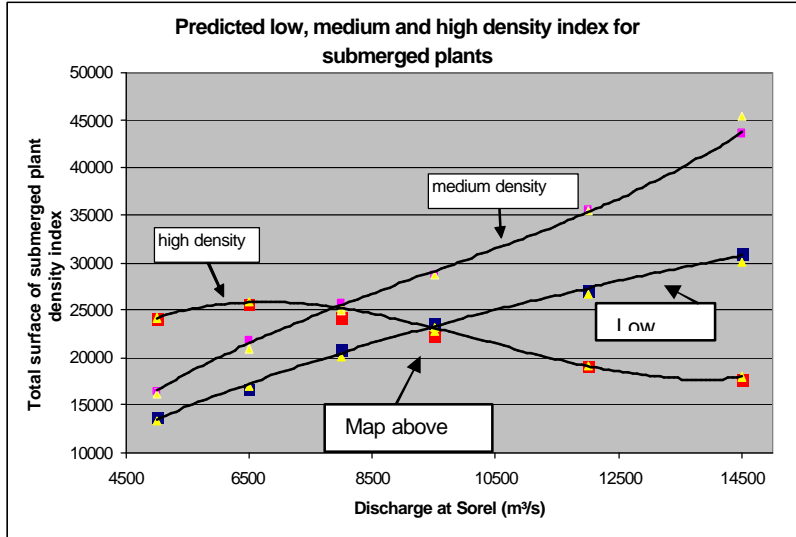
Figure: Relation between the 2D modeling of density classes and the discharge in Sorel, data and best fit curve: Low_Density (ha) = -3446.7646 + (4.2428 * Q\_Sorel) - (0.0002 * Q\_Sorel^2) + (0.00000000462 * Q\_Sorel^3) , with r^2 = .9923 Medium_Density (ha) = 5337.9319 + 8.3607 * Q\_Sorel - 0.0008 * Q\_Sorel^2 + 0.0000000266 * Q\_Sorel^3 , with r^2 = .9978 High_Density (ha) = 0.0000000452 * Q\_Sorel^3 - 0.001397 * Q\_Sorel^2 + 12.68 * Q\_Sorel - 10000 , with r^2 = .9855
