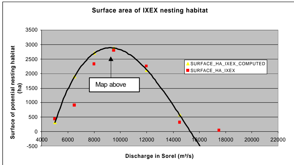
Figure: Relation between the calculated surface area for IXEX nesting habitat and the discharge in Sorel, data and best fit curve : IXEX\_COMPUTED = 0.0000000066 * Q\_Sorel^3 - 0.0003 * Q\_Sorel^2 + 3.8463 * Q\_Sorel - 12244 , with r^2 = .9241
