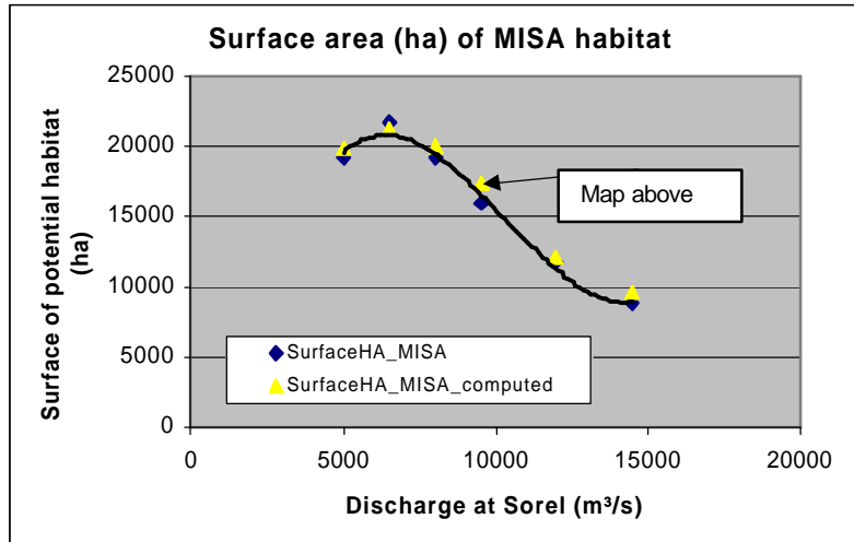
Figure: Relation between the calculated "Surface area of potential habitat" for MISA and the discharge in Sorel, data and best fit curve: MISA = 0.0000000482 * (Q\_Sorel)^3 - 0.0015 * (Q\_Sorel)^2 + 13.341 * (Q\_Sorel) - 15340
