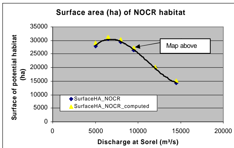
Figure: Relation between the calculated "Surface area of potential habitat" for NOCR and the discharge in Sorel, data and best fit curve: \text{NOCR} = 0.000000051 * (Q\_Sorel)^3 - 0.00169 * (Q\_Sorel)^2 + 15.79 * (Q\_Sorel) - 14000
