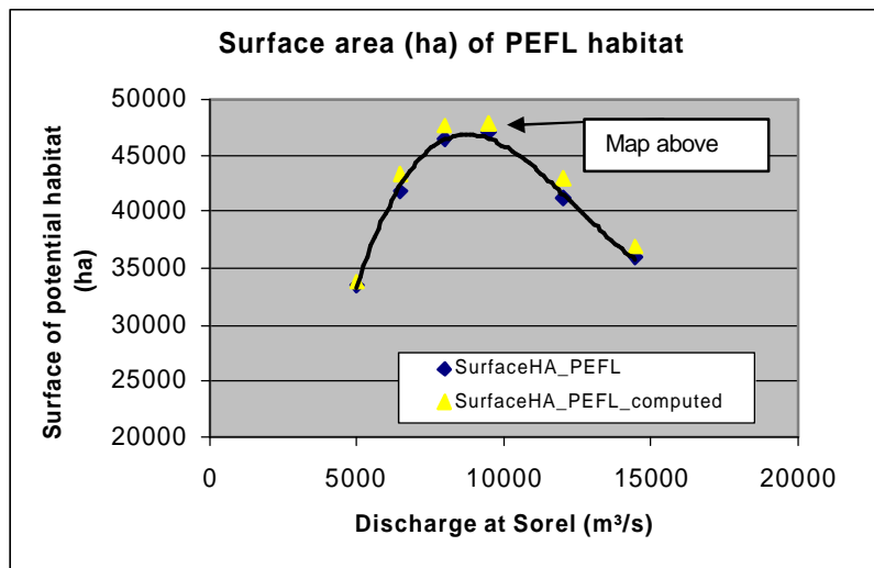
Figure: Relation between the calculated "Surface area of potential habitat" for PEFL and the discharge in Sorel, data and best fit curve: PEFL=0.0000000635*(Q\_Sorel)^3 - 0.0024*(Q\_Sorel)^2 + 27.573*(Q\_Sorel) - 51926
