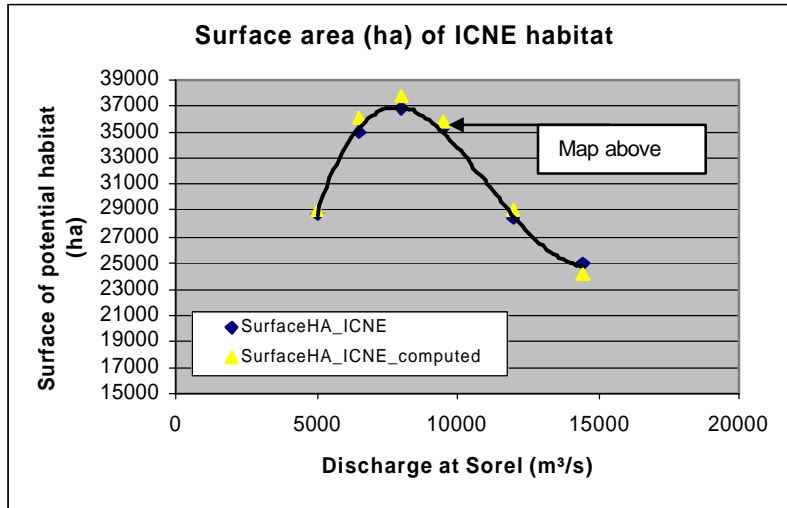
Figure: Relation between the calculated “Surface area of potential habitat” for ICNE and the discharge in Sorel, data and best fit curve: ICNE=0.0000000792*(Q\_Sorel)^3 - 0.0027*(Q\_Sorel)^2 + 27.747*(Q\_Sorel) - 51998
