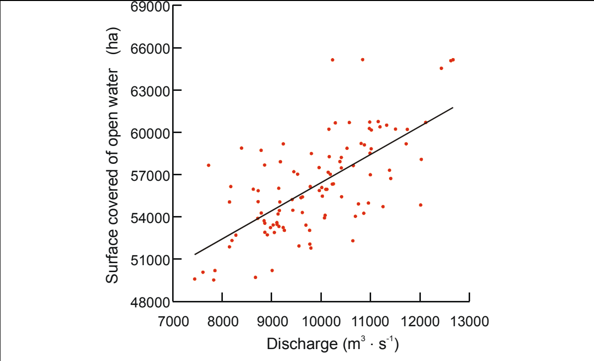
Figure 10. Relationship between estimated surface covered by open water (logistic regression) and discharges in the Saint-Lawrence River from 1900 to 2000.
