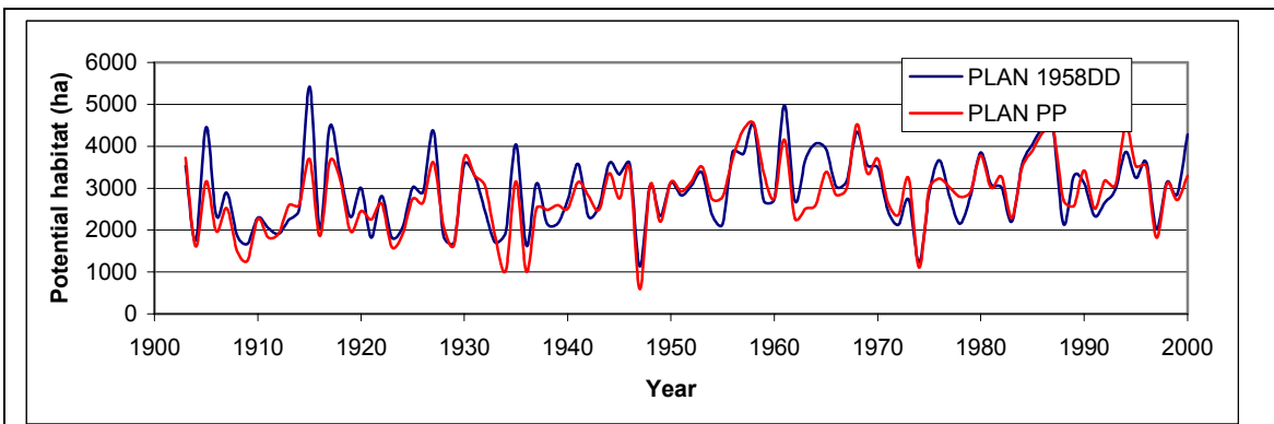
Figure 8. Comparison of reproductive habitat surface area for the frog for Plan 1958DD and Plan PP
