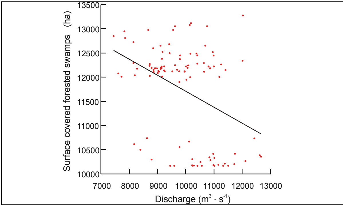
Figure 13. Relationship between estimated surface covered by forested swamps (logistic regression) and discharges in the Saint-Lawrence River from 1900 to 2000.
