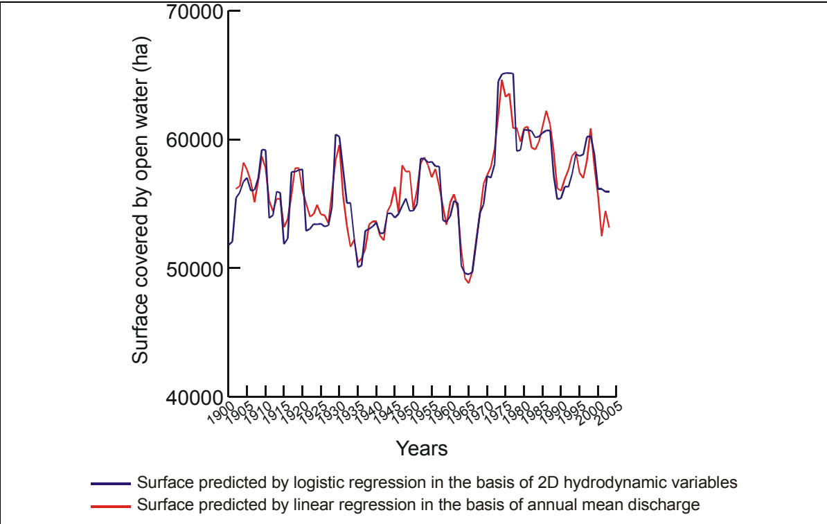
Figure 11. Relationship between surface covered by open water (ha) from 1900 to 2000.
