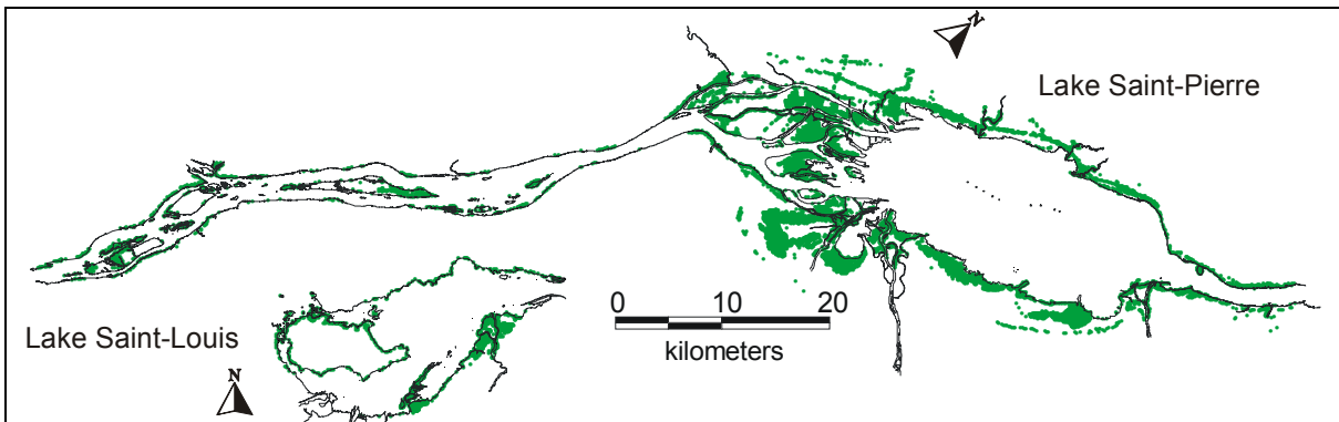
Figure 12. Distribution of forested swamps, predicted by logistic regression for the St. Lawrence River floodplain in 1985 (mean discharge = 11503 \text{ m}^3 \cdot \text{s}^{-1} )
