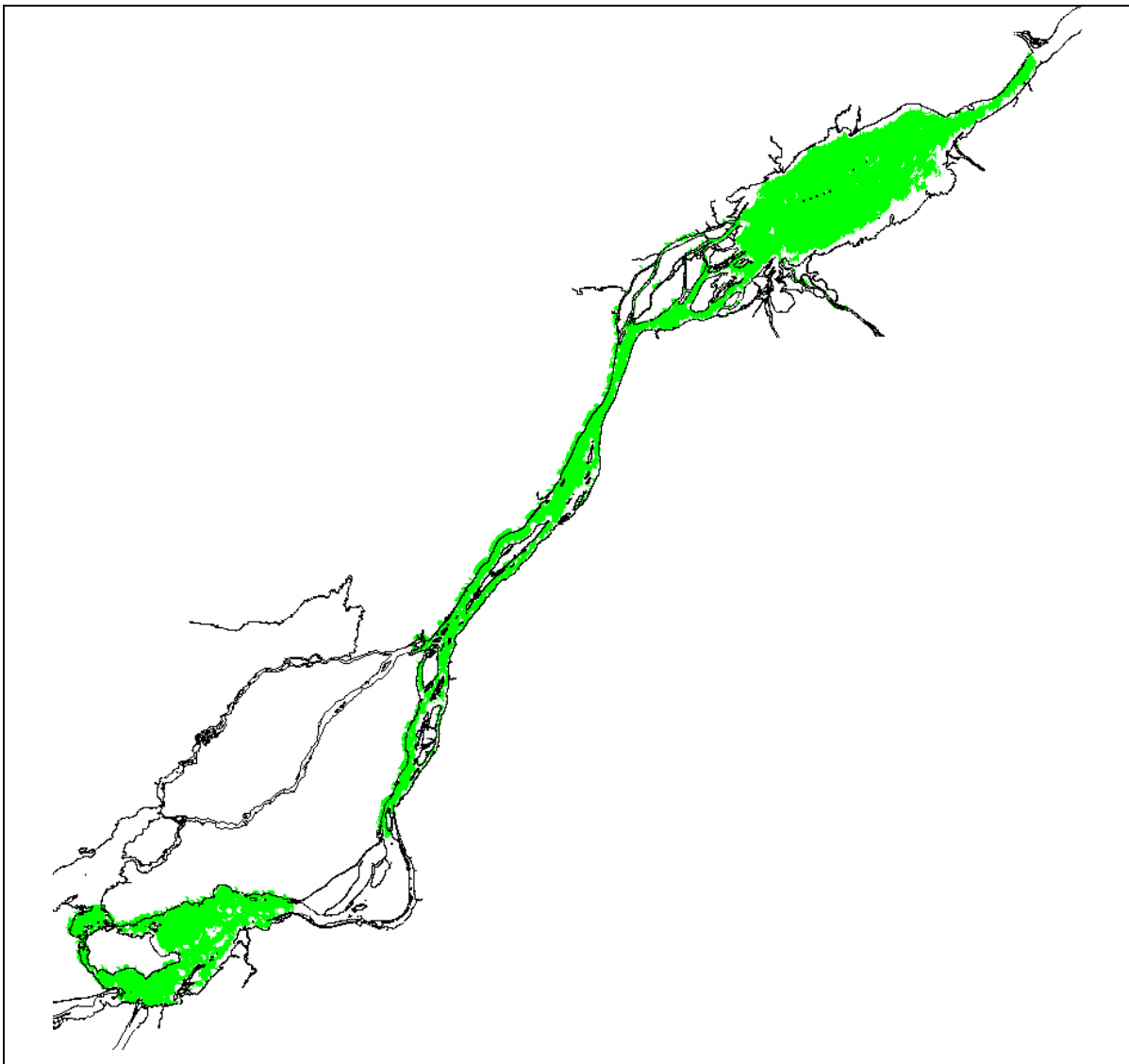
Figure 3. Map of the suitable habitat (feeding and living) for the Walleye ( Stizostedion vitreum ) for an average discharge (9500 m 3 /s at Sorel)
