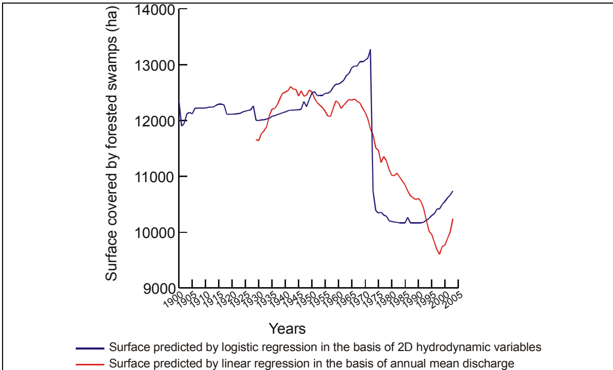
Figure 14. Relationship between surface covered by forested swamps (ha) according to years from 1900 to 2000.
