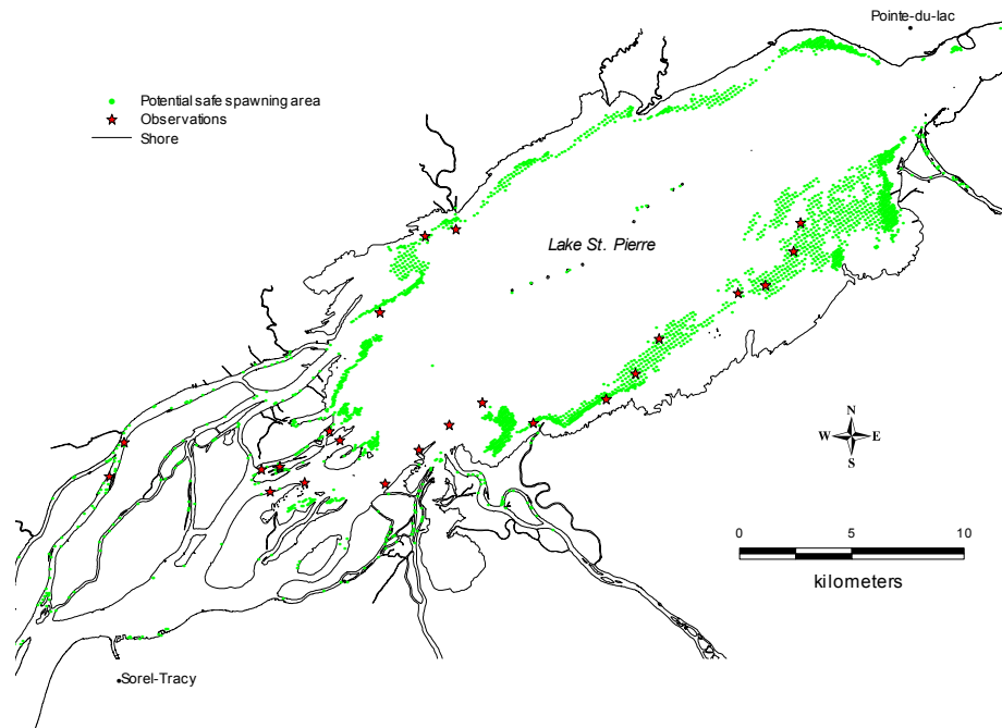
Figure 25. Map of the 2D habitat model for the Bridler shiner, in Lake Saint-Pierre (1995 designated quarter month)
