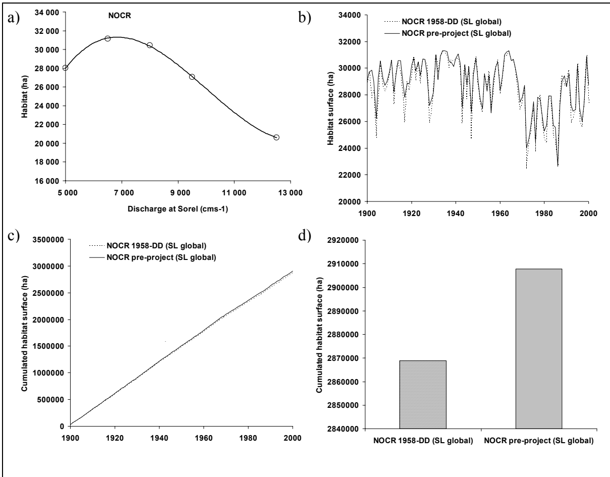
Figure 2. (a) Global relationship between “Surface area of suitable summer habitat” for NOCR and the discharge in Sorel; (b) suitable average summer habitat (ha) for the period 1900-2000, calculated with the 1958-DD and Pre-project Plans; (c) cumulated suitable habitat (ha) over time for the period 1900-2000; (d) difference in suitable habitat between the two scenarios 1958-DD and Pre-Project after 100 years.
