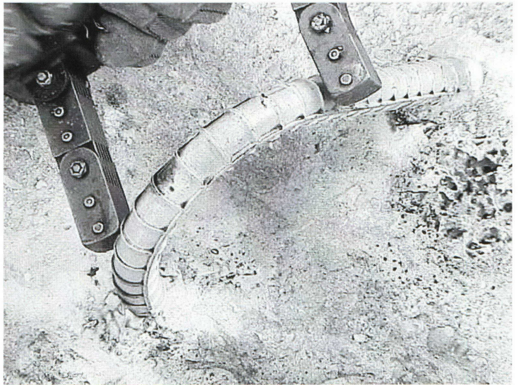
Figure 3: Magnetic Particle Inspections (Mpi)
