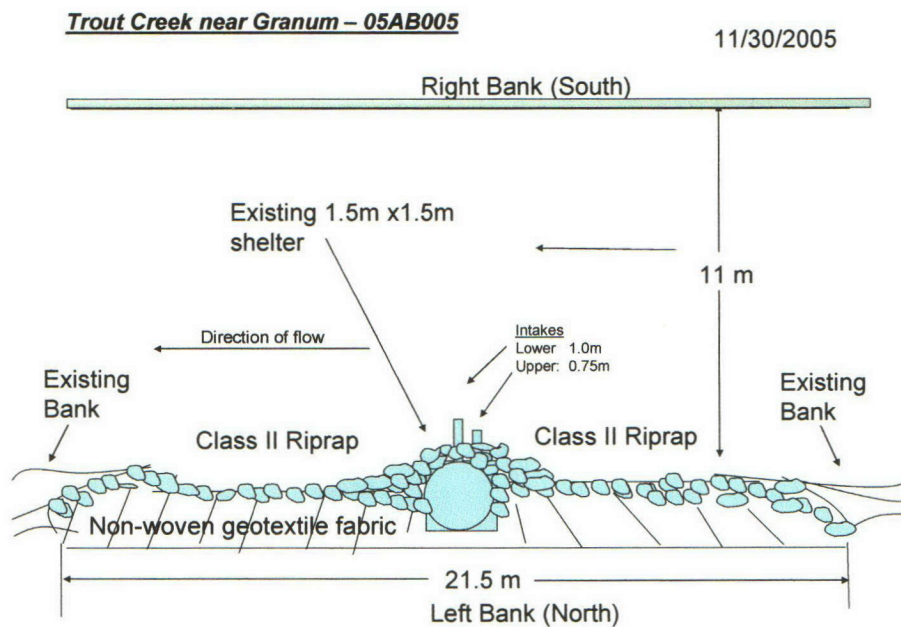
Figure 4: Trout Creek Shoreline remediation topo sketch
