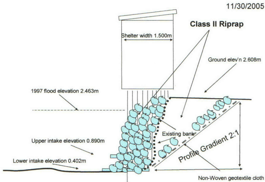
Figure 3: Trout Creek Shoreline remediation Plan Profile Sketch
