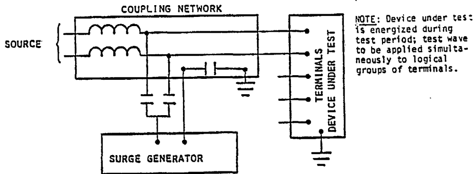
Fig. 1.A. Points of application for the SWC Common Mode Test
