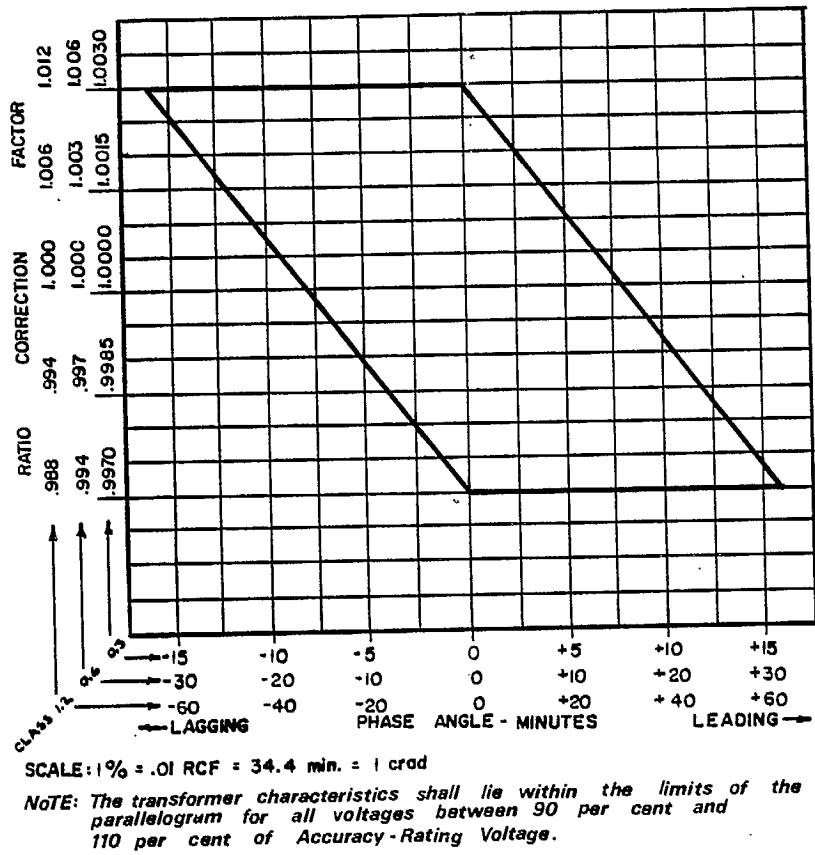
FIGURE 6 LIMITS OF ACCURACY CLASSES
