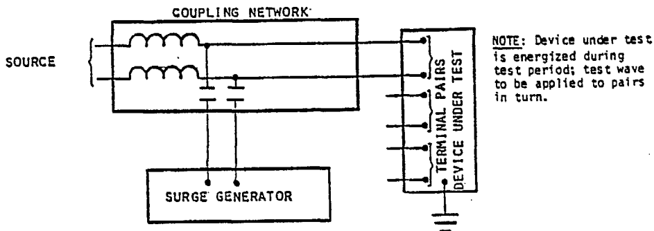
Fig. 1.A. Points of application for the SWC Common Mode Test
