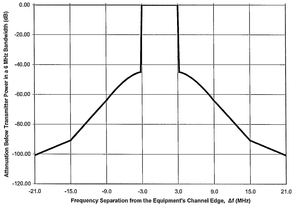
Figure 1 Unwanted Emissions Limits with \Delta f < 18 MHz
