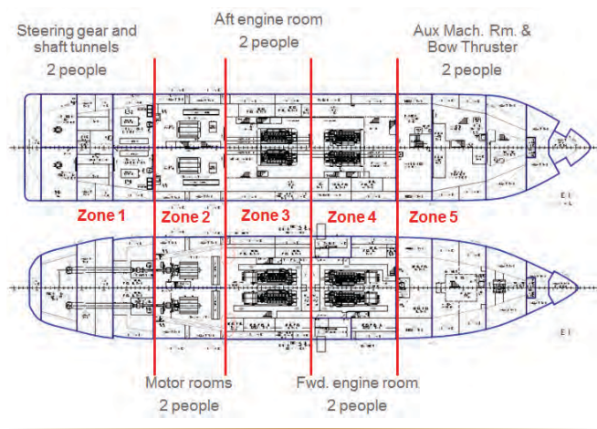
Zones checked during the roaming leak checks.
