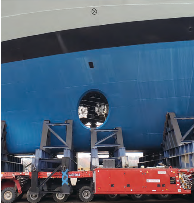
Figure 5. The AOPV transverse tunnel bow thruster.
