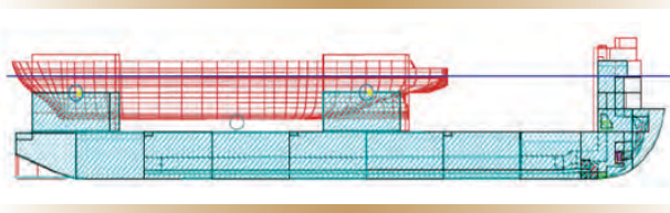
Depiction of Boa Barge 37 at maximum submersion.
