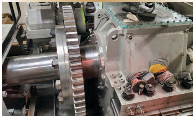
Figure 2. Thrust block and turning gear arrangement.
