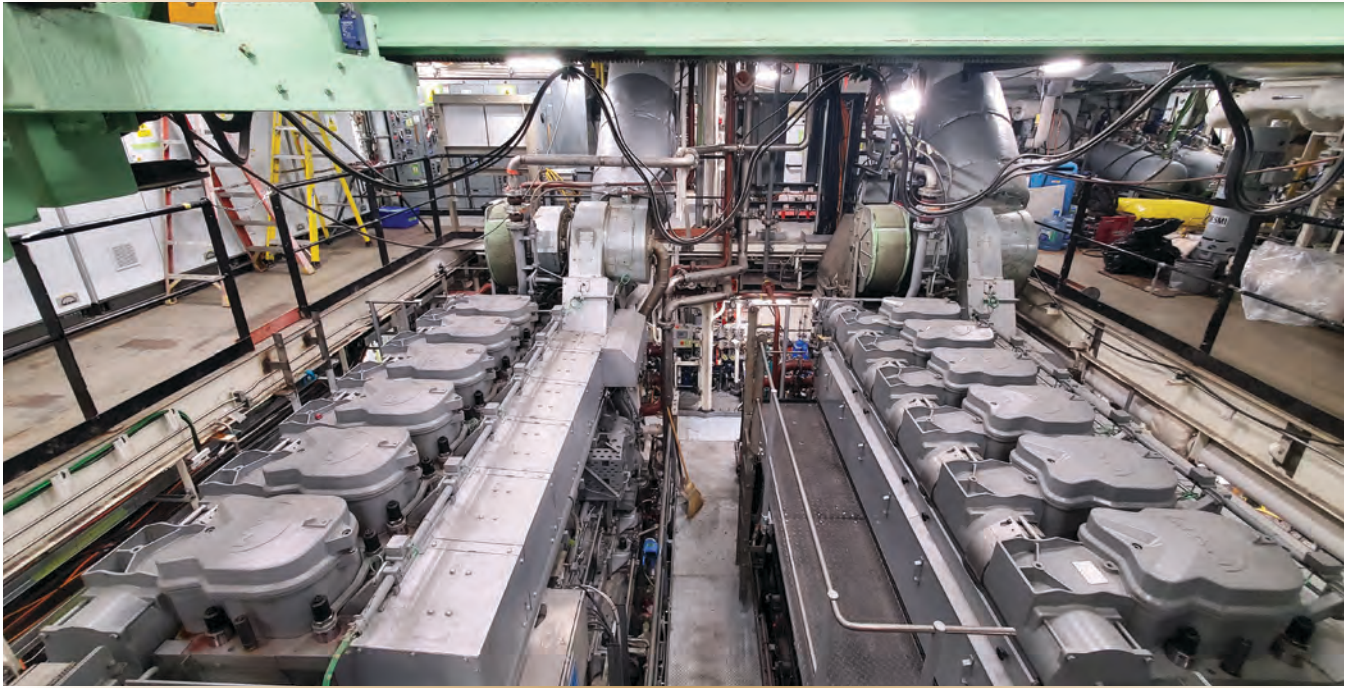
Figure 1. Two of the AOPV's four 3600-kW MAN diesel engines that provide electrical power for propulsion and ship electrical systems.
