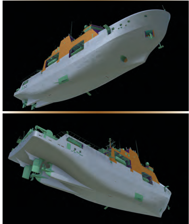
Figure 2. These computer modelling images from Irving Shipbuilding Inc. show how the geometry of the AOPV hull design has been optimized for ice breaking, as well as for seakeeping in support of helicopter operations and crew comfort. Crews have been reporting their satisfaction with the operation of these ships in all conditions.
