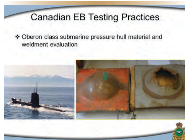
Figure 6. Oberon -class submarine explosion bulge test panels.
