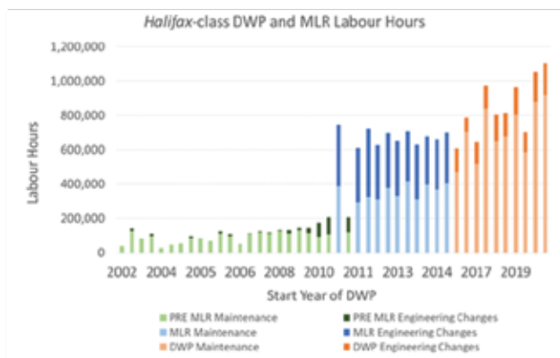
Figure 4. Docking work period labour hours increase at a roughly exponential rate for the Halifax class.
