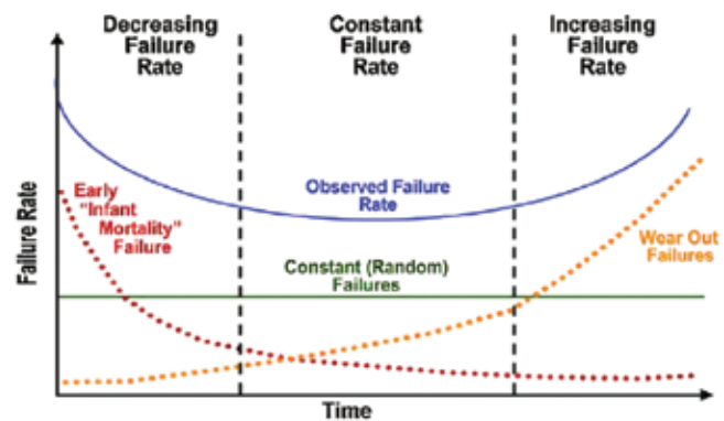
Figure 2. The bathtub curve is a combination of three separate and unequal failure distributions.
