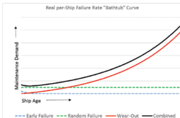
Figure 5. Properly sizing root cause distributions adjust the Navy per-ship bathtub curve to an almost purely exponential distribution.
