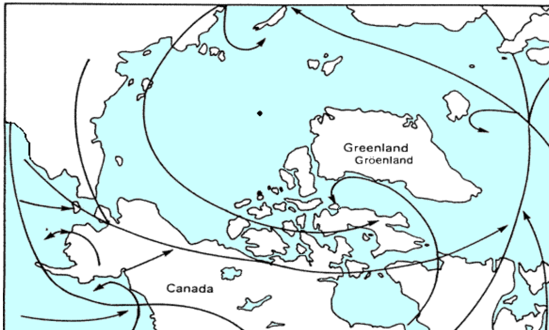
Figure 15 - Principal storm tracks in summer in Canadian Arctic
