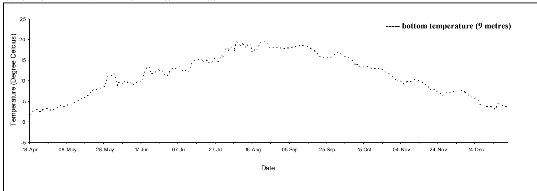
Daily mean temperature for Caribou, N.S., 2020.
