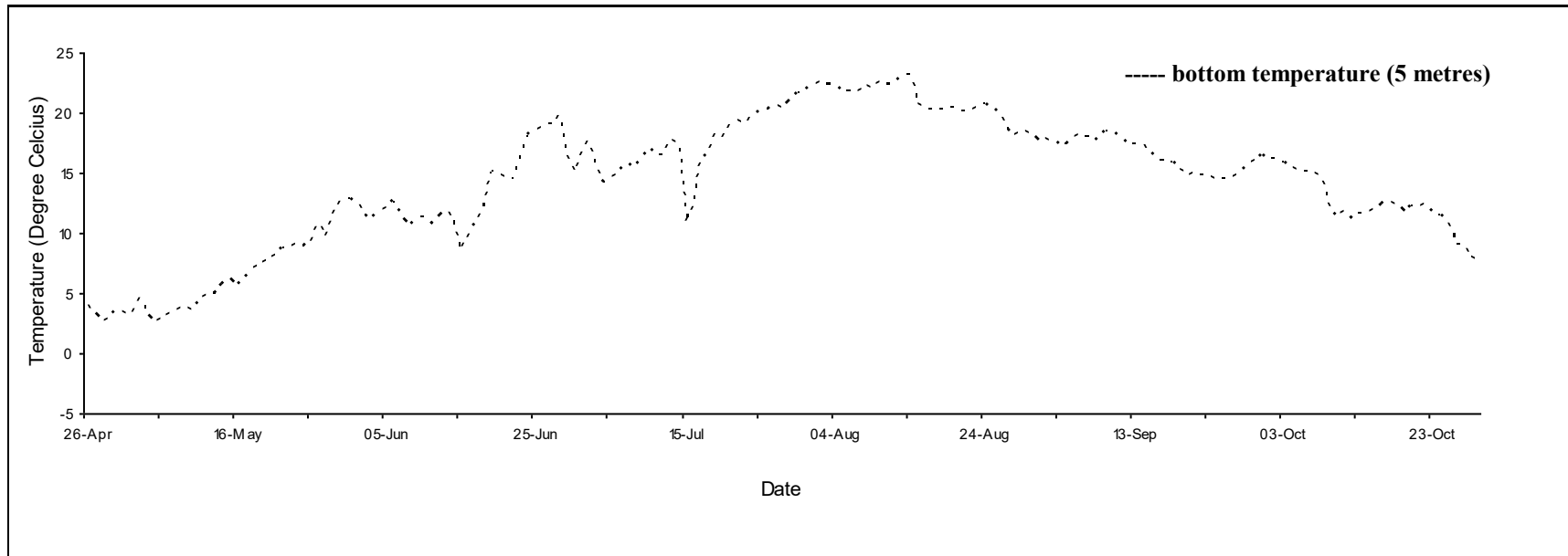
Daily mean temperature for St Peters, P.E.I., 2020.
