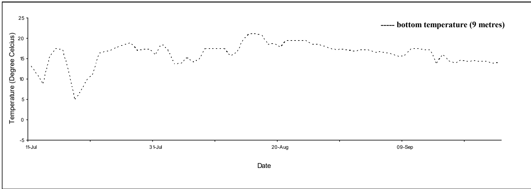
Daily mean temperature for Alberton, P.E.I., 2020.
