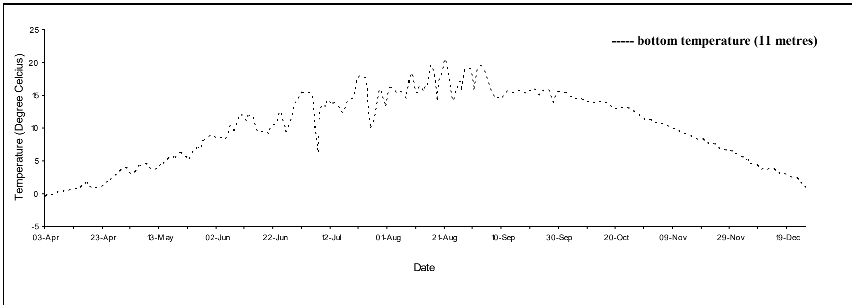
Daily mean temperature for Cascumpeque, P.E.I., 2021.
