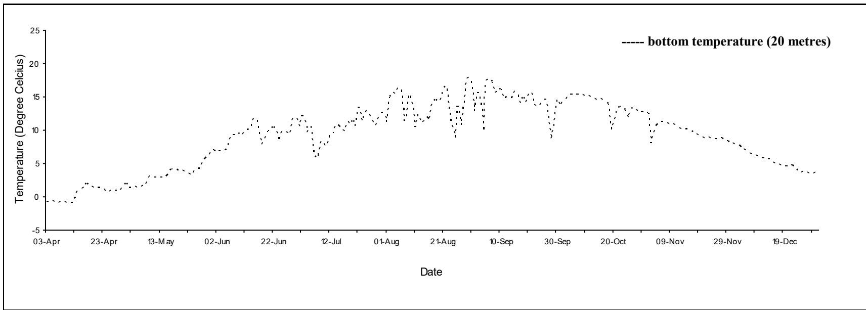
Daily mean temperature for Souris, P.E.I., 2021.
