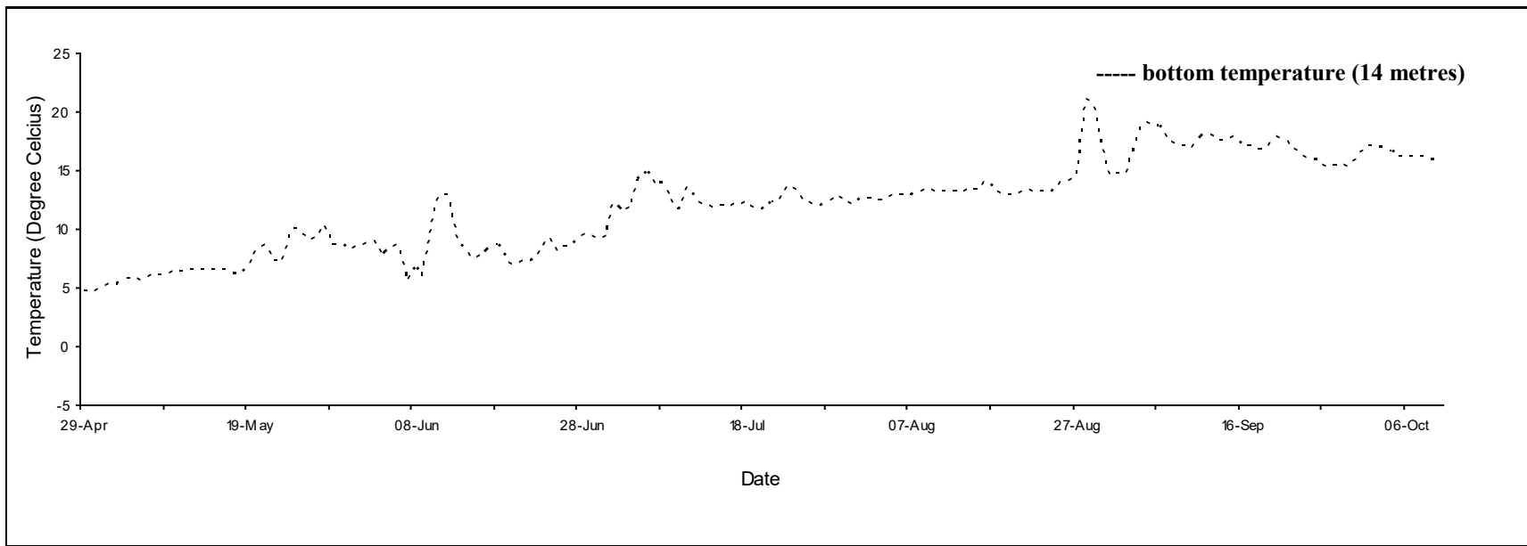
Daily mean temperature for Wallace 1, N.S., 2021.
