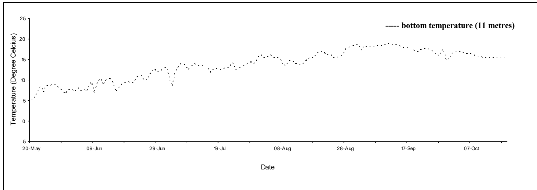
Daily mean temperature for Arisaig, N.S., 2021.
