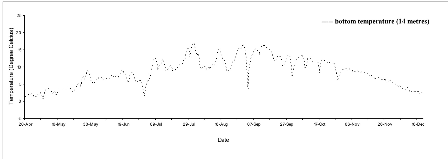
Daily mean temperature for Miscou, N.B., 2021.
