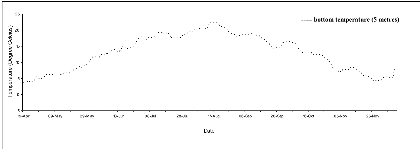
Daily mean temperature for Shediac, N.B., 2020.
