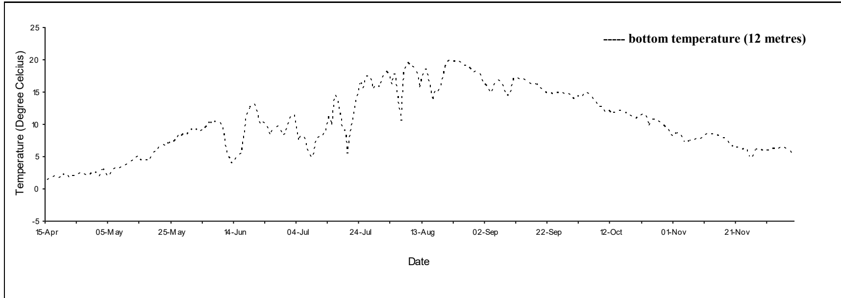
Daily mean temperature for Covehead 2, P.E.I., 2020.
