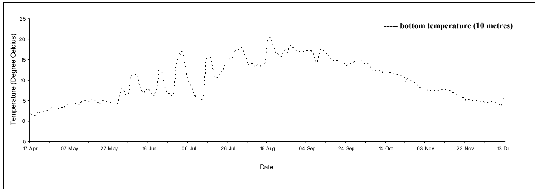
Daily mean temperature for Richibucto, N.B., 2020.
