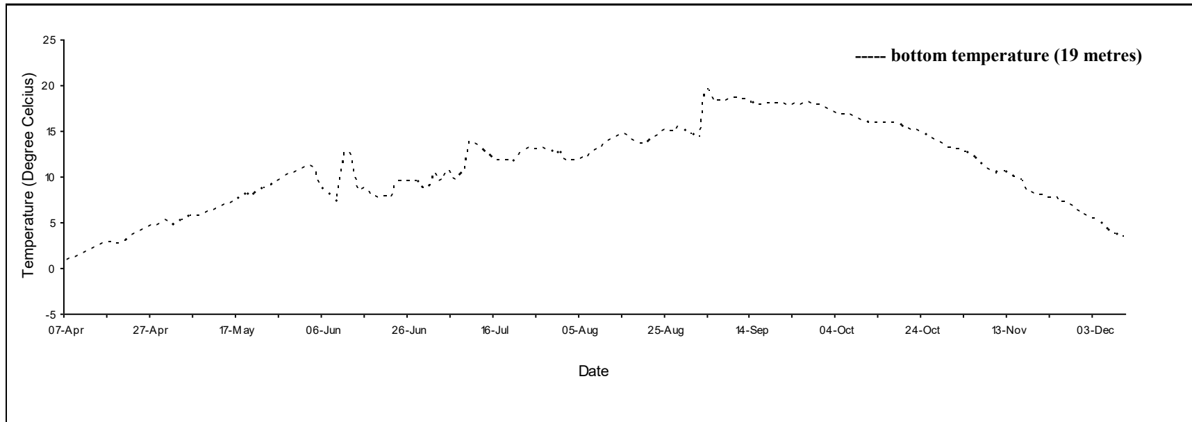
Daily mean temperature for Strait Crossing 2, 2021.
