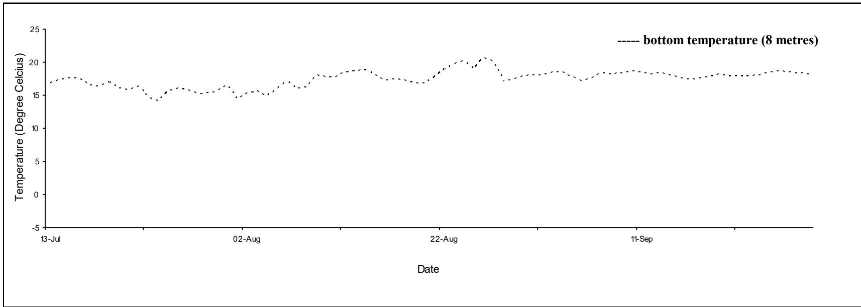
Daily mean temperature for Nine Mile Creek, P.E.I., 2021.
