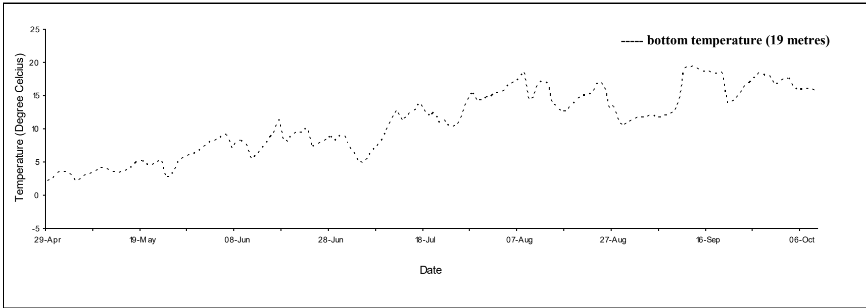
Daily mean temperature for Port Hood, N.S., 2021.
