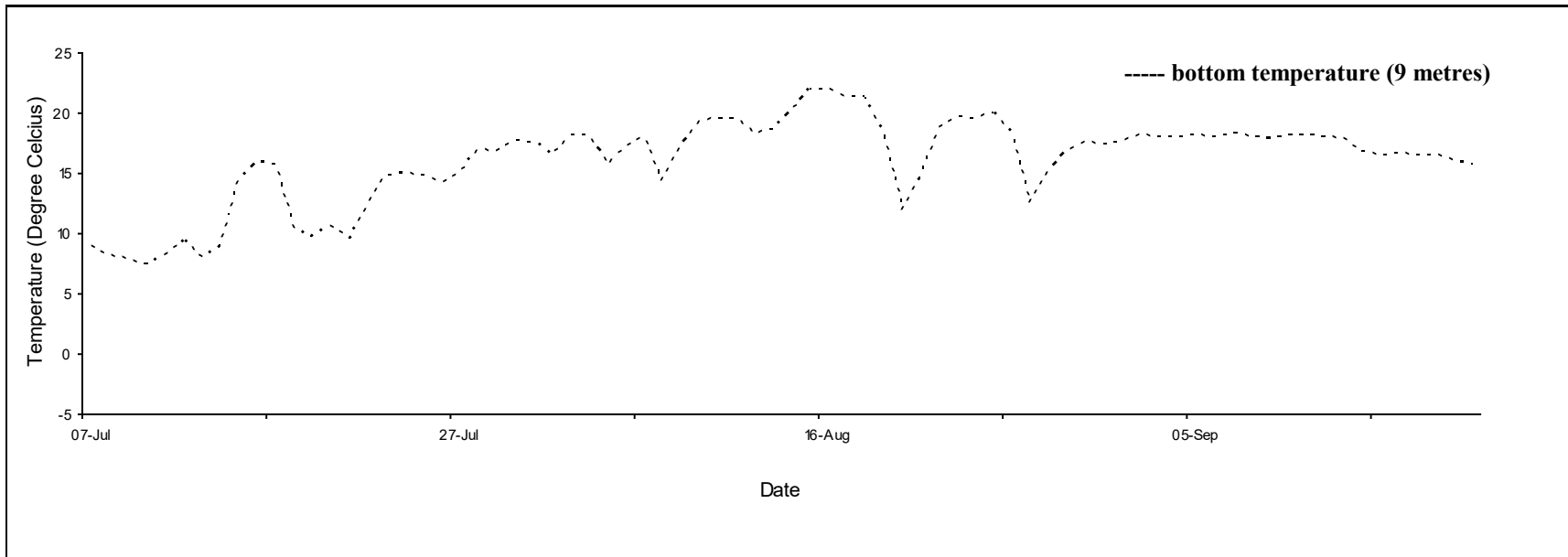
Daily mean temperature for Fortune 1, P.E.I., 2020.
