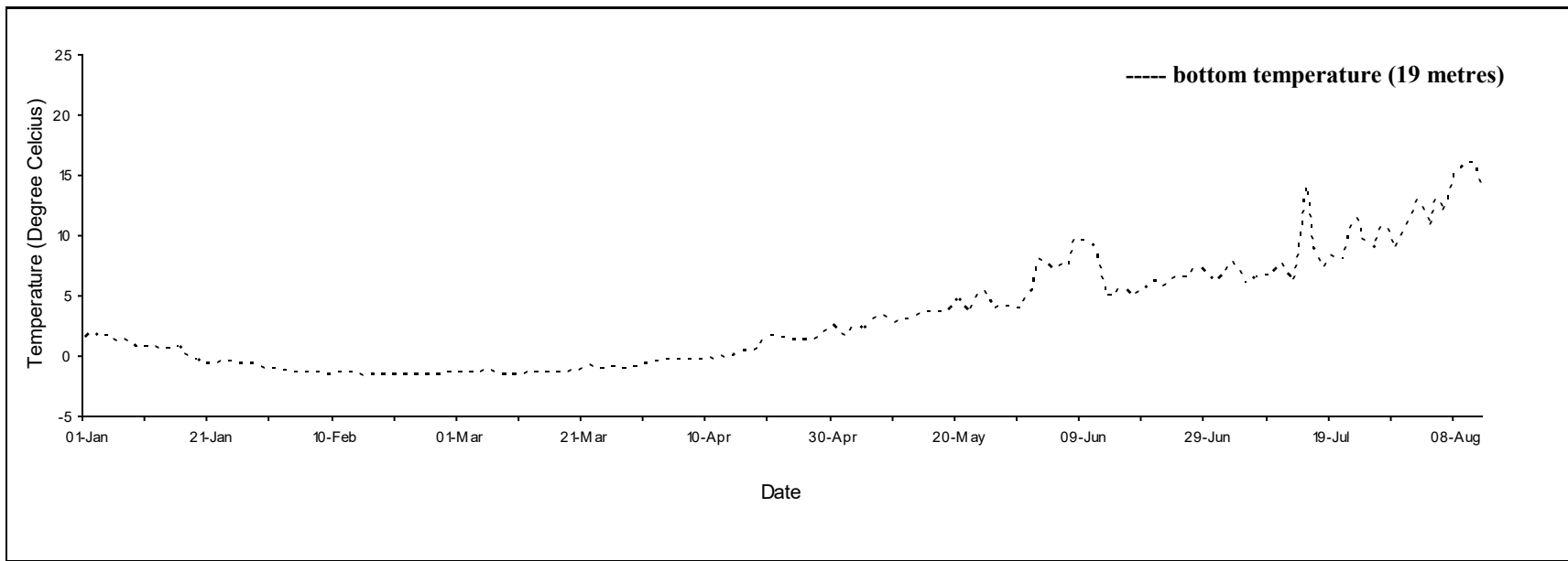
Daily mean temperature for Bayfield, N.S., 2020.
