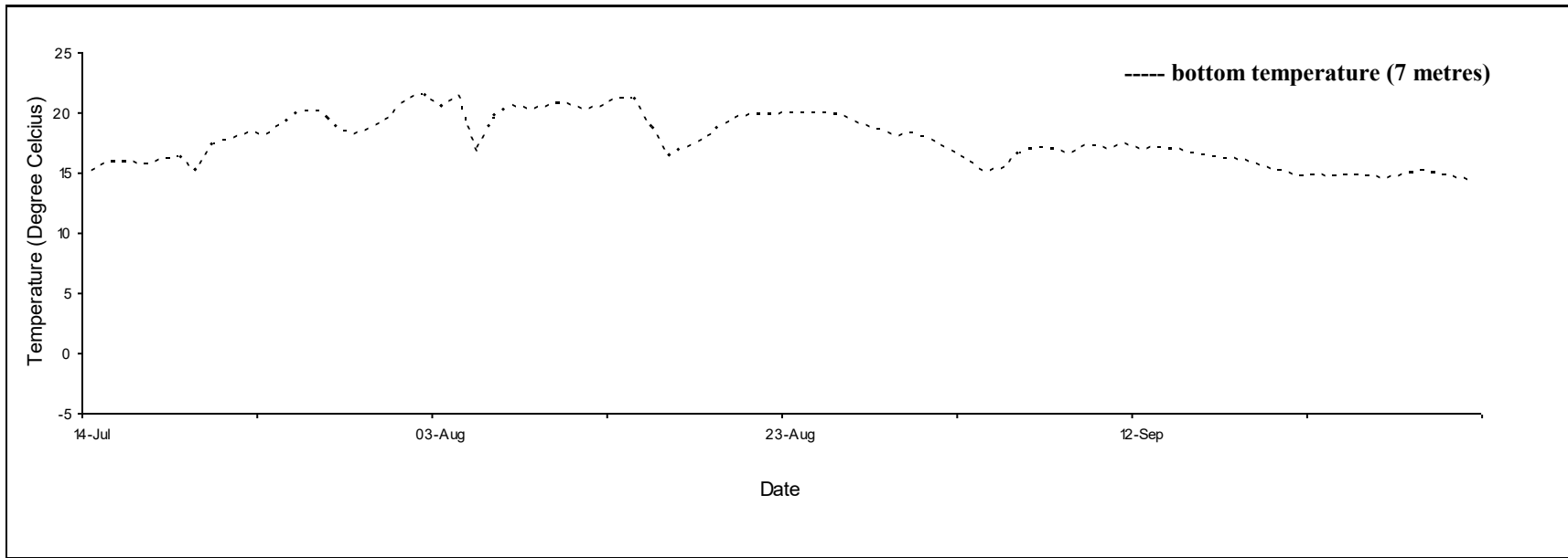
Daily mean temperature for Covehead 1, P.E.I., 2020.
