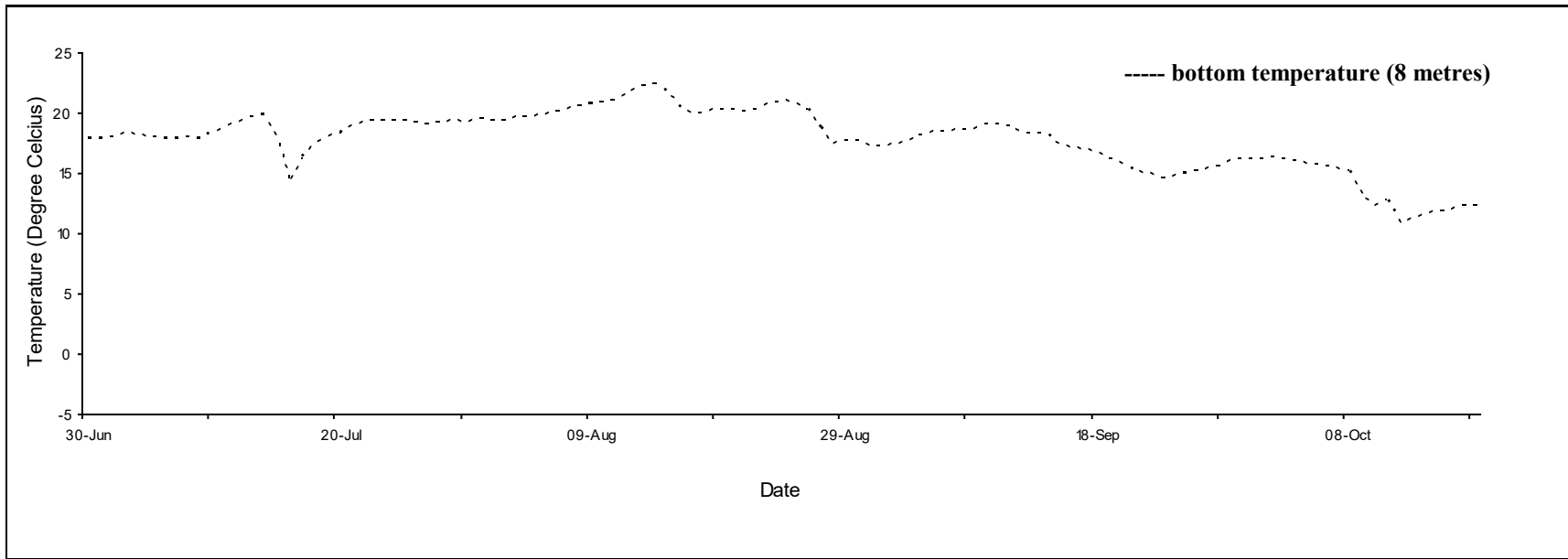
Daily mean temperature for Egmont Bay, P.E.I., 2020.
