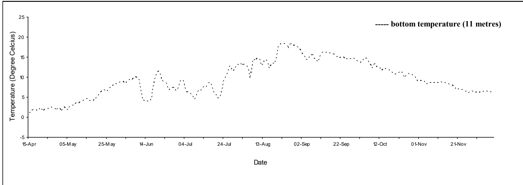
Daily mean temperature for North Tracadie, P.E.I., 2020.
