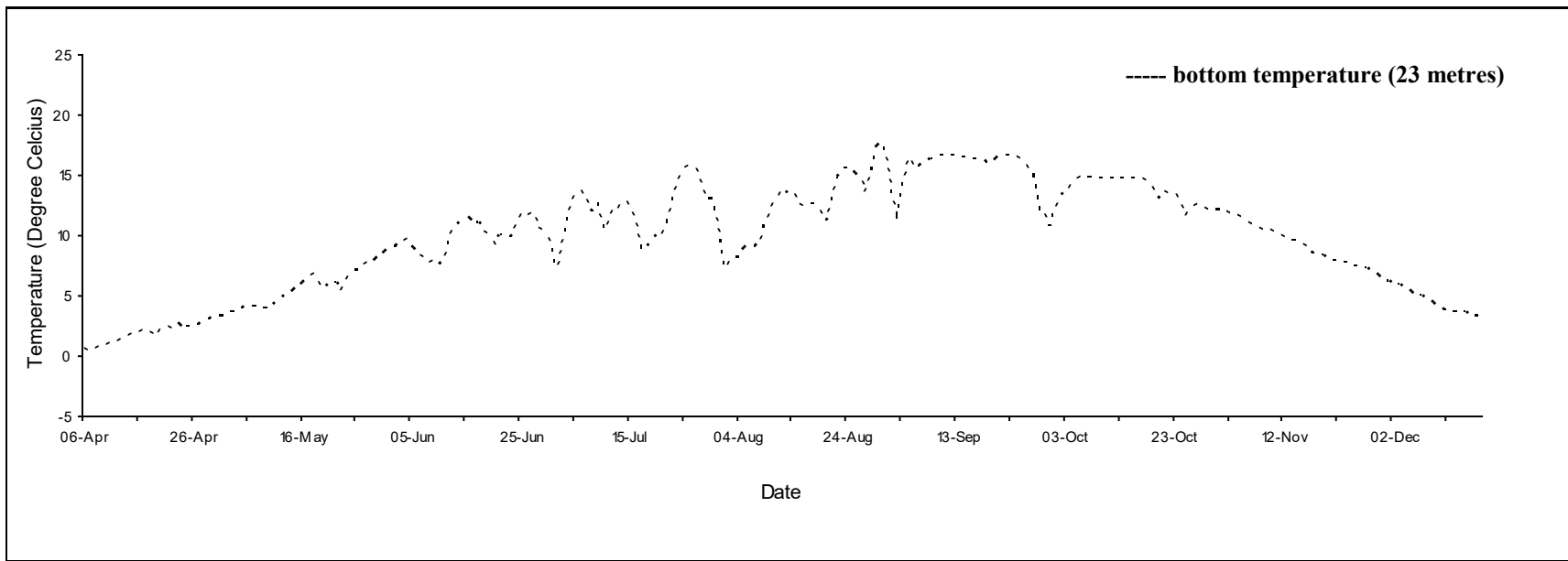
Daily mean temperature for West Point, P.E.I., 2021.
