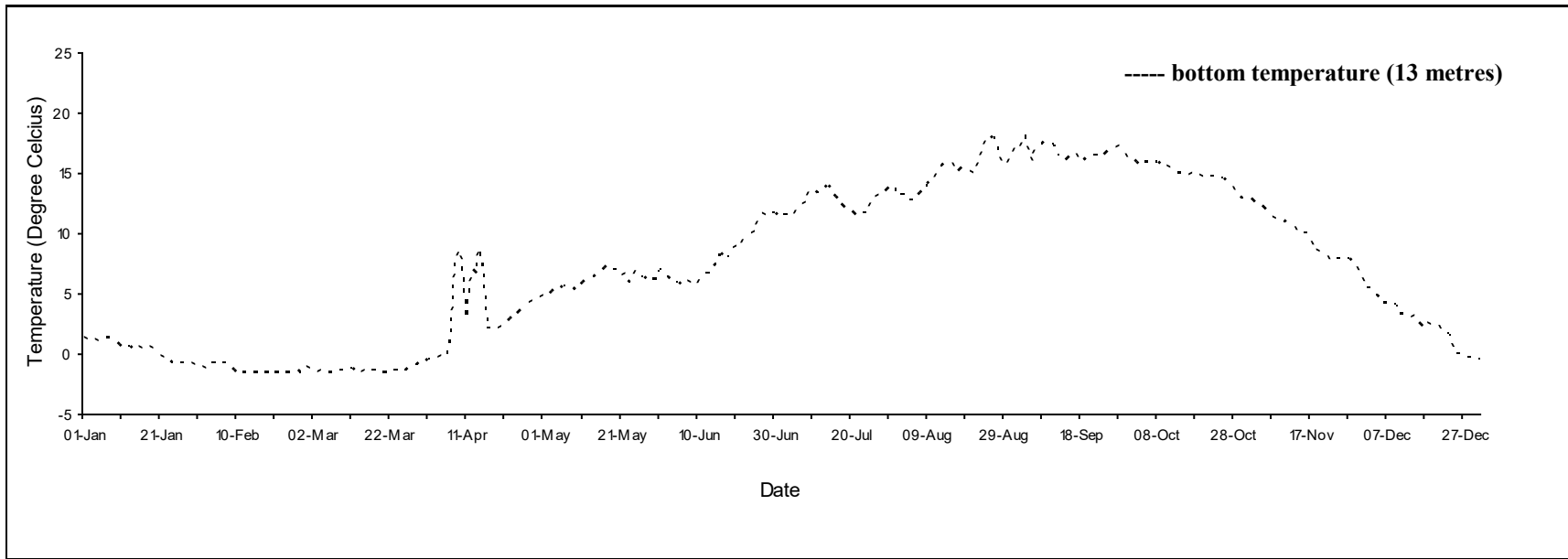
Daily mean temperature for Prim Reef, P.E.I., 2021.
