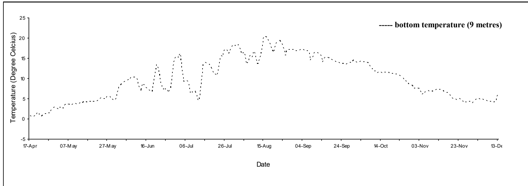
Daily mean temperature for Pointe Sapin, N.B., 2020.
