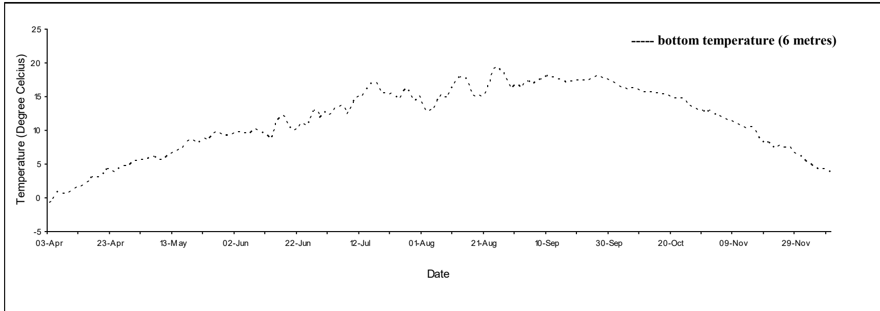
Daily mean temperature for Victoria, P.E.I., 2021.
