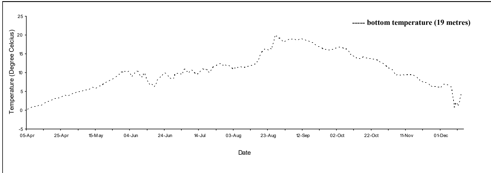
Daily mean temperature for Strait Crossing 2, 2020.
