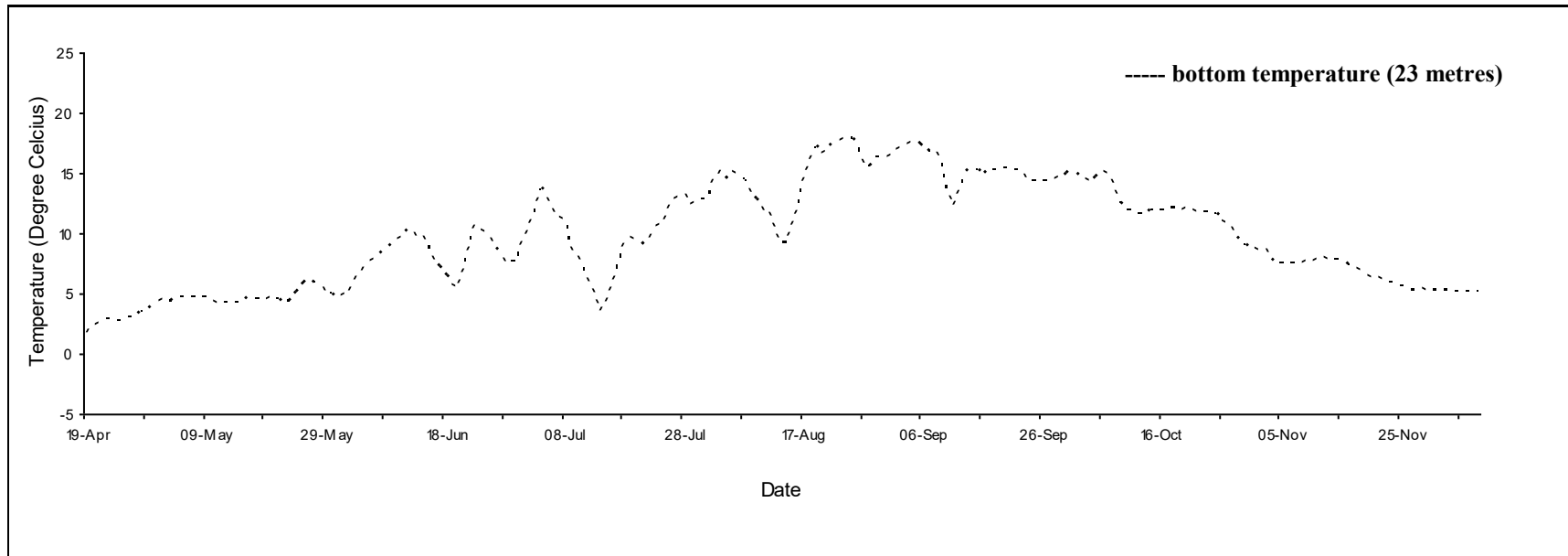
Daily mean temperature for West Point, P.E.I., 2020.
