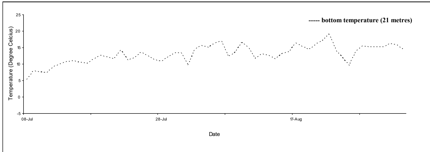
Daily mean temperature for Fortune 2, P.E.I., 2021.
