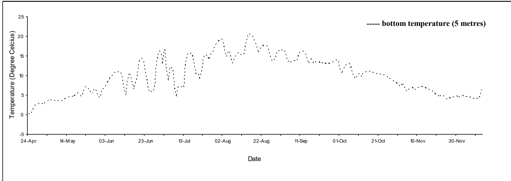
Daily mean temperature for Tabusintac, N.B., 2020.
