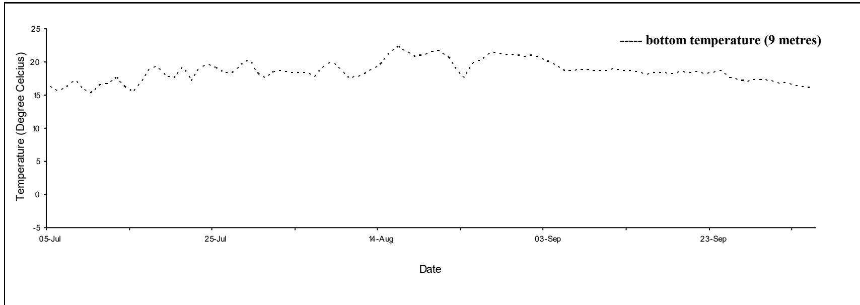
Daily mean temperature for Wallace 2, N.S., 2021.
