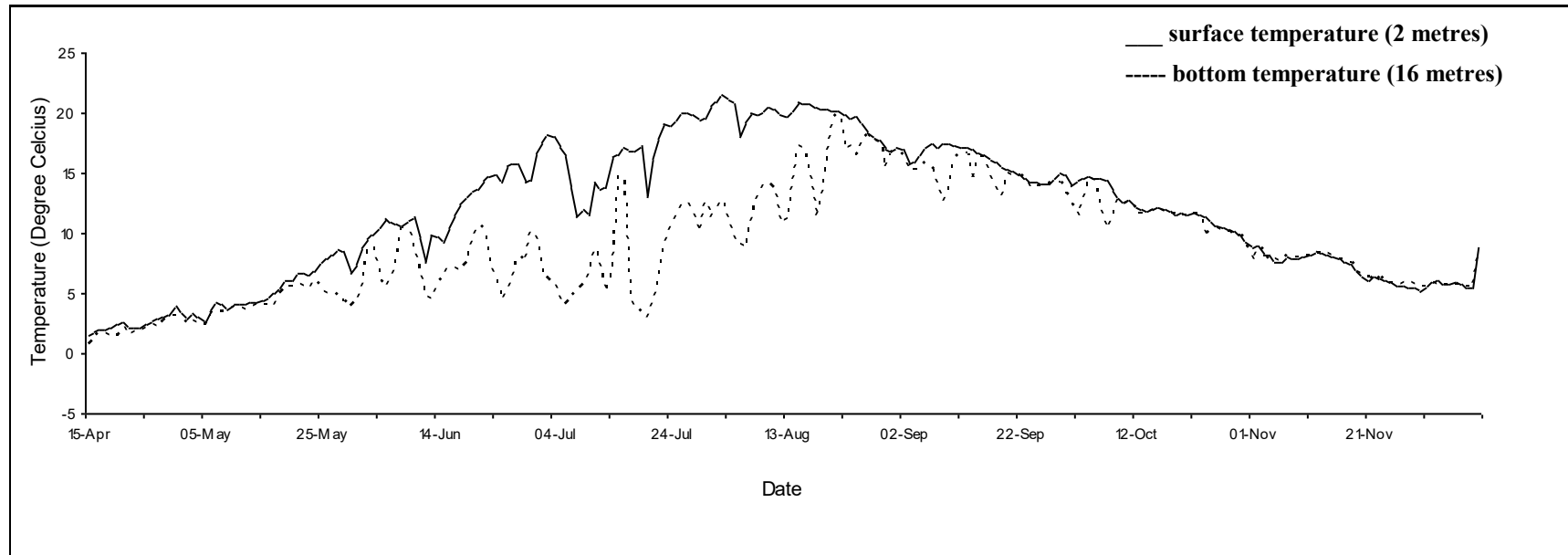
Daily mean temperature for Malpeque, P.E.I., 2020.
