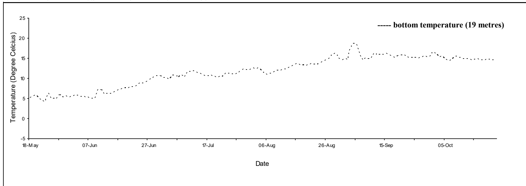
Daily mean temperature for River John, N.S., 2021.
