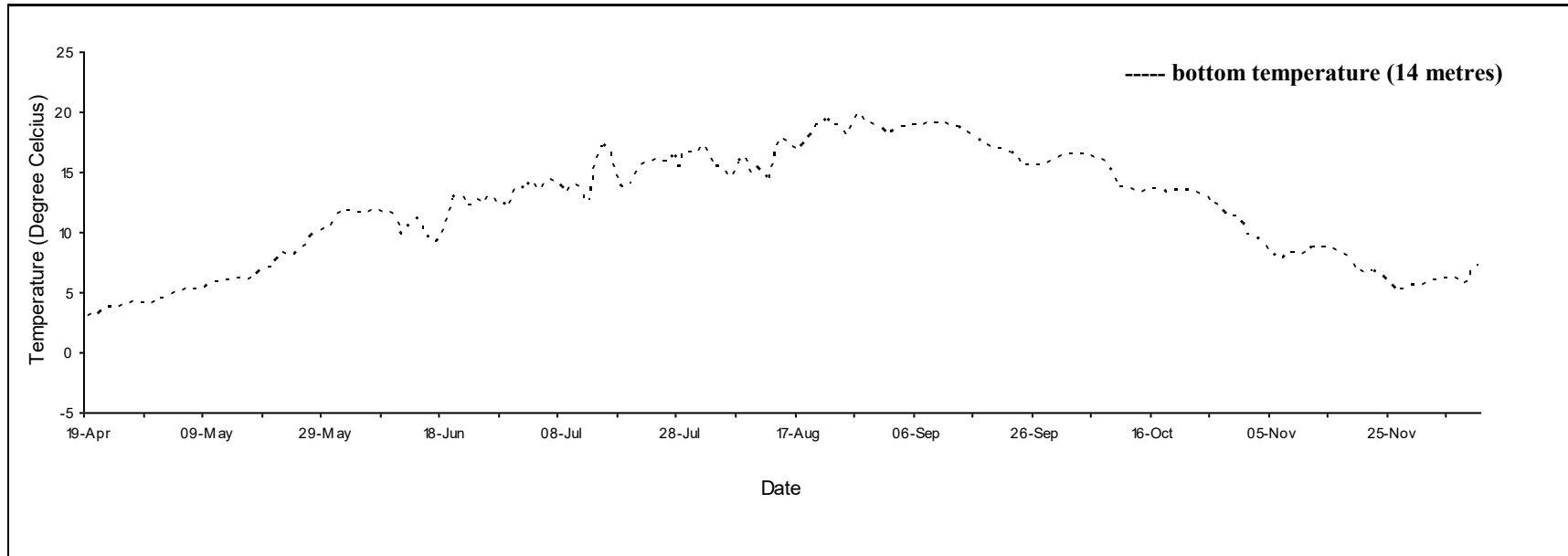
Daily mean temperature for Cape Tormentine, N.B., 2020.
