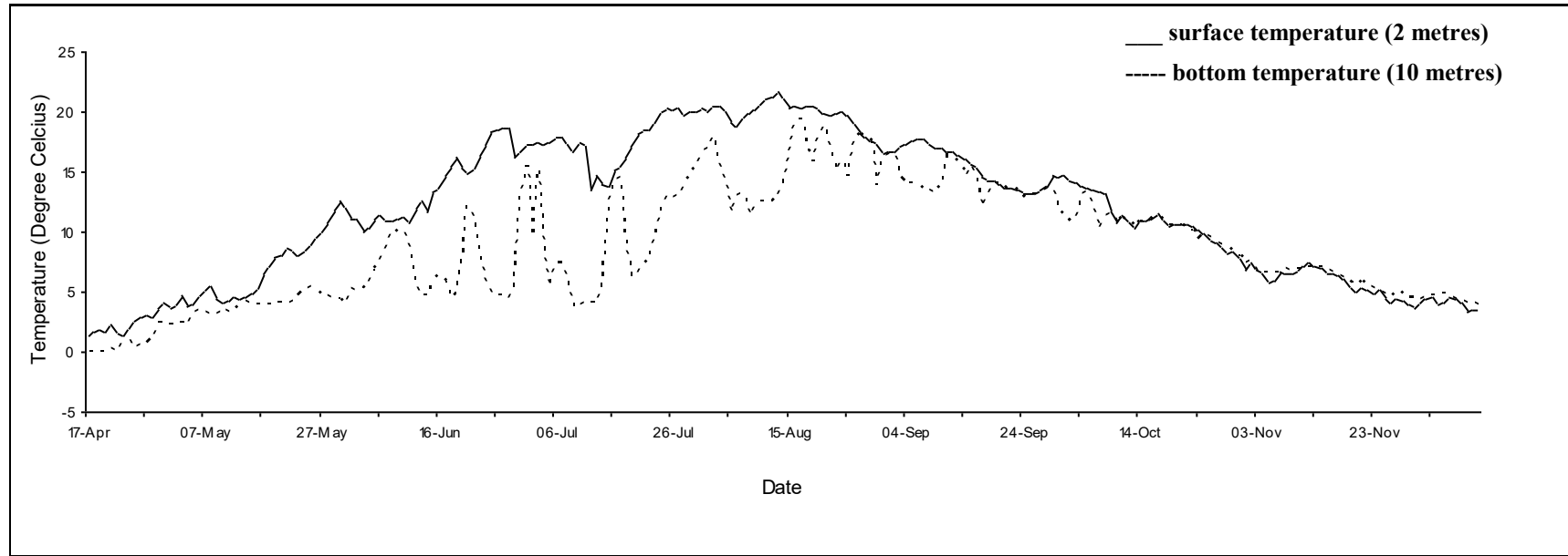
Daily mean temperature for Escuminac, N.B., 2020.
