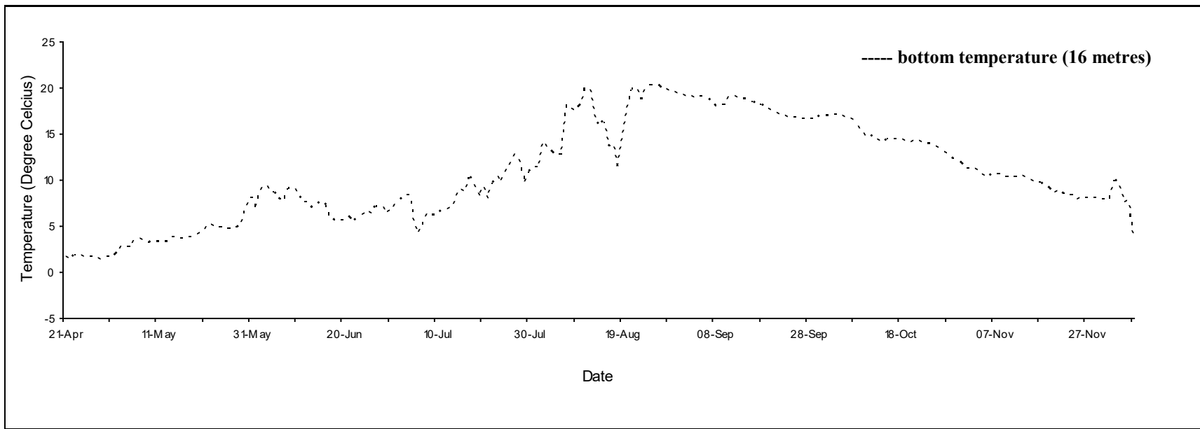
Daily mean temperature for Jack Shoal, N.S., 2020.
