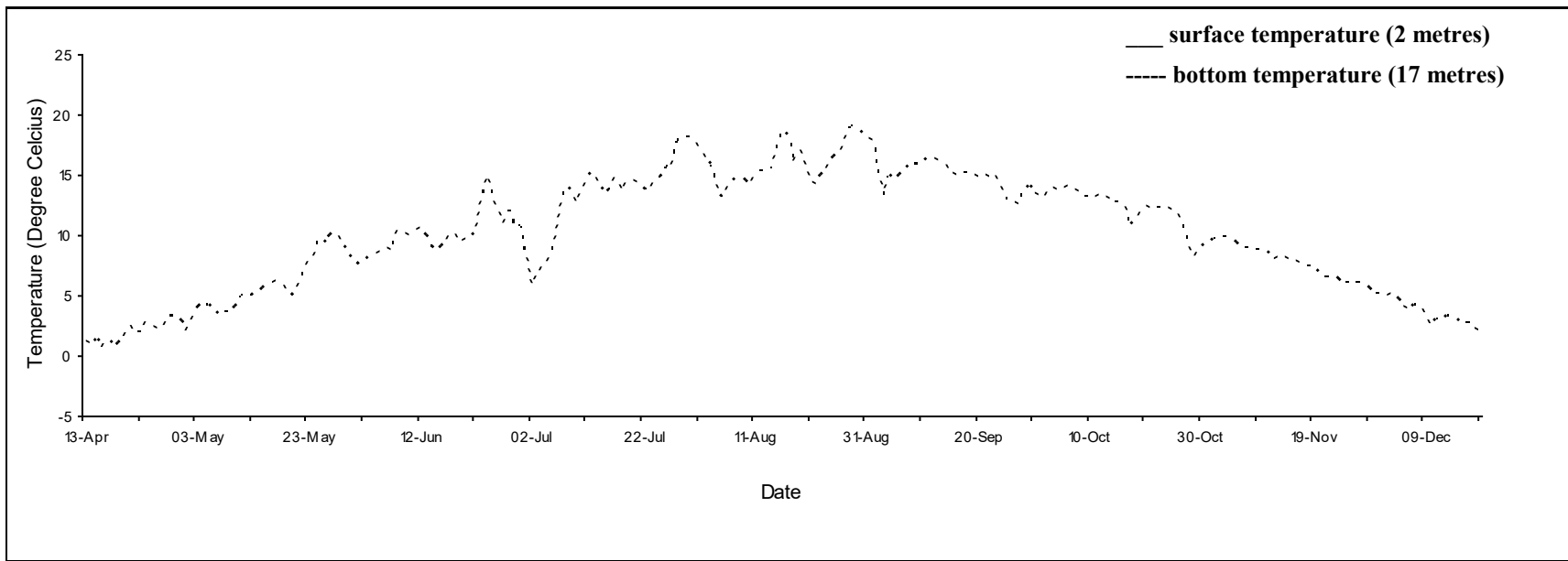
Daily mean temperature for Shippagan, N.B., 2021.
