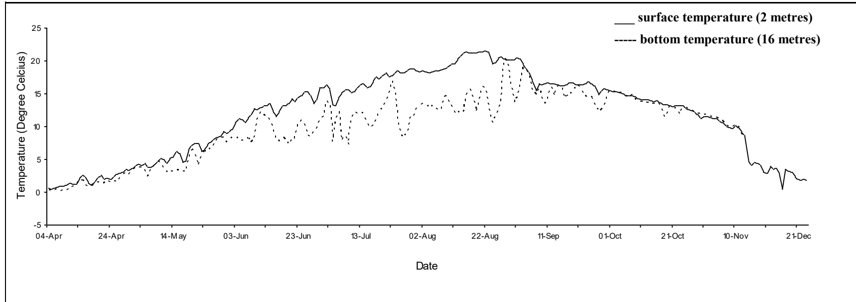
Daily mean temperature for Malpeque, P.E.I., 2021.
