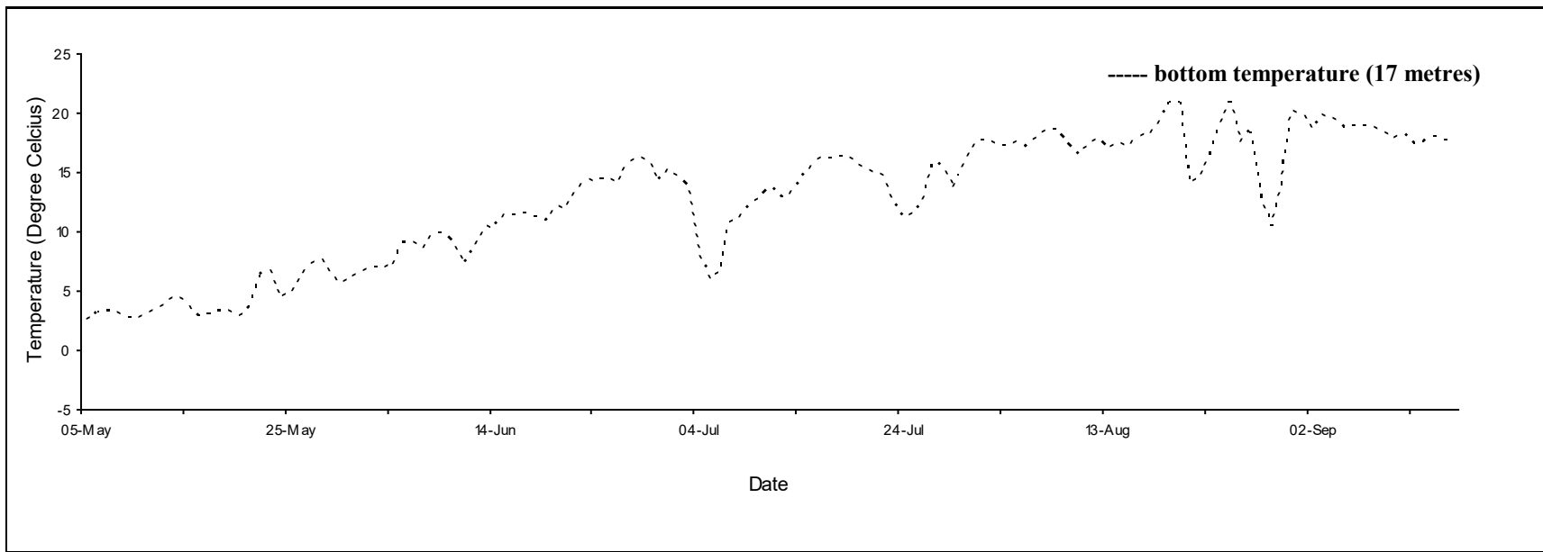
Daily mean temperature for Cheticamp, N.S., 2021.
