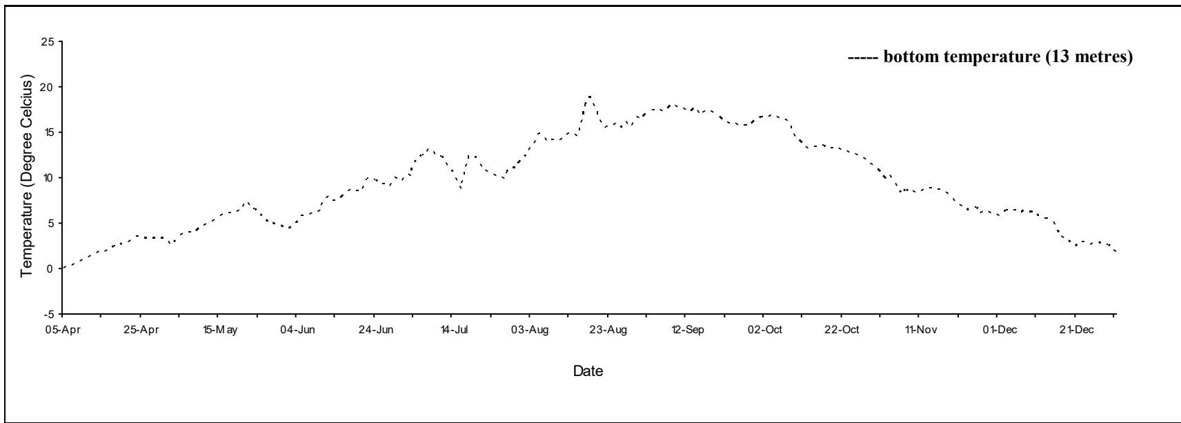
Daily mean temperature for Prim Reef, P.E.I., 2020.
