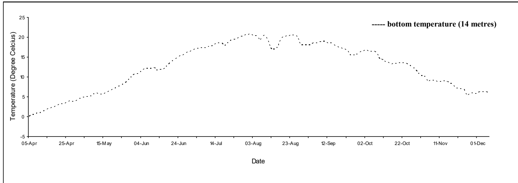
Daily mean temperature for Strait Crossing 1, 2020.
