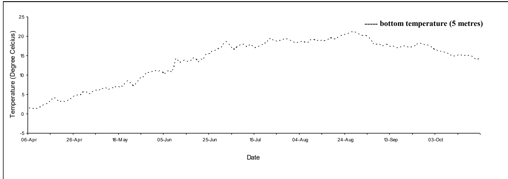
Daily mean temperature for Shediac, N.B., 2021.
