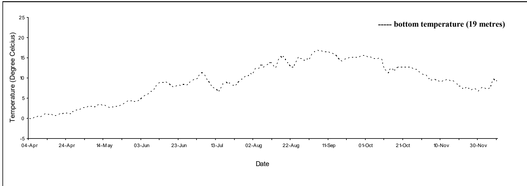
Daily mean temperature for Indian Rocks, P.E.I., 2020.
