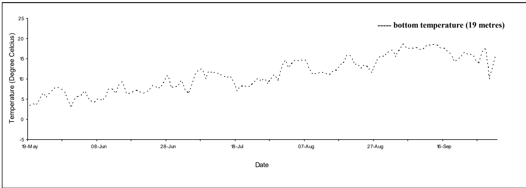
Daily mean temperature for Ballantynes, N.S., 2021.
