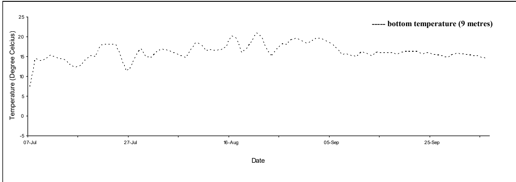
Daily mean temperature for Alberton, P.E.I., 2021.
