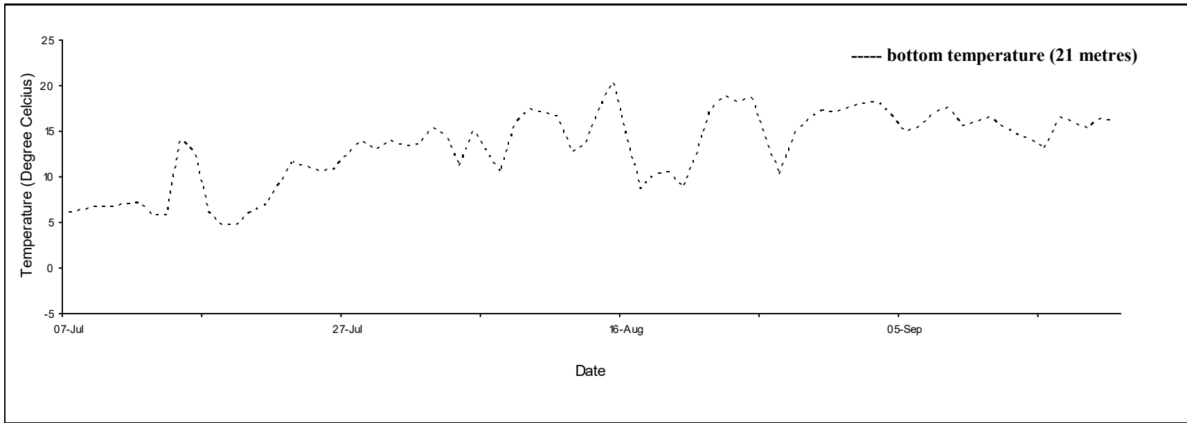
Daily mean temperature for Fortune 2, P.E.I., 2020.
