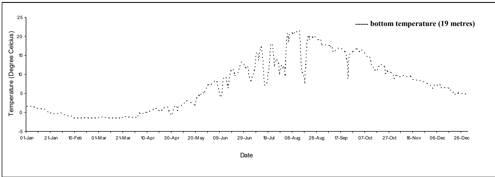
Daily mean temperature for Pleasant Bay 1, N.S., 2020.
