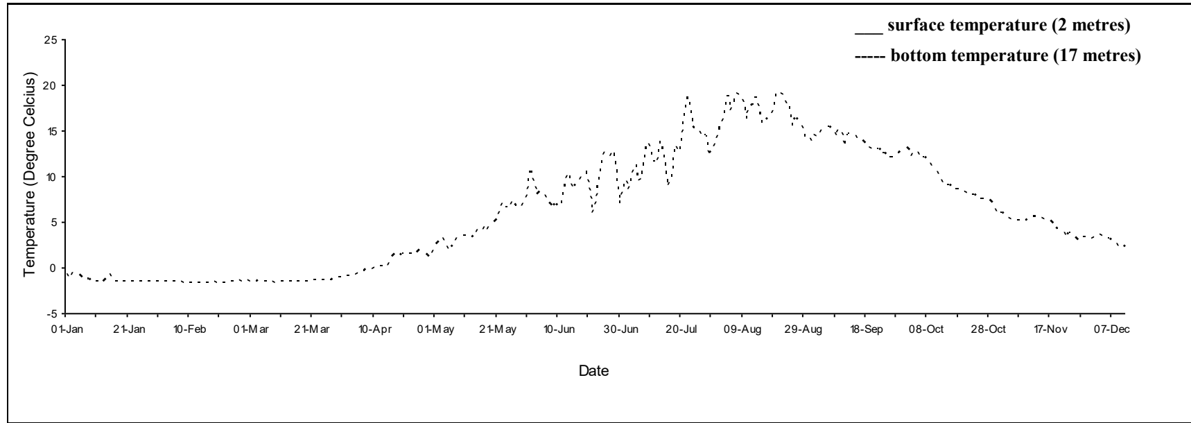
Daily mean temperature for Shippagan, N.B., 2020.
