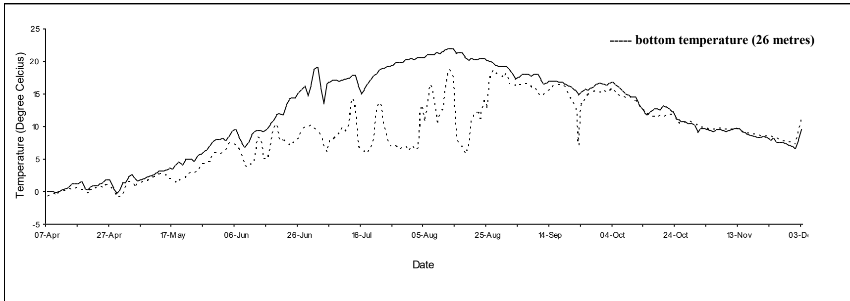
Daily mean temperature for Pleasant Bay 2, N.S., 2020.
