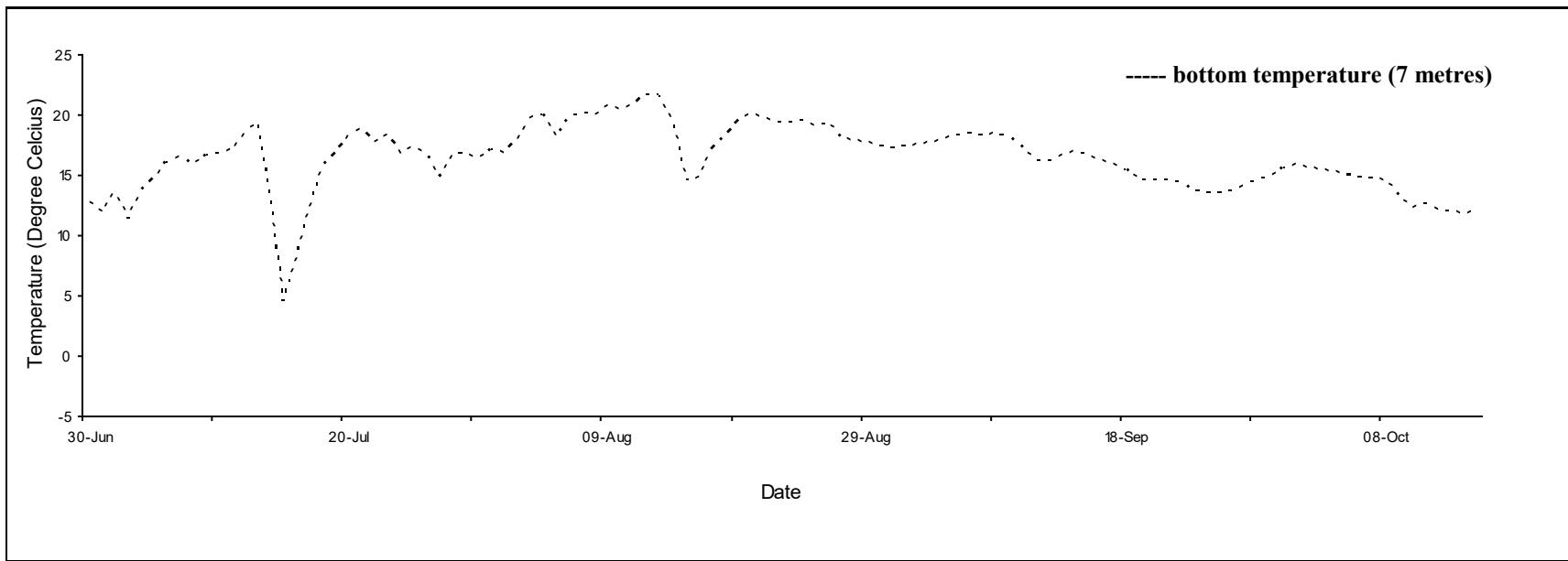
Daily mean temperature for Skidders Pond, P.E.I., 2020.
