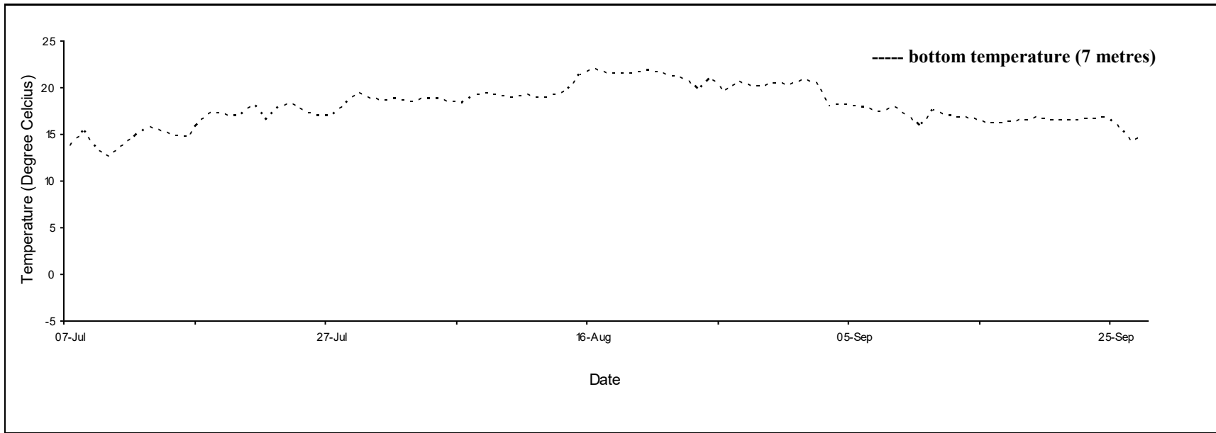
Daily mean temperature for Covehead 1, P.E.I., 2021.
