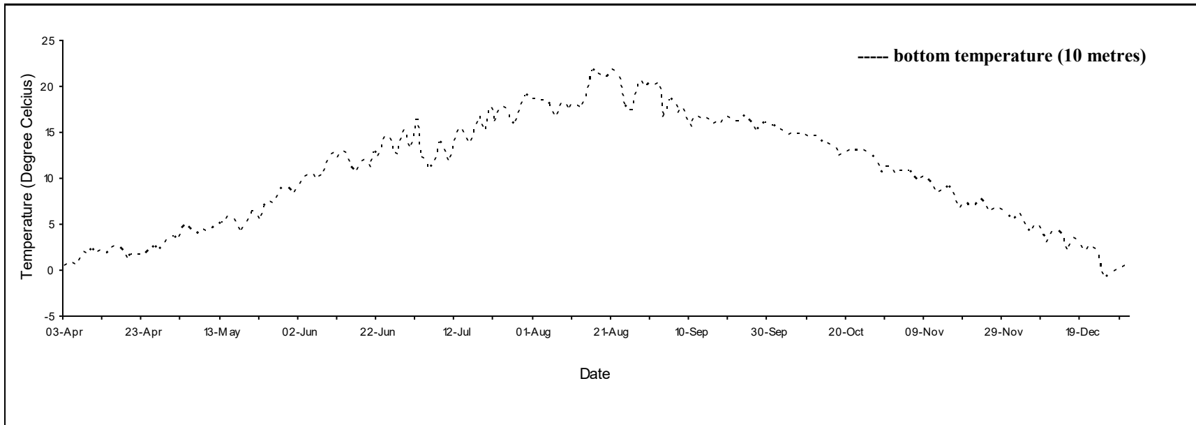
Daily mean temperature for Rustico, P.E.I., 2021.
