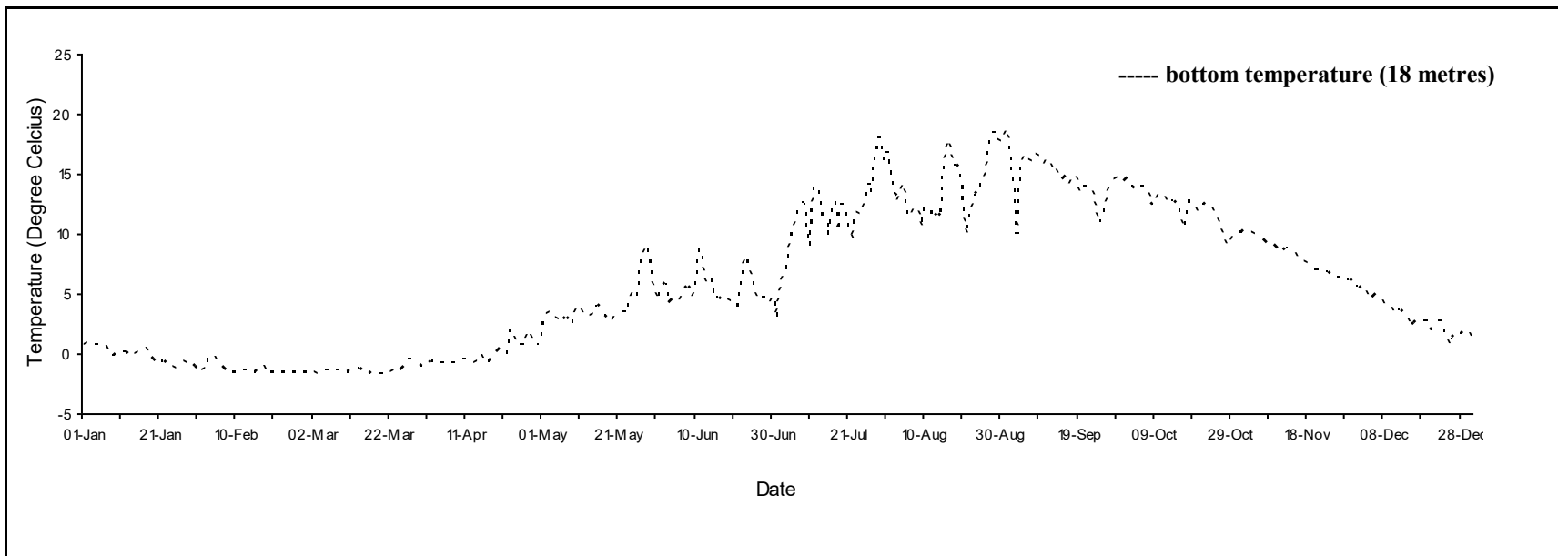
Daily mean temperature for Anse Bleue 2, N.B., 2021.
