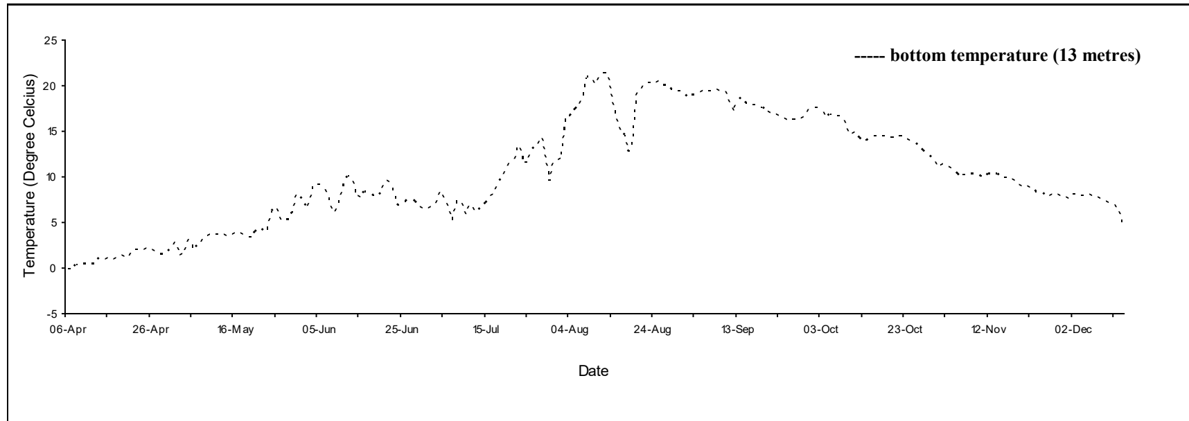
Daily mean temperature for Judique Shoals, N.S., 2020.
