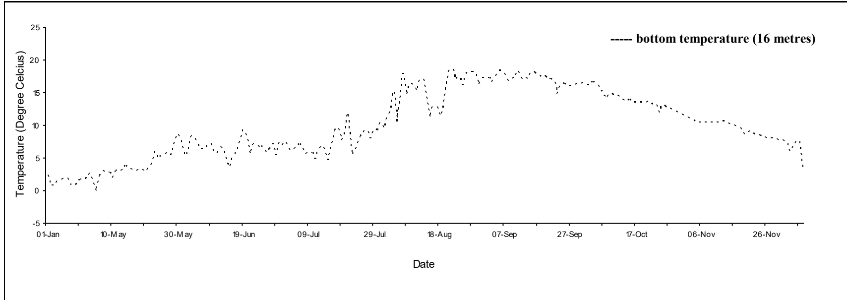
Daily mean temperature for Cape George, N.S., 2020.
