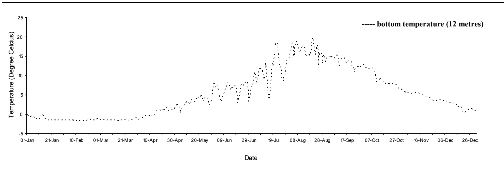
Daily mean temperature for Anse Bleue 1, N.B., 2020.
