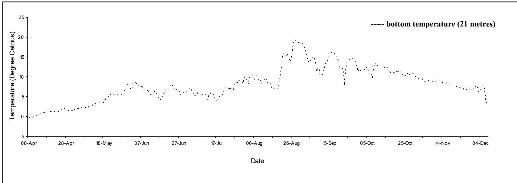
Daily mean temperature for East Point reef, P.E.I., 2020.
