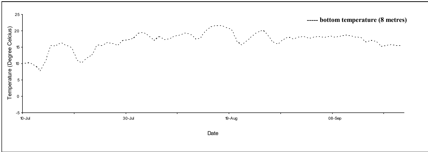
Daily mean temperature for Murray Harbour, P.E.I., 2020.
