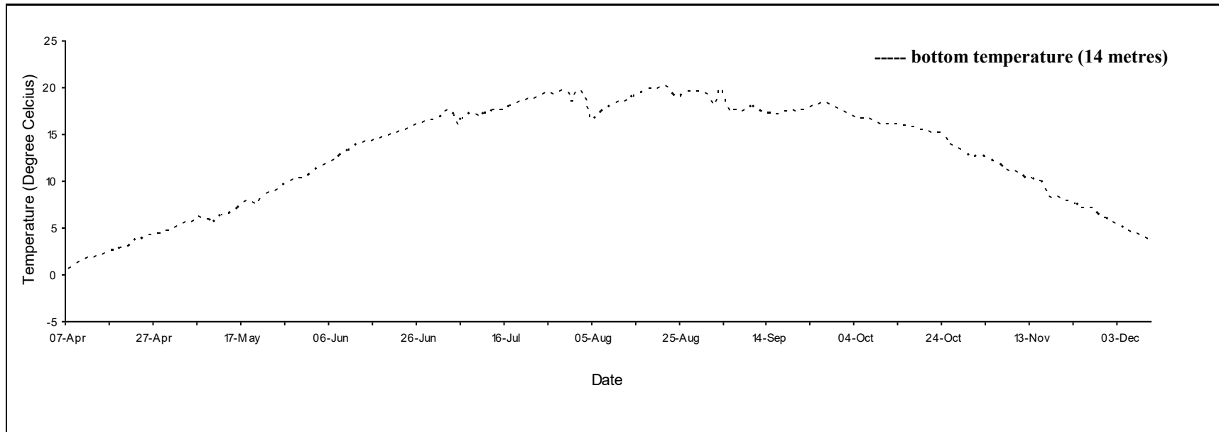
Daily mean temperature for Strait Crossing 1, 2021.
