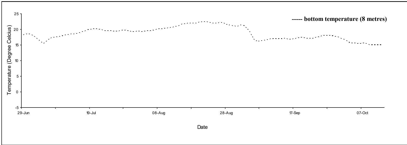
Daily mean temperature for Egmont Bay, P.E.I., 2021.
