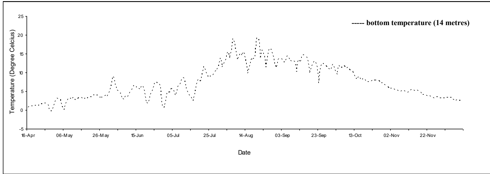
Daily mean temperature for Miscou, N.B., 2020.
