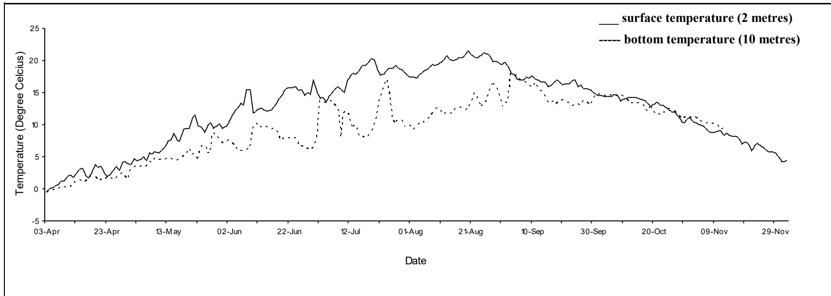
Daily mean temperature for Escuminac, N.B., 2021.
