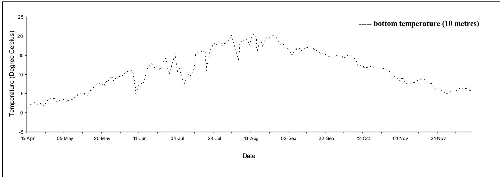
Daily mean temperature for Rustico, P.E.I., 2020.
