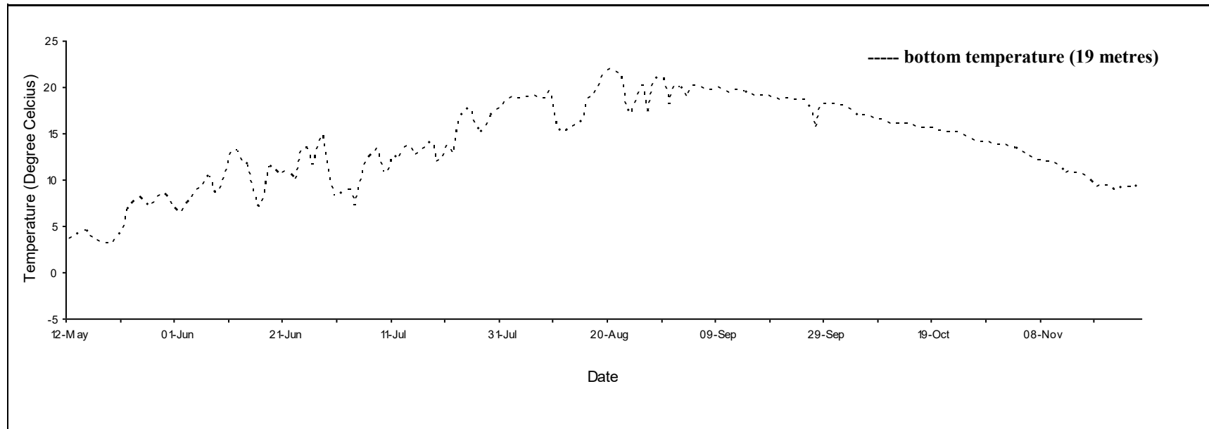
Daily mean temperature for Aulds Cove, N.S., 2021.
