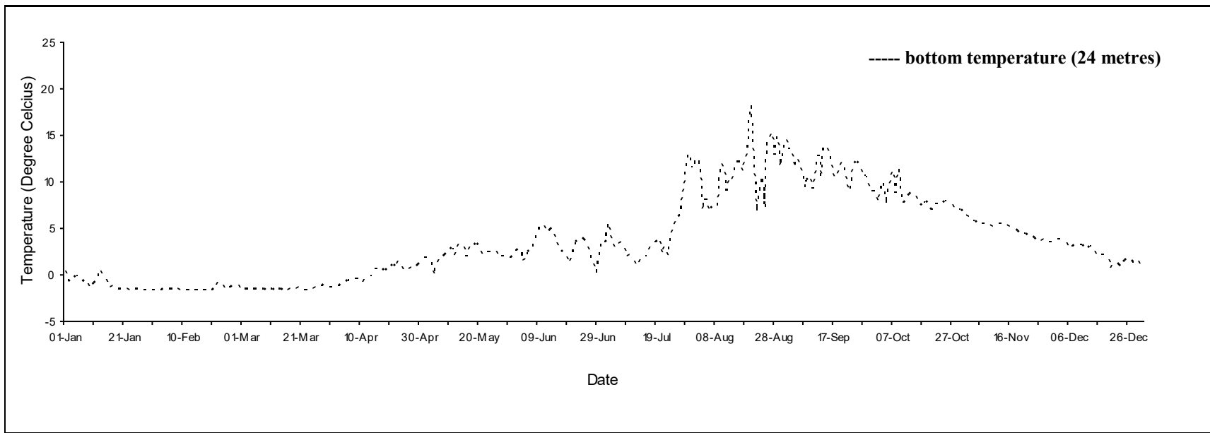
Daily mean temperature for Anse Bleue 3, N.B., 2020.
