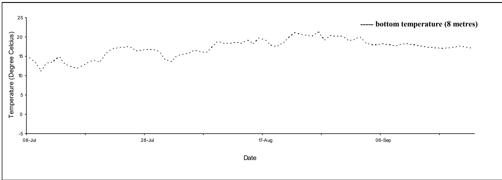
Daily mean temperature for Murray Harbour, P.E.I., 2021.
