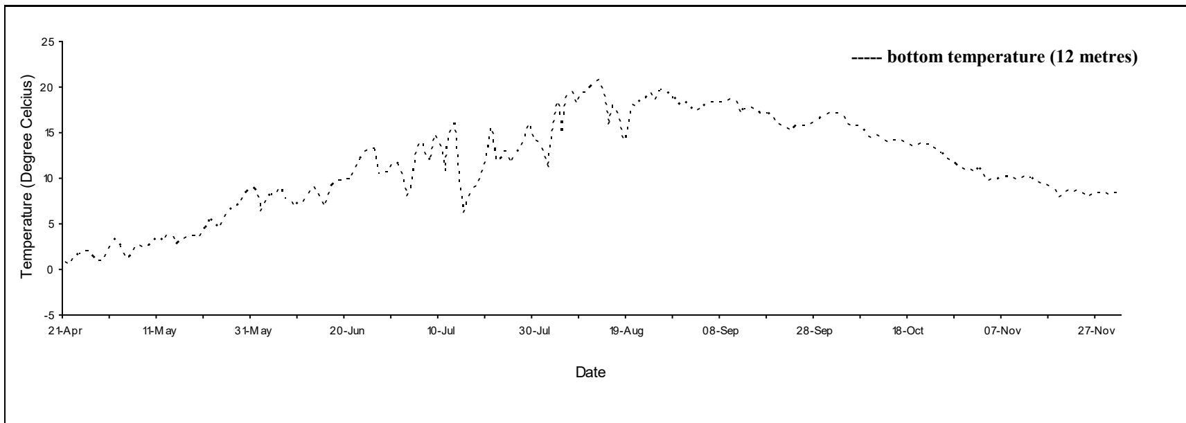
Daily mean temperature for Mabou Harbour, N.S., 2020.
