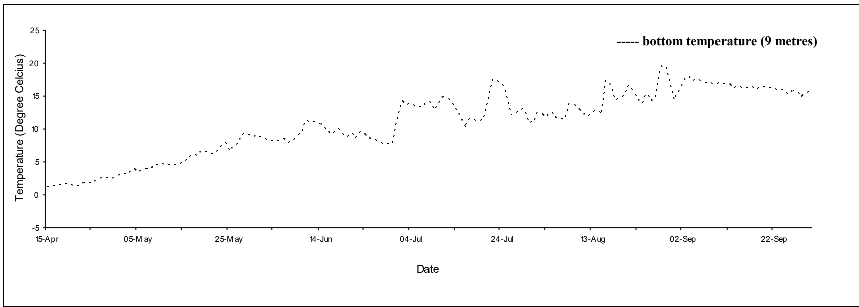
Daily mean temperature for Pointe Sapin, N.B., 2021.
