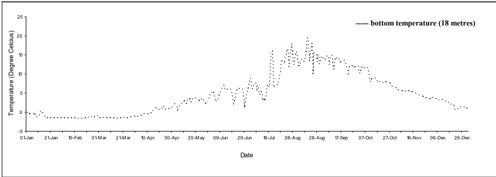
Daily mean temperature for Anse Bleue 2, N.B., 2020.
