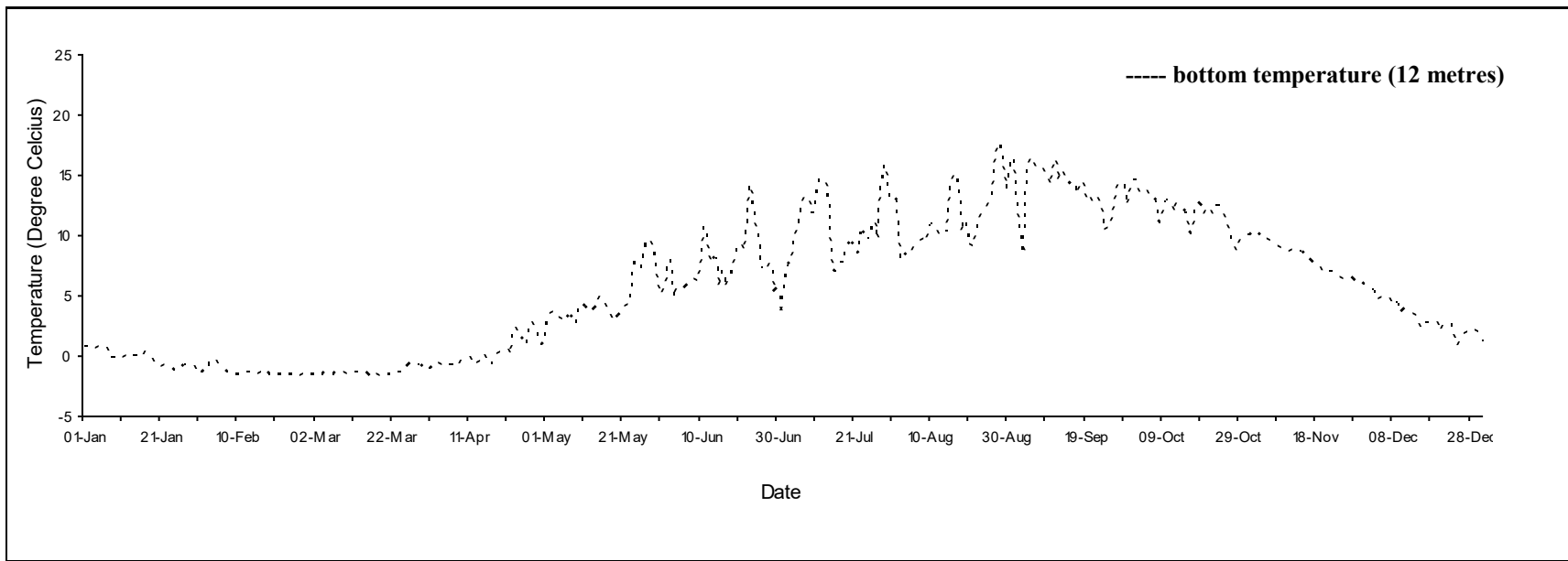
Daily mean temperature for Anse Bleue 1, N.B., 2021.
