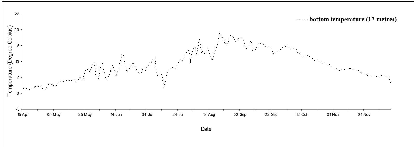
Daily mean temperature for North Cape, P.E.I., 2020.
