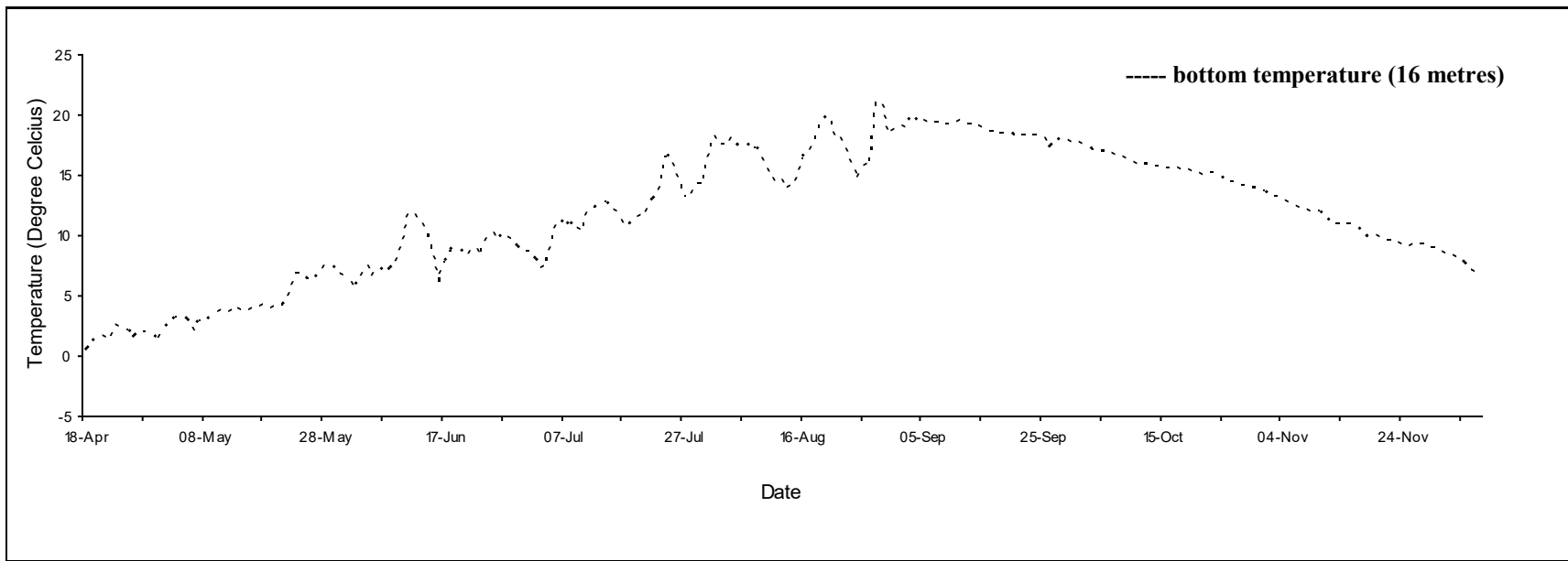
Daily mean temperature for Jack Shoal, N.S., 2021.
