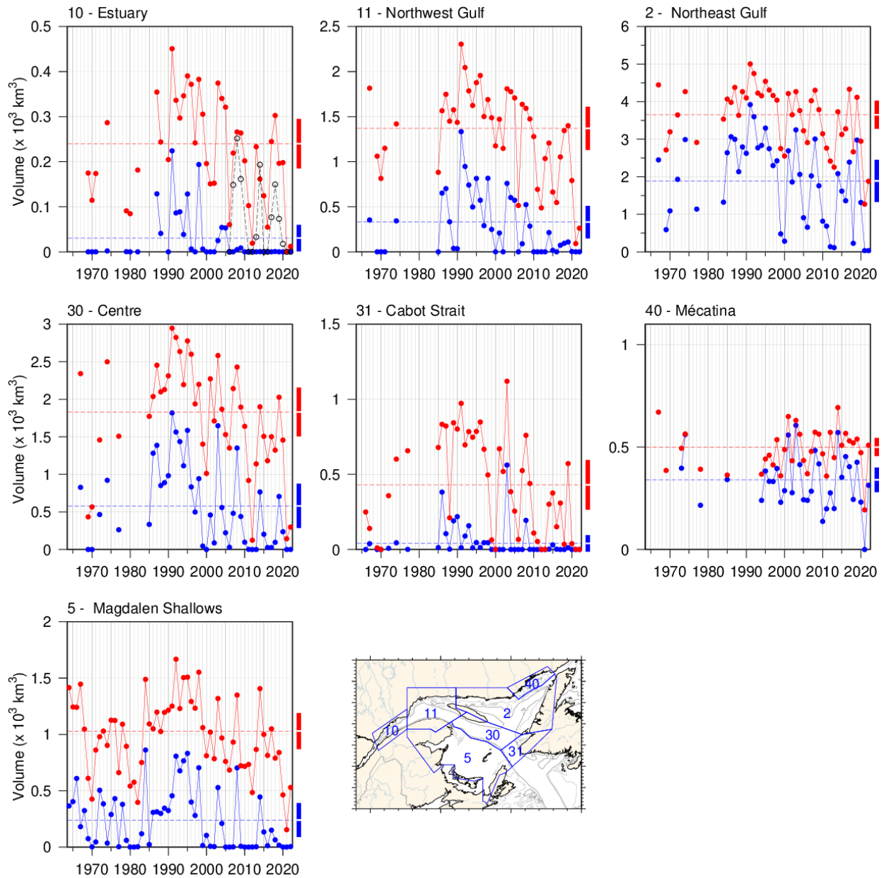
Fig. 38. Volume of the CIL colder than 0^\circ\text{C} (blue) and colder than 1^\circ\text{C} (red) in August and September (Data mostly in September on Magdalen Shallows and August elsewhere). The volume of the CIL colder than 1^\circ\text{C} in November for available years since 2006 is also shown for the St. Lawrence Estuary (black dashed line). Red and blue dashed lines are 1991–2020 averages and rectangles on the right side show the 1991–2020 mean \pm 0.5 SD.
