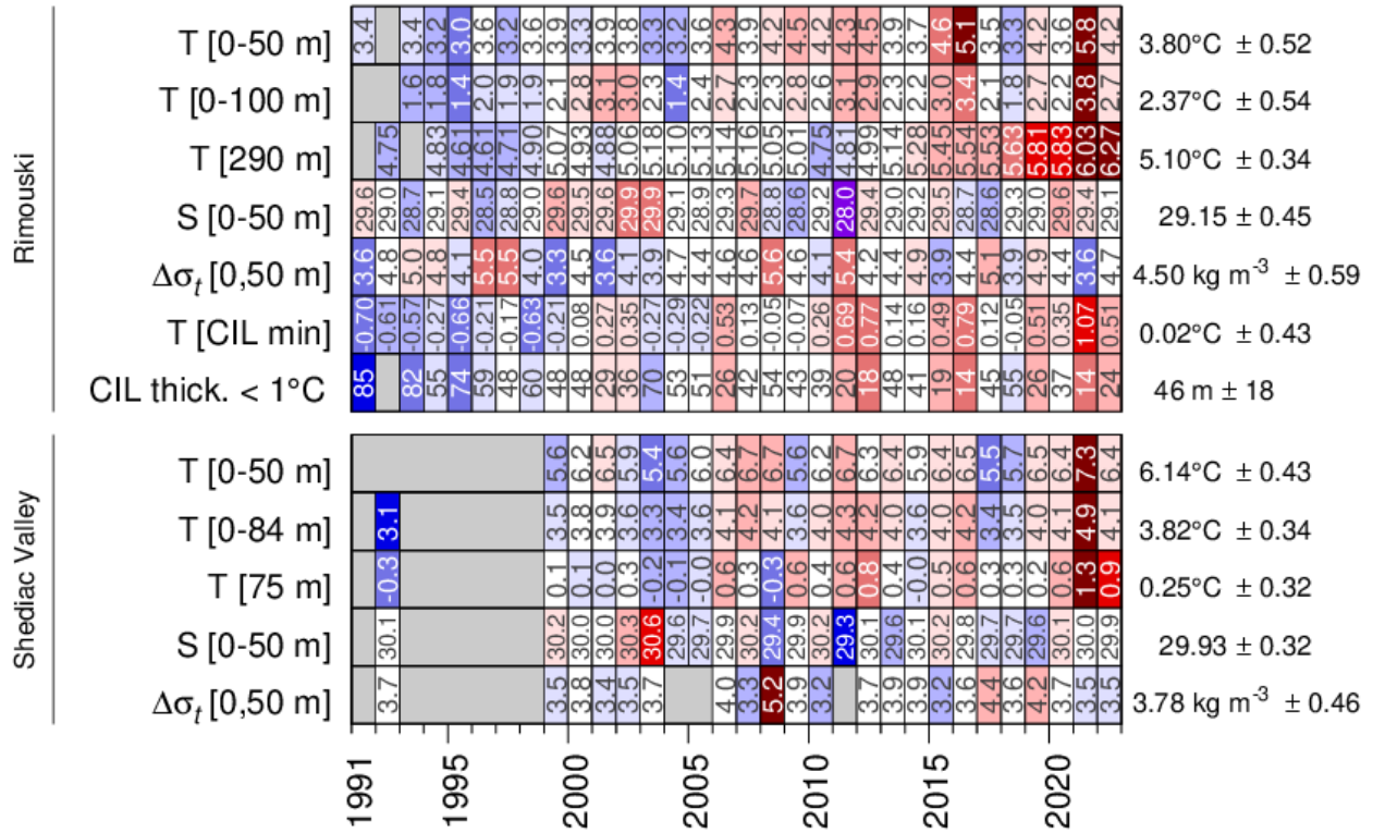
Fig. 66. May to October temperature and salinity layer averages, stratification (expressed as the density difference between 0 m and 50 m), and CIL temperature minimum and thickness ( T < 1^\circ\text{C} ) for high frequency monitoring stations. Numbers in panels are monthly average values colour-coded according to the anomaly relative to the 1991–2020 climatology. Three months of anomaly data, between May and October, are required to show an average anomaly for any given year, except for deep water temperature at Rimouski station. Data in either July or August are also required for stratification at Shediac Valley. Temperatures at 290 m and 75 m at Rimouski station and Shediac Valley station are considered to represent near-bottom temperatures.
