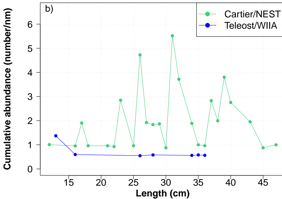
Figure 235. Biplot of Cartier catch versus Teleost catch (upper panel a), and cumulative length frequency distributions (lower panel b) for Ocean pout (species code 640, Zoarces americanus ).
