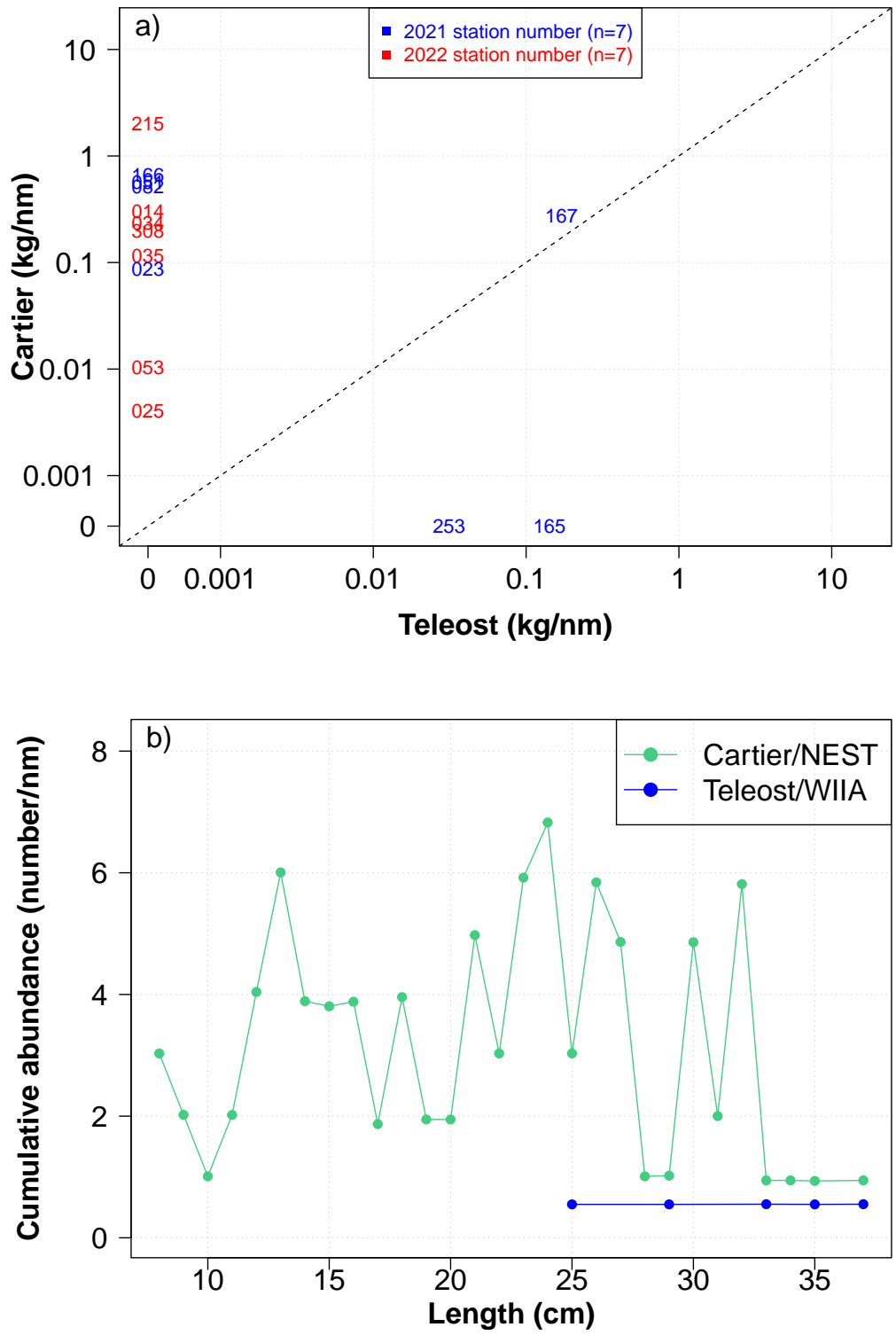
Figure 236. Biplot of Cartier catch versus Teleost catch (upper panel a), and cumulative length frequency distributions (lower panel b) for Vahl's eelpout (species code 647, Lycodes vahlii ).
