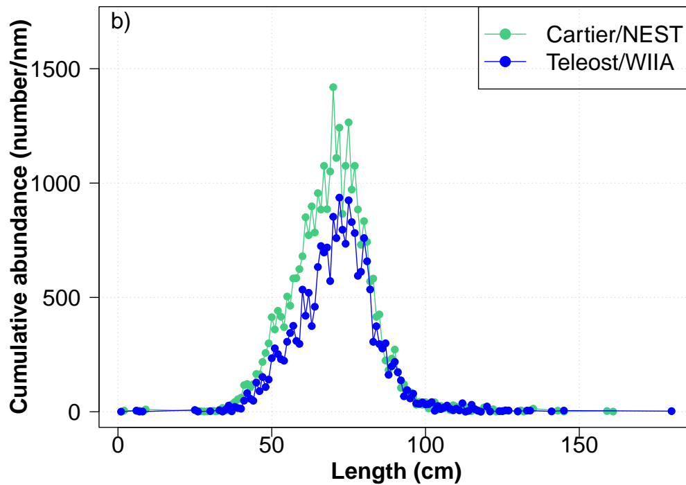
Figure 242. Biplot of Cartier catch versus Teleost catch (upper panel a), and cumulative length frequency distributions (lower panel b) for American lobster (species code 2550, Homarus americanus ).
