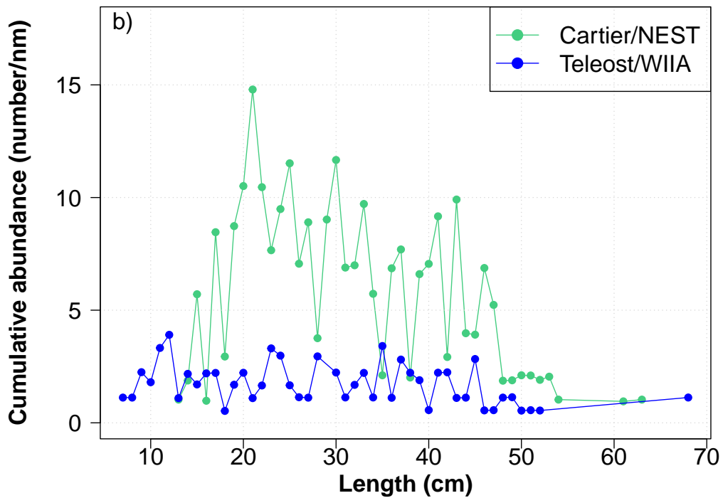
Figure 229. Biplot of Cartier catch versus Teleost catch (upper panel a), and cumulative length frequency distributions (lower panel b) for Laval's eelpout (species code 620, Lycodes lavalaei ).
