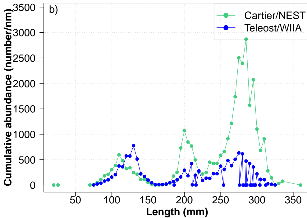
Figure 202. Biplot of Cartier catch versus Teleost catch (upper panel a), and cumulative length frequency distributions (lower panel b) for Atlantic herring (species code 60, Clupea harengus ).
