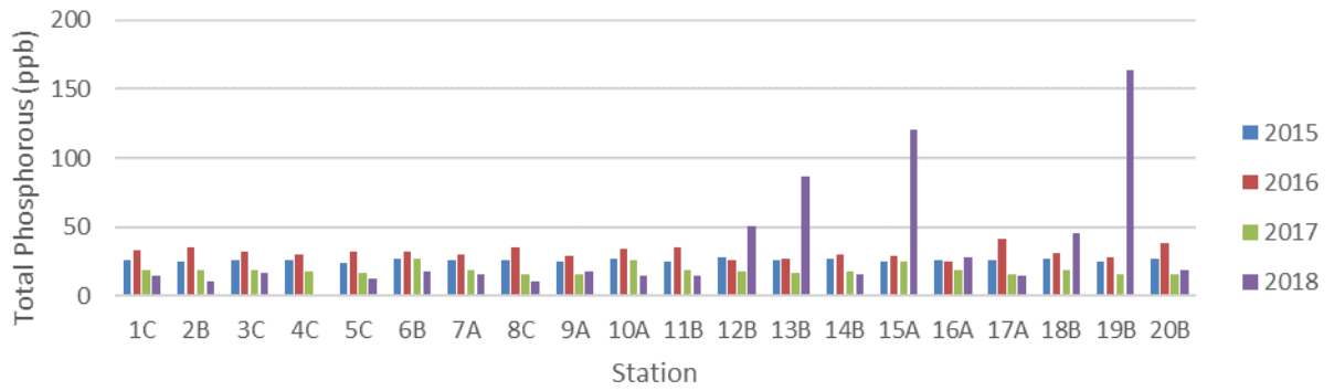
Figure 28. Annual total phosphorous by sampling station from ECW water quality monitoring 2015 to 2018.
