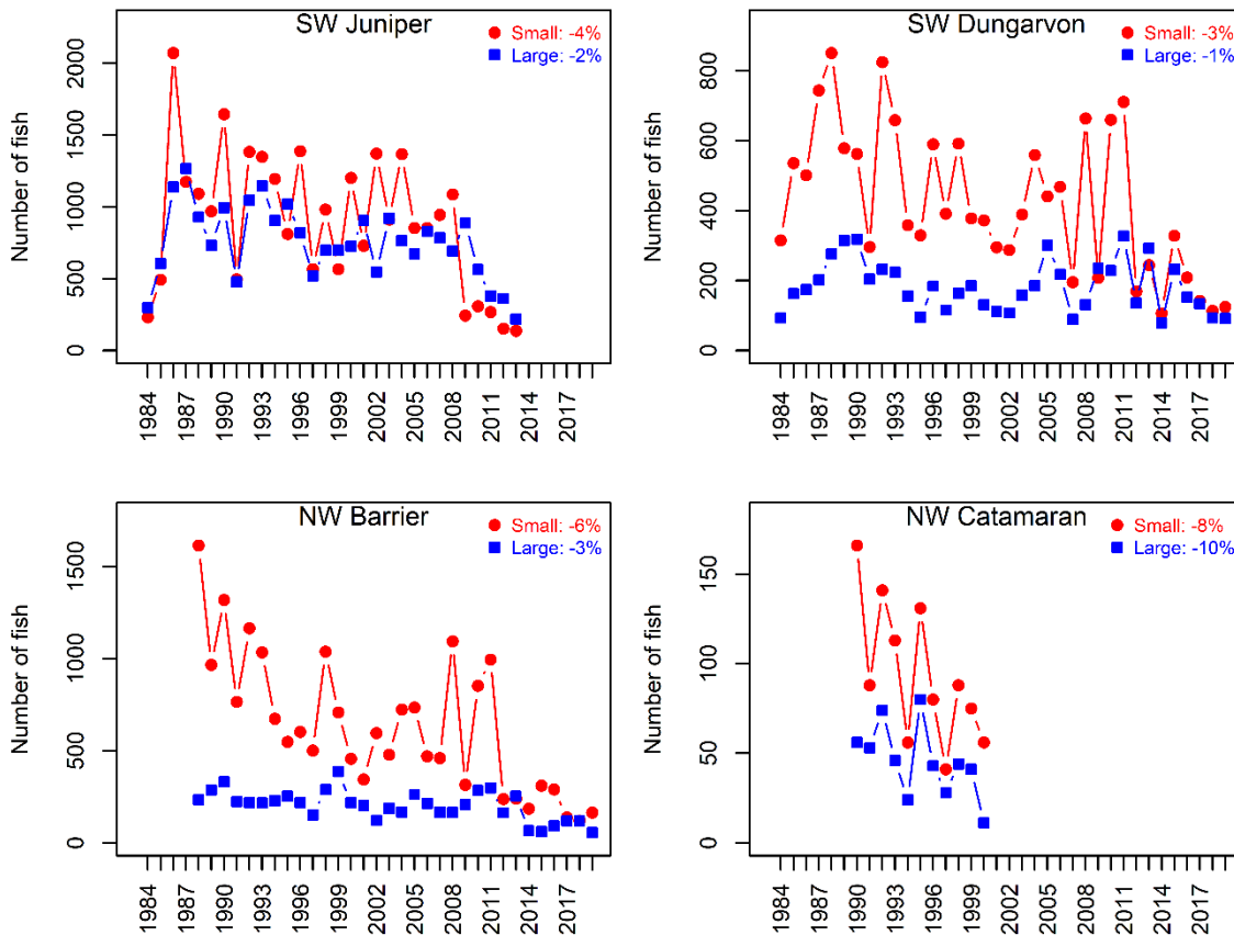
Figure 9. Indices of abundance (counts) of small Salmon and large Salmon at headwater monitoring facilities in the Miramichi River, 1984 to 2019. The annual percent change (exponential trend) over the available time series is shown in the upper right corner of each panel.
