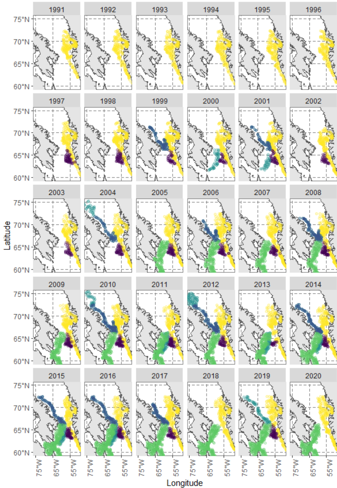
Figure 2. Survey coverage by year from 1991 to 2020, including DFO 0A-South (dark blue), 0A-North and 0B (light blue), NSRF-DFO shrimp (green; overlaps with the 0B survey), GINR 1C-D (purple) and 1A-F (yellow).
