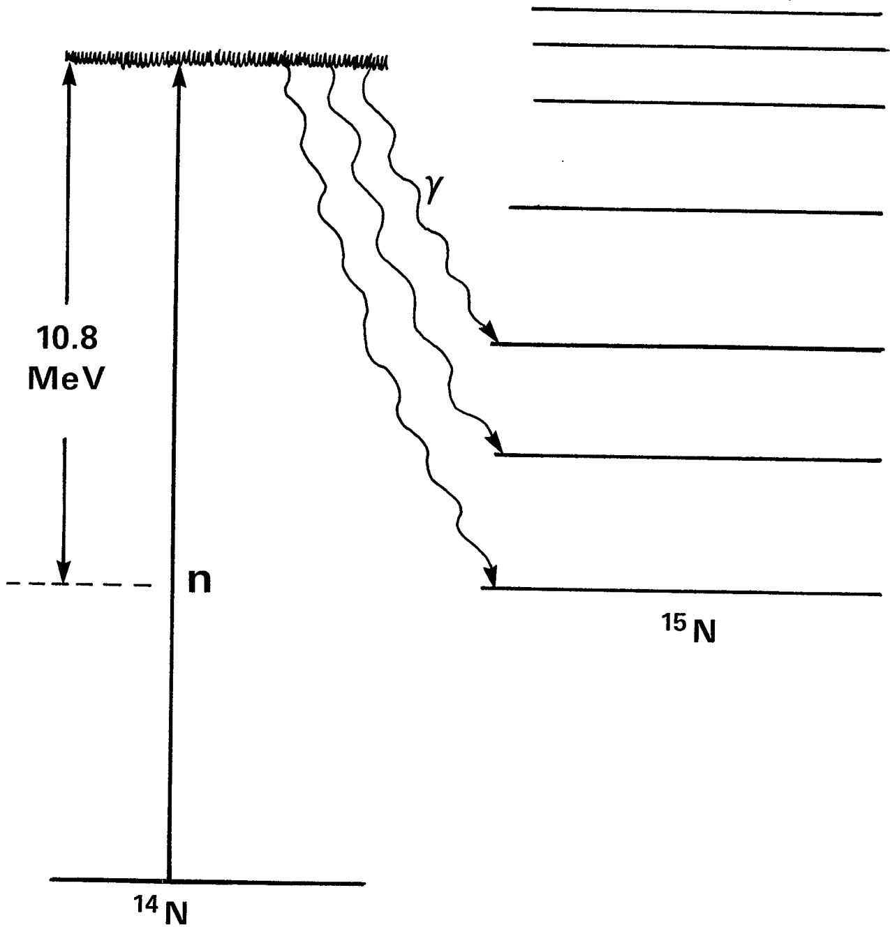
Figure 21 SCHEMATIC DIAGRAM OF THE ^{14}\text{N}(n,\gamma)^{15}\text{N} REACTION.
