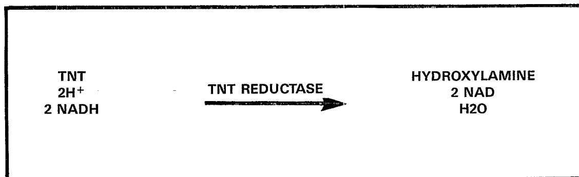
TNT DETECTION REACTION
