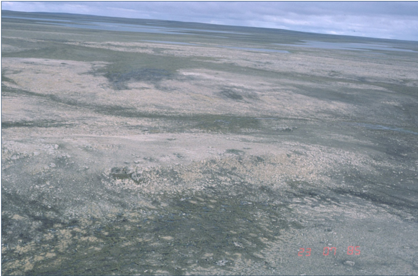
Figure 3. Typical eastern Victoria Island till plain with a bouldery surface. The till is thin, <2 m, and some bedrock is exposed. The surface is marked by common small polygons, which occur when sufficient matrix sediment is present; mid-distant scene is \sim 1 km across. Photograph by D.R. Sharpe. NRCan photo 2018-313
