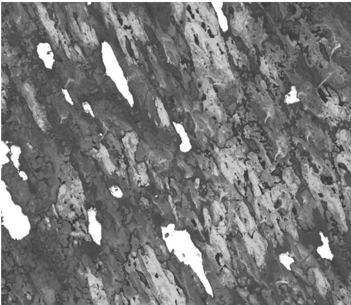
Figure 4a. Streamlined landforms oriented northwest occur in thin sediment and/or in bedrock ridges. Note sediment reworking in shoreline tails (small white ridges). Flow from southeast to northwest. SPOT panchromatic image ~4 km by 4 km.
