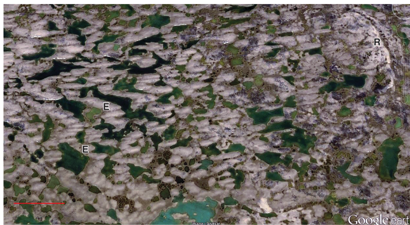
Figure 5. A drumlin field with complex forms converges westward, west of Albert Edward Bay; streamlined uplands show eroded exposed rock (R) on the upflow side (east) and sediment ridges further downflow (west). The drumlin forms appear as waveform aggregates of en échelon forms (E). Google Earth image; red scale bar is ~1 km.
