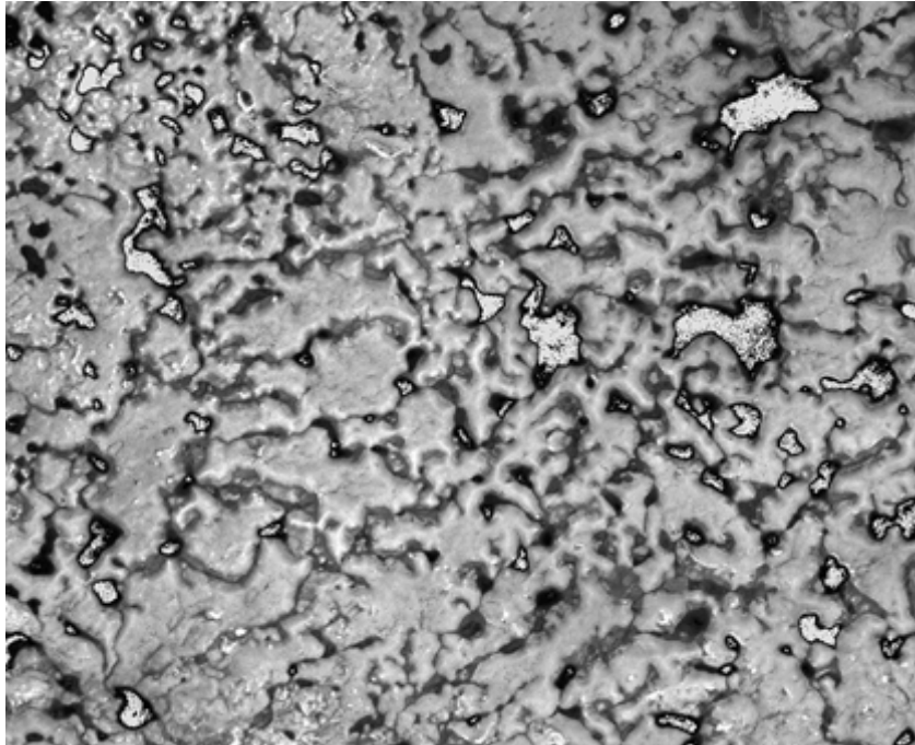
Figure 6. Classic hummocky terrain with distinct irregular ridge and plateau features; light-toned ridge edges are bordered by dark depressions. Plateaus have flat surfaces and ridges at the edges. Ice-wedge polygons are apparent as speckled patterns at ~ 1:20 000 scale.
