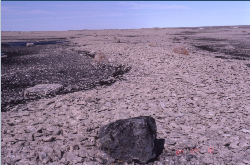
Figure 7b. Ground image of raised gravelly shoreline ridge composed mainly of flaggy carbonate clasts on bedrock. Photograph by D.R. Sharpe. NRCan photo 2018-314
