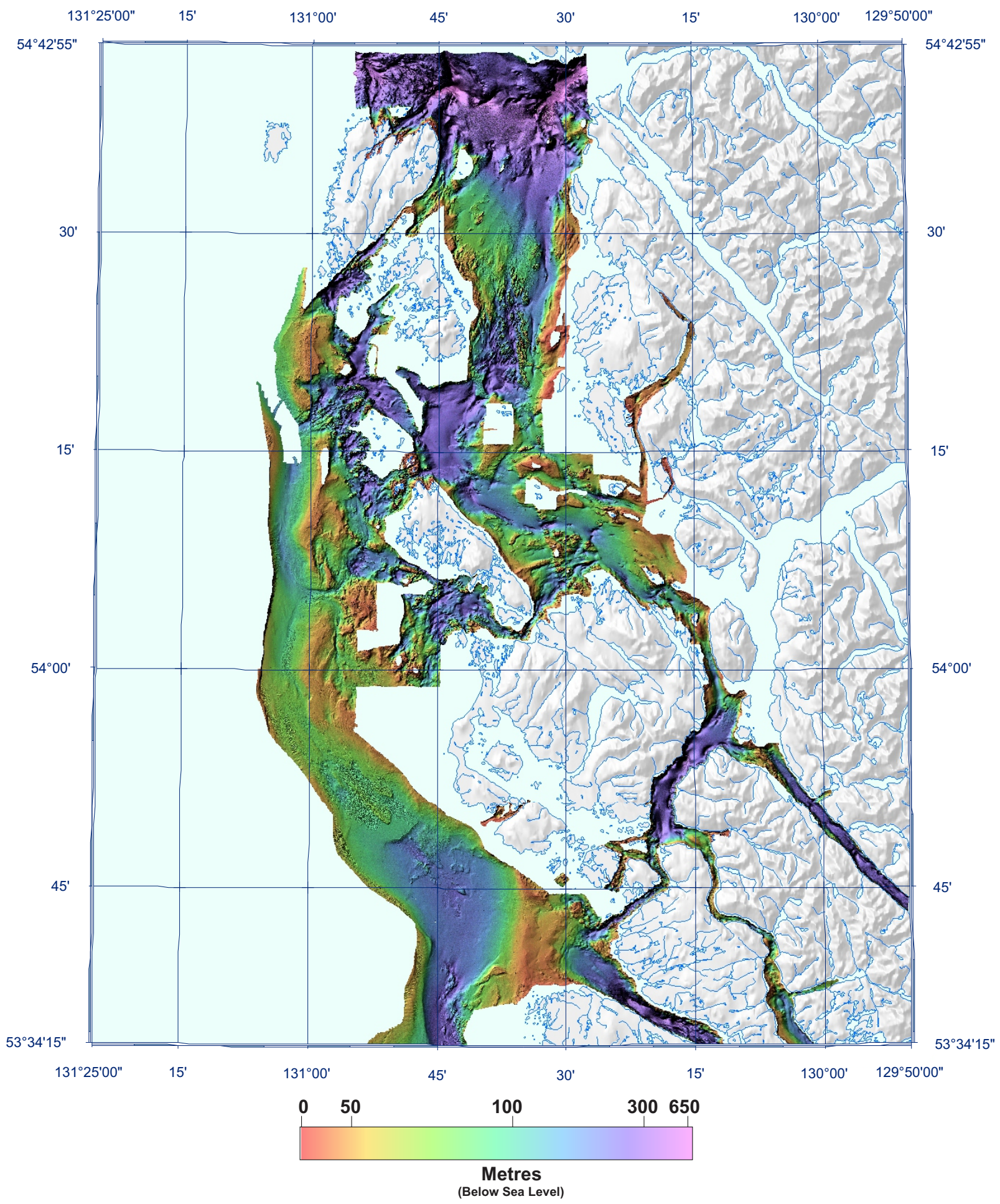
Figure 3. Multibeam bathymetry, Chatham Sound region, north coastal British Columbia.
