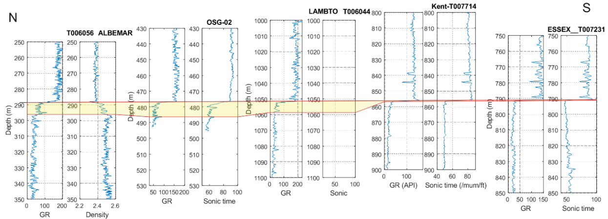
Figure 5: Cross-section showing the picked tops and bases of the Collingwood Member across the study area. See Fig. 4a for location of the cross-section.
