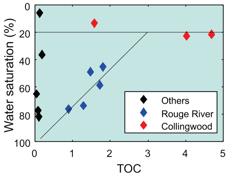
Figure 16: Cross plot of TOC content with water saturation showing relationship between organic content and water saturation in the same rock groups as shown of Fig. 15. “Others” indicate non-source rock quality samples.
