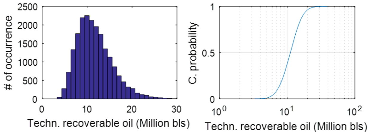
Figure 25: Probabilistic distribution of recoverable oil resource in the targeted Upper Ordovician shale units: Histogram (left) and cumulative distribution (right).
