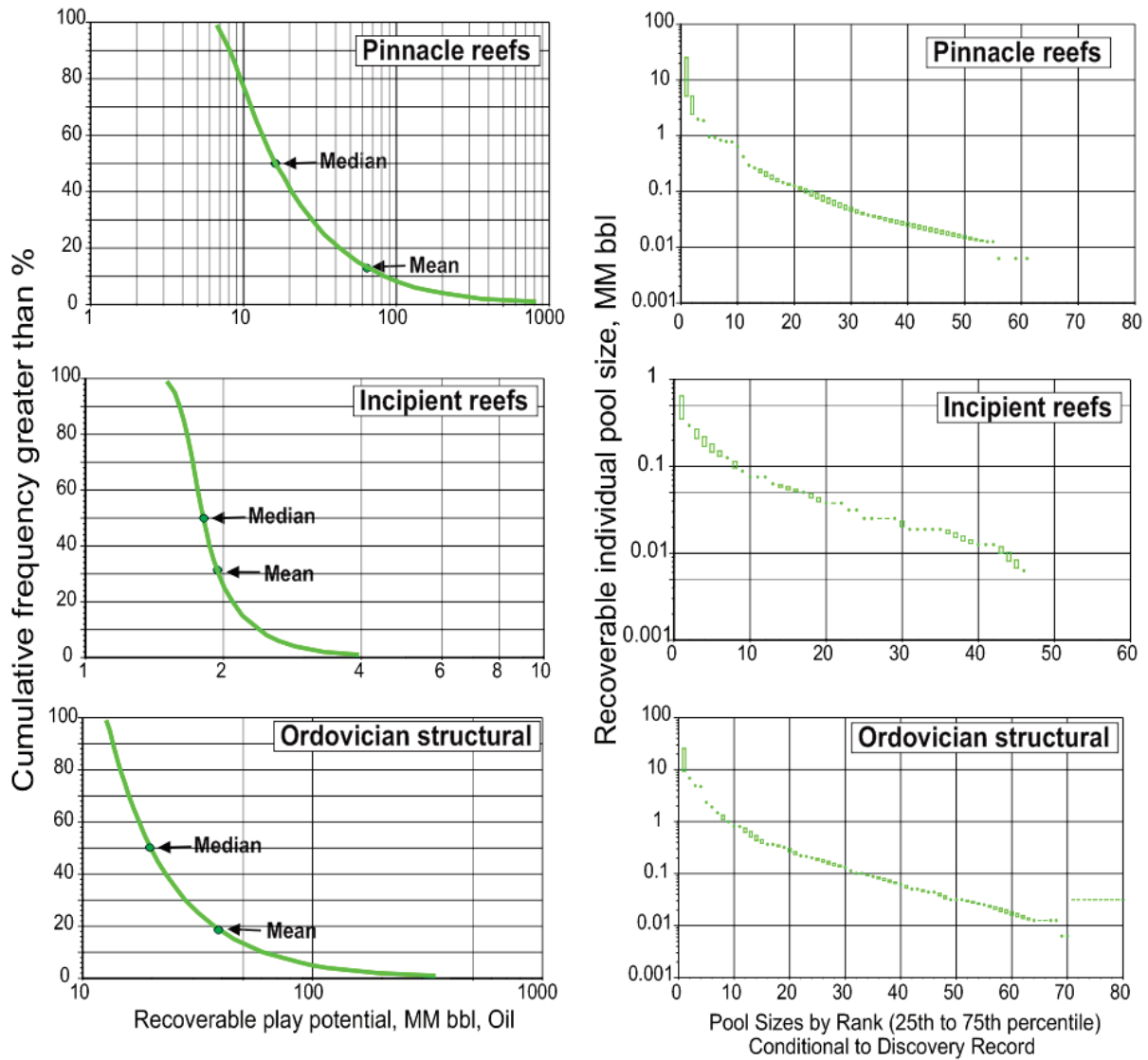
Figure 29: Estimates of recoverable remaining oil potential and pool-size by rank plots of conventional oil plays that partially occur in the NWMO study area.
