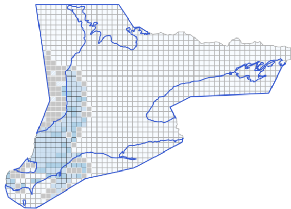
B Salt
