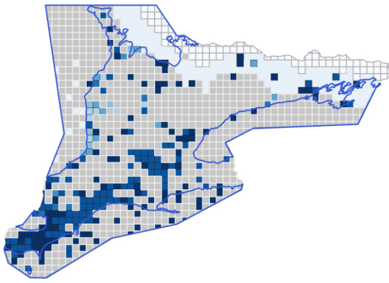
Sherman Fall
