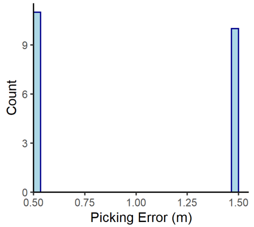
Neahga n= 21
