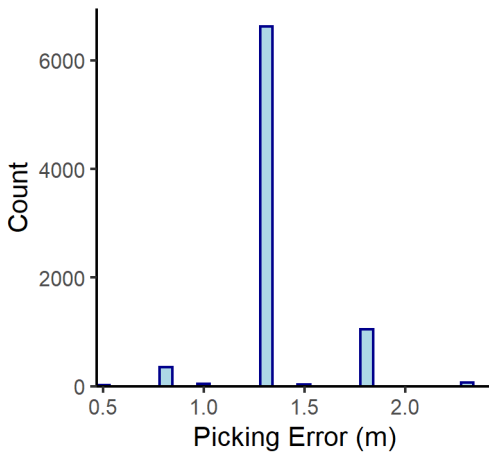
Whirlpool n= 8177
