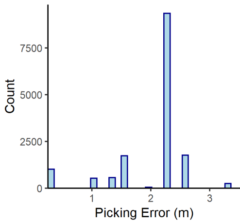
Guelph n= 15217
