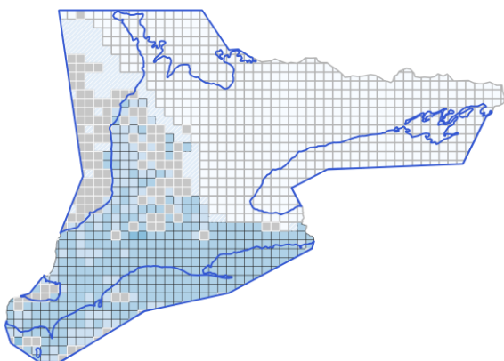
C Unit
