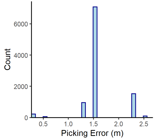
Queenston n= 9946
