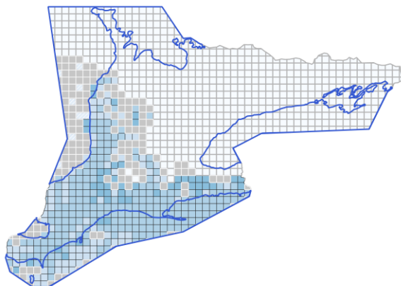
B Unit
