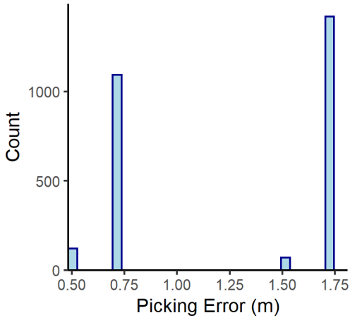
Thorold n= 2705
