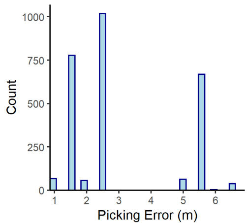
Manitoulin n= 2691
