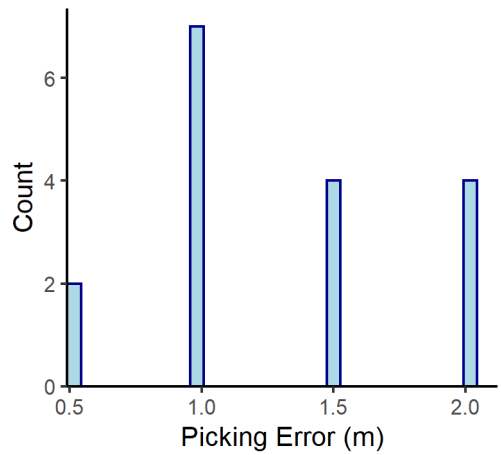
Wingfield n= 17
