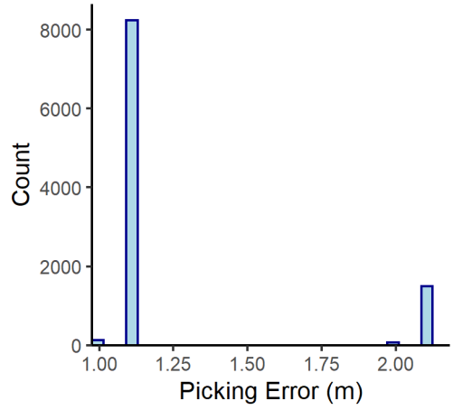
Grimsby n= 9923
