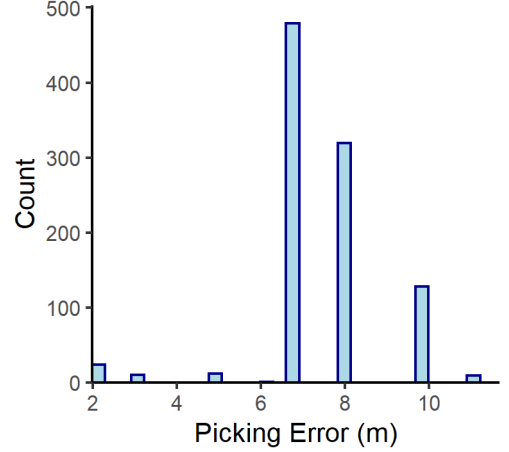
Kirkfield n= 982
