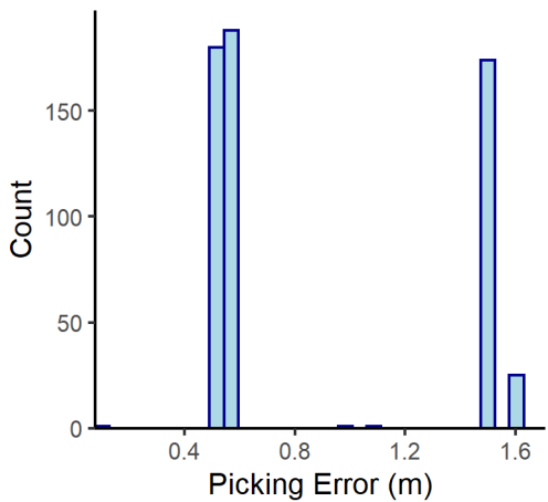
Oriskany n= 570
