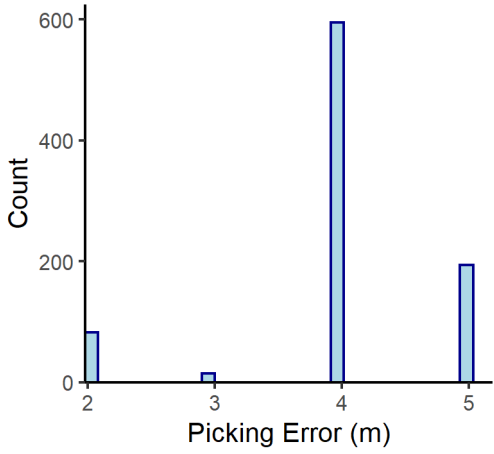
Precambrian n= 885
