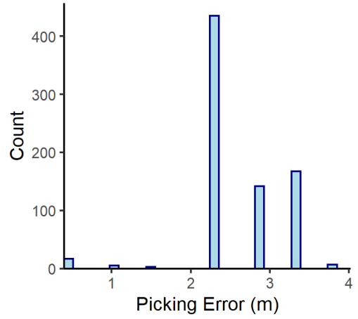
Cambrian n= 776
