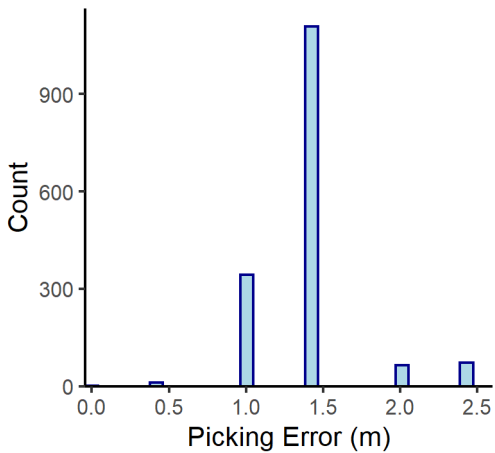
Columbus n= 1603
