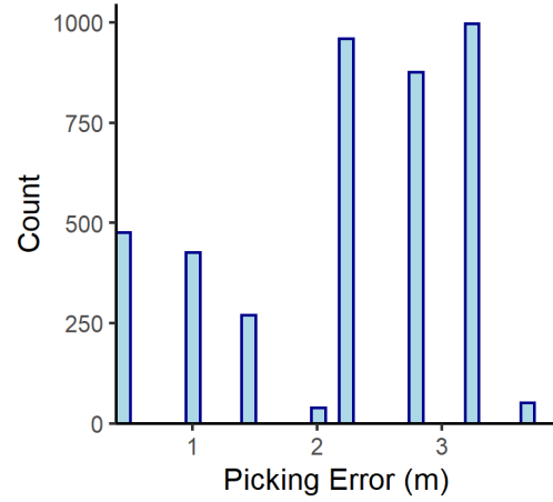
Gasport n= 4089
