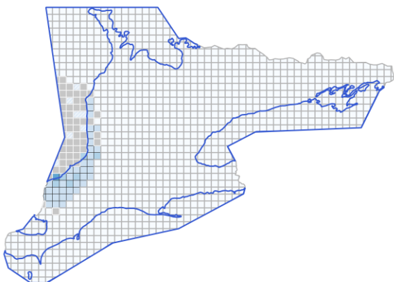
D Salt
