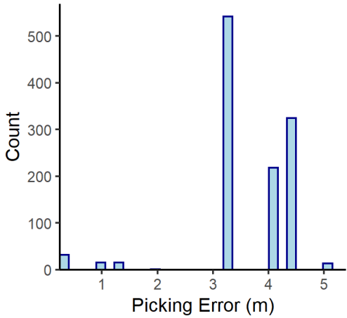
Coboconk n= 1161
