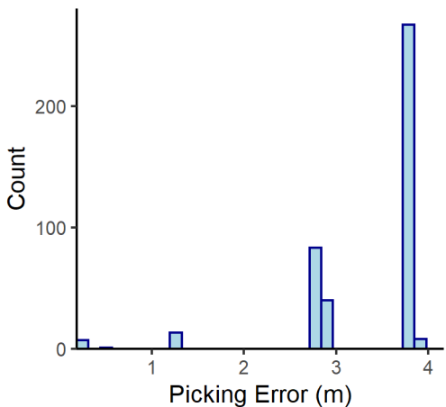
Marcellus n= 419
