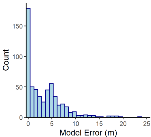
Oriskany n= 570
