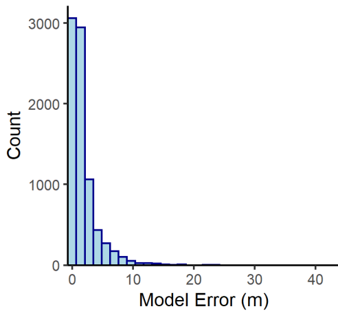
Whirlpool n= 8213
