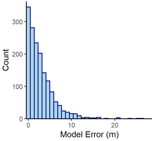
Columbus n= 1603
