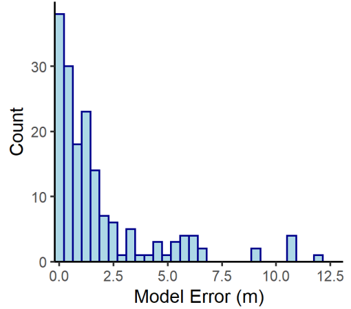
Port Lambton Group n= 168
