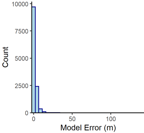
Georgian Bay – Blue Mountain n= 12609
