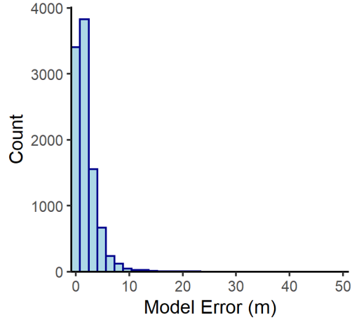
Grimsby n= 9940
