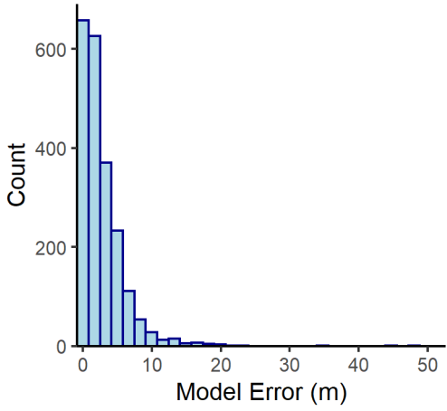
D Unit n= 2133
