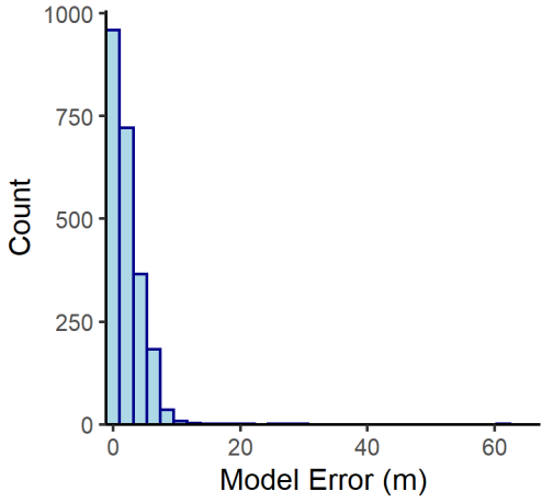
Precambrian n= 2283
