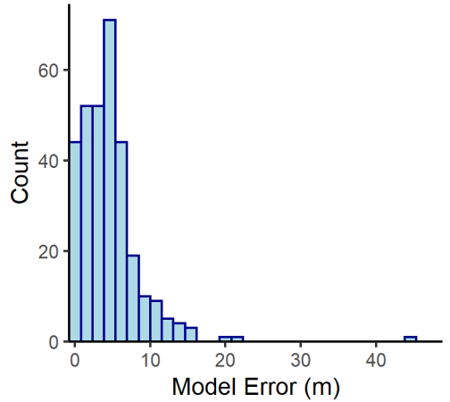
D Salt n= 316
