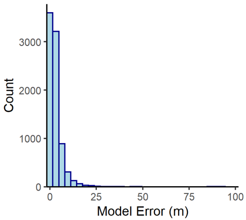
G Unit n= 8293
