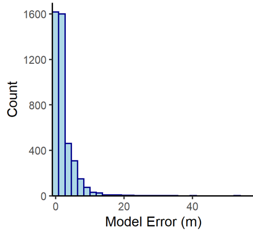
Gasport n= 4316
