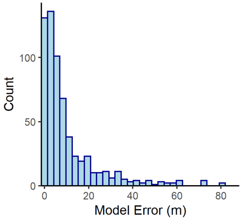
F Salt n= 623
