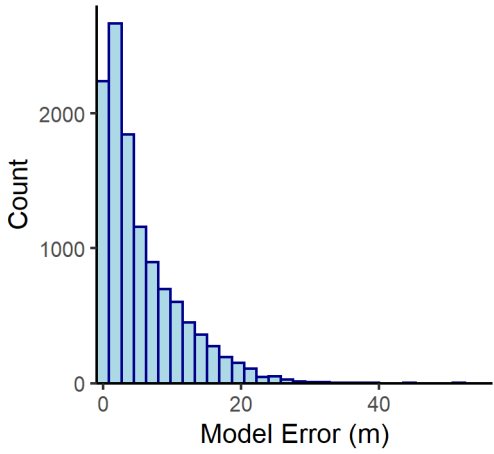
DeCew Rochester (Lions Head) n= 11805
