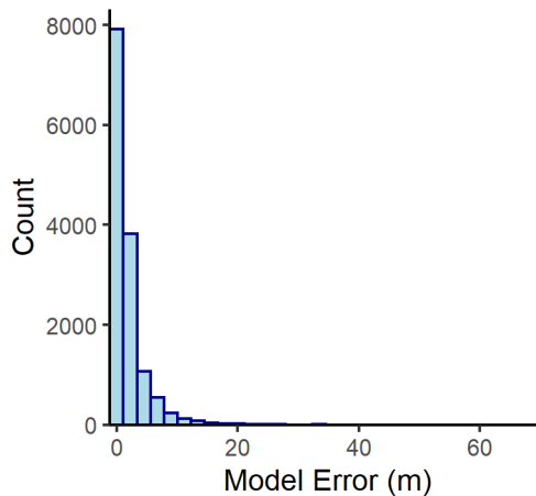
Lucas n= 13910
