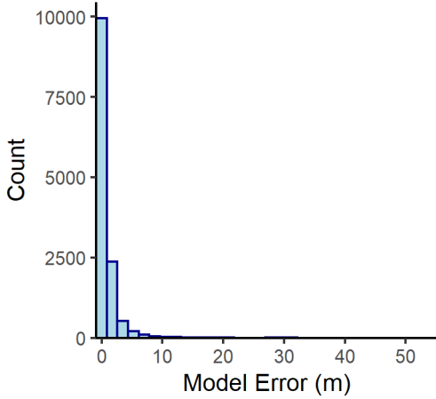
Kettle Point n= 13335
