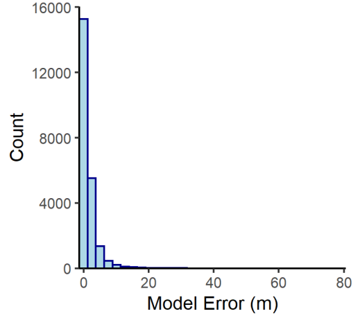
Dundee n= 23152
