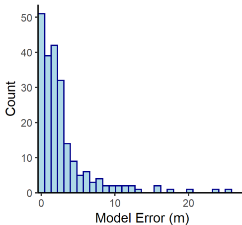
Sylvania n= 222
