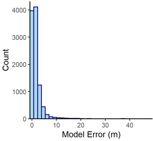
Cabot Head n= 10155
