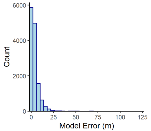
Bass Islands/Bertie n= 13560
