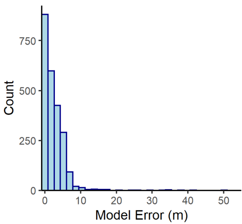
Coboconk n= 2349
