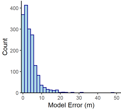
B Equivalent n= 1693
