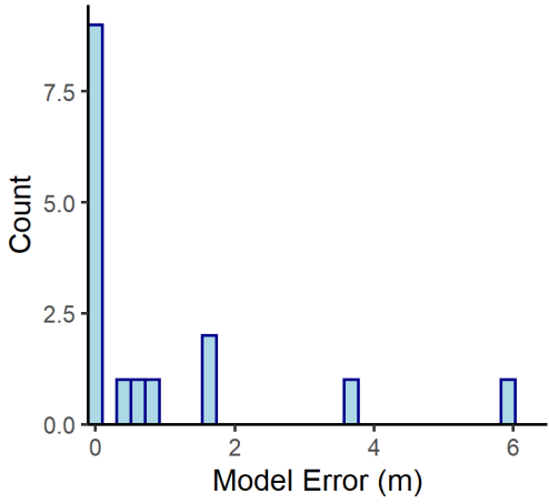
St. Edmund n= 16
