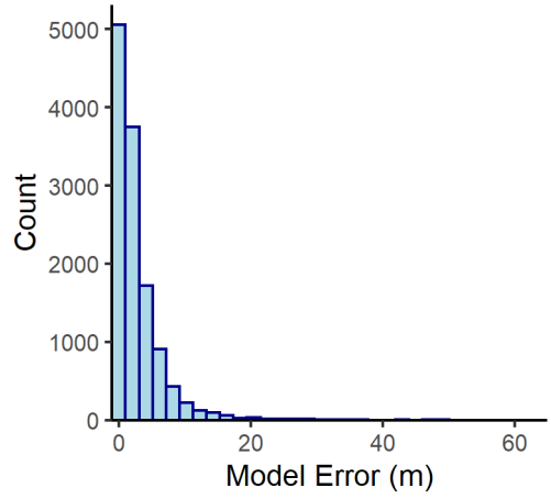
E Unit n= 12502
