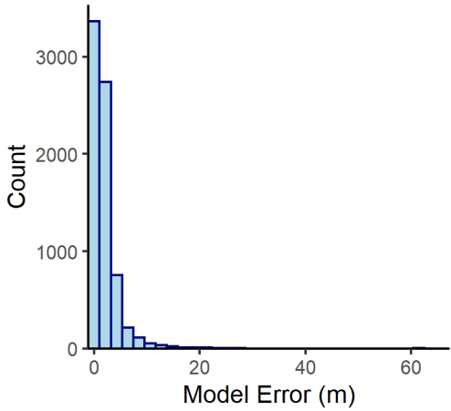
Goat Island n= 7355
