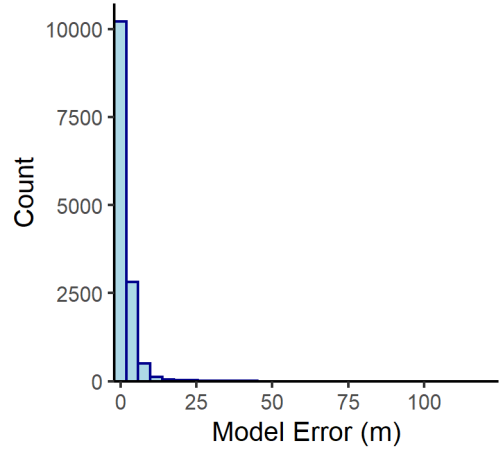
Hamilton Group n= 13818
