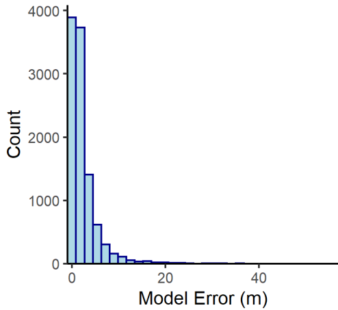
C Unit n= 10427
