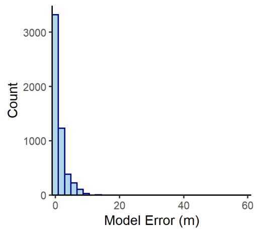
Kirkfield n= 5303
