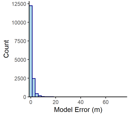
Cobourg n= 15344
