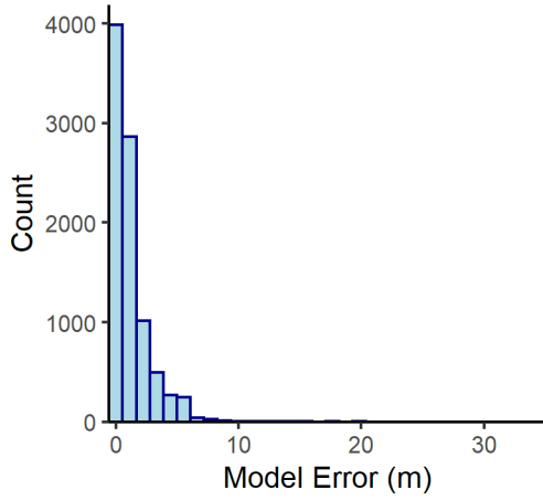
Sherman Fall n= 8975
