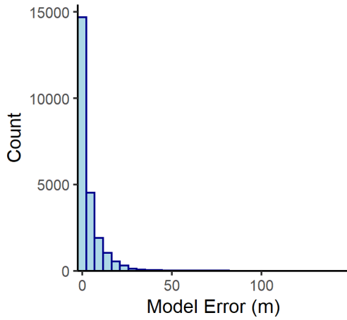
Guelph n= 23409
