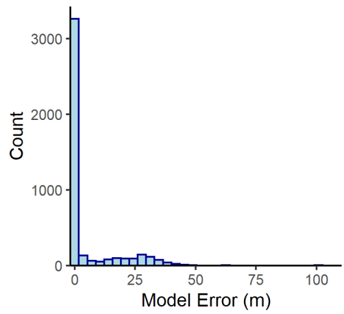
Gull River n= 4270
