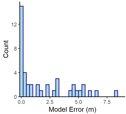
Wingfield n= 42
