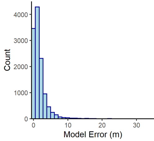
Irondequoit – Rockway- Fossil Hill n= 12075
