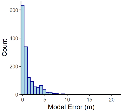
Marcellus n= 1442
