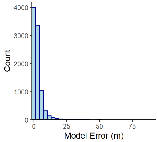
F Unit n= 9066
