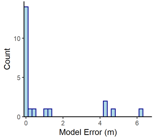
Neahga n= 22
