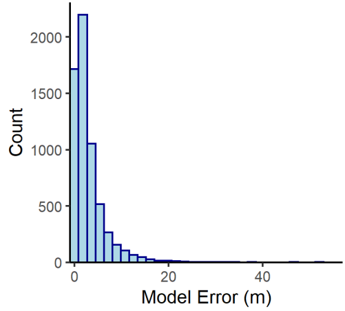
B Unit n= 6204
