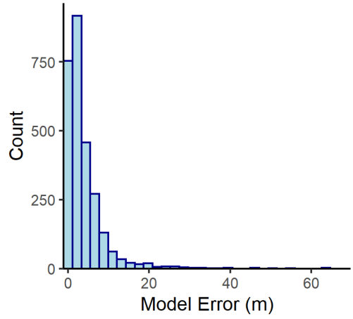
B Salt n= 2721
