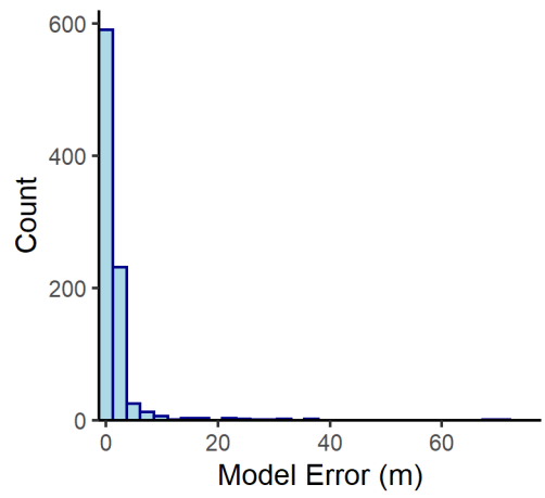
Cambrian n= 884
