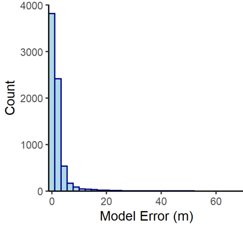
A-1 Carbonate n= 7254
