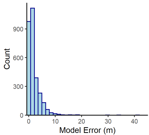
Manitoulin n= 2969
