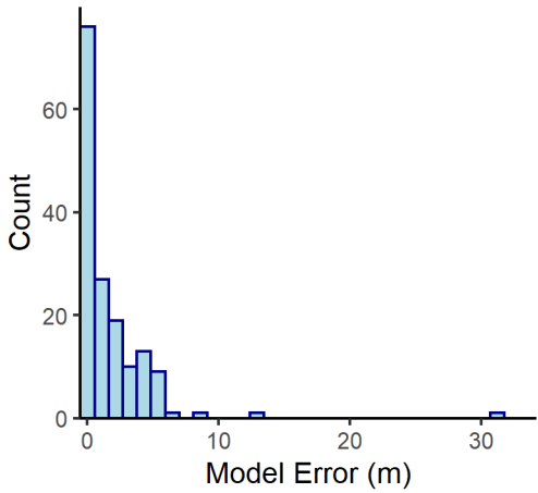
Dyer Bay n= 158
