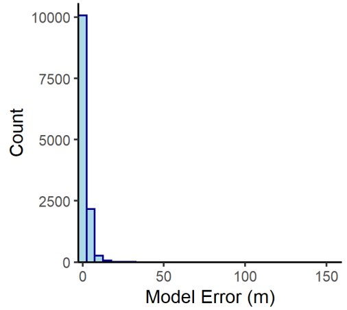
Queenston n= 12610
