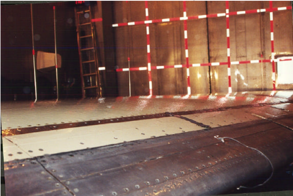
Photo 2.13 Thermistor Probe on Wing
