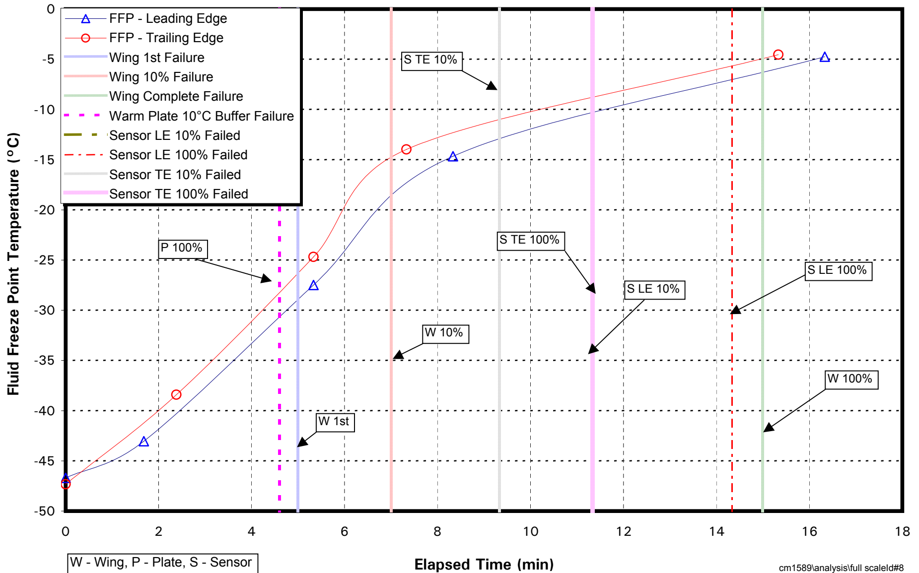
FIGURE E-8 Fluid Freeze Point Temperature Profile UCAR XL54, OAT = -6.9°C, 14.0 g/dm 2 /h January 26, 2000 - ID # 8
