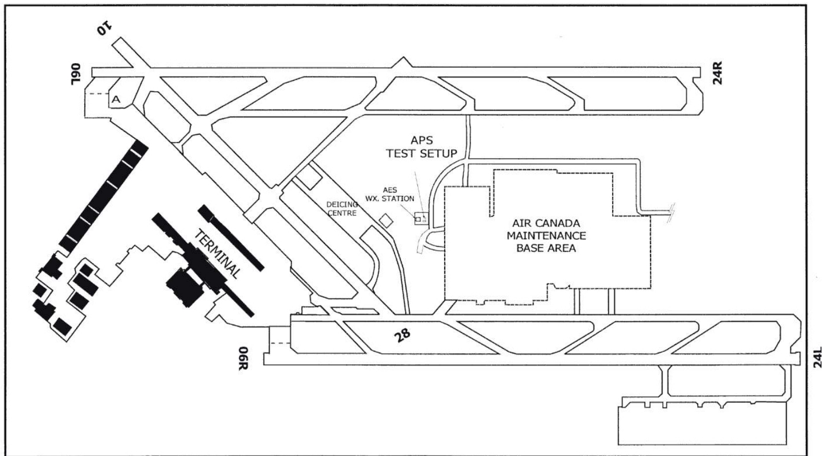
FIGURE 2.1 DEICING PAD LOCATION AT DORVAL AIRPORT
